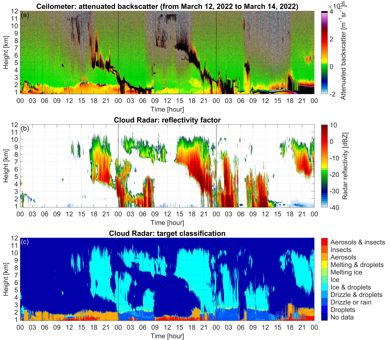
Figure 1. (a) Attenuated backscatter measured by a CHM15k ceilometer, (b) reflectivity measured by a RPG-FMCW Doppler cloud radar, and (c) the radar target classification in Granada, March 12-14, 2022. Height is above sea level.
