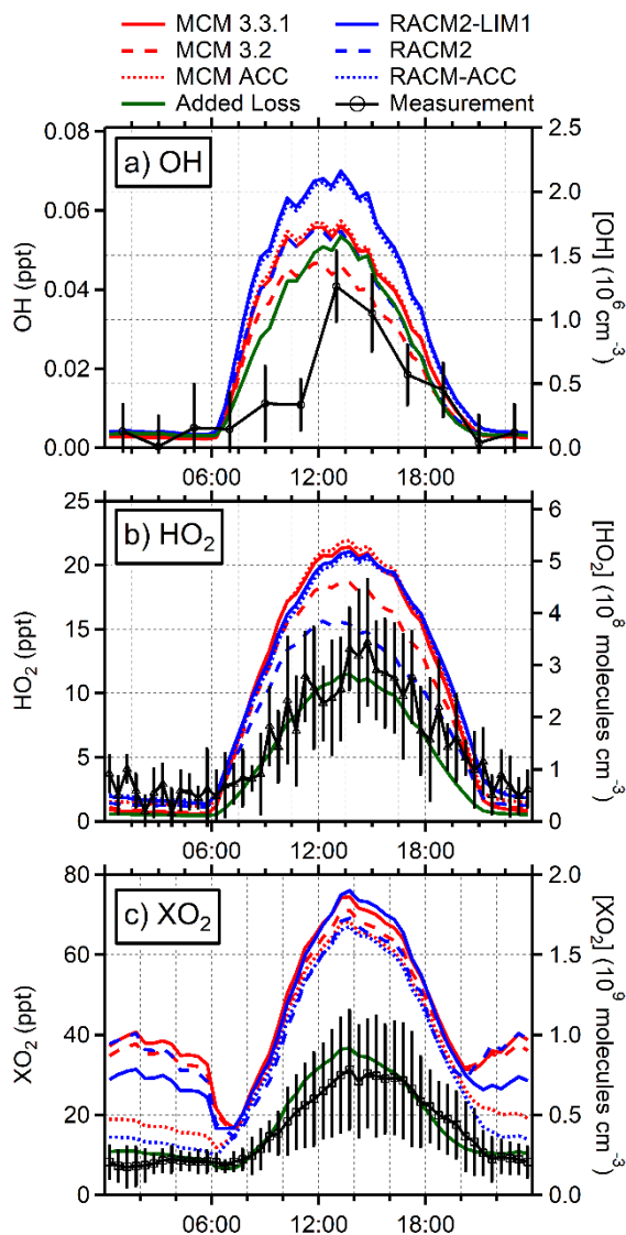
Figure 4: Diurnal average measured (black) and modeled concentrations of (a) OH, (b) HO 2 , and (c) XO 2 . MCM models are shown in red and RACM 2 in blue. The green line represents an additional version of the RACM-ACC model with added sinks for HO 2 and isoprene peroxy radicals. The colored lines represent an average of individual daily model runs from only the days that each respective species was measured (OH: 7/3–7/9, 7/11–7/14, and 7/16–7/25; HO 2 : 7/3–7/9 and 7/11–7/31; XO 2 : 7/9–7/14 and 7/18–7/26). Error bars represent the 1 \sigma measurement precision.
