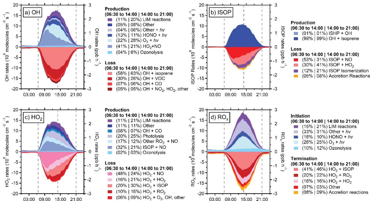
550 Figure 6: Radical budgets from the RACM2-LIM1 model with additional accretion reactions (RACM-ACC) for a) OH, b) isoprene- based peroxy radicals (ISOP), c) HO 2 , and d) total RO x . Shades of blue represent reactions that produce/initiate radicals, and shades of red represent radical loss/termination reactions. LIM reactions (purple) include reactions added as part of the Leuven Isoprene Mechanism. Percentages represent the relative initiation or termination rates of each respective process in the morning (06:30: to 14:00) and during the evening (14:00 to 21:00) which are indicated by the vertical dashed lines.
