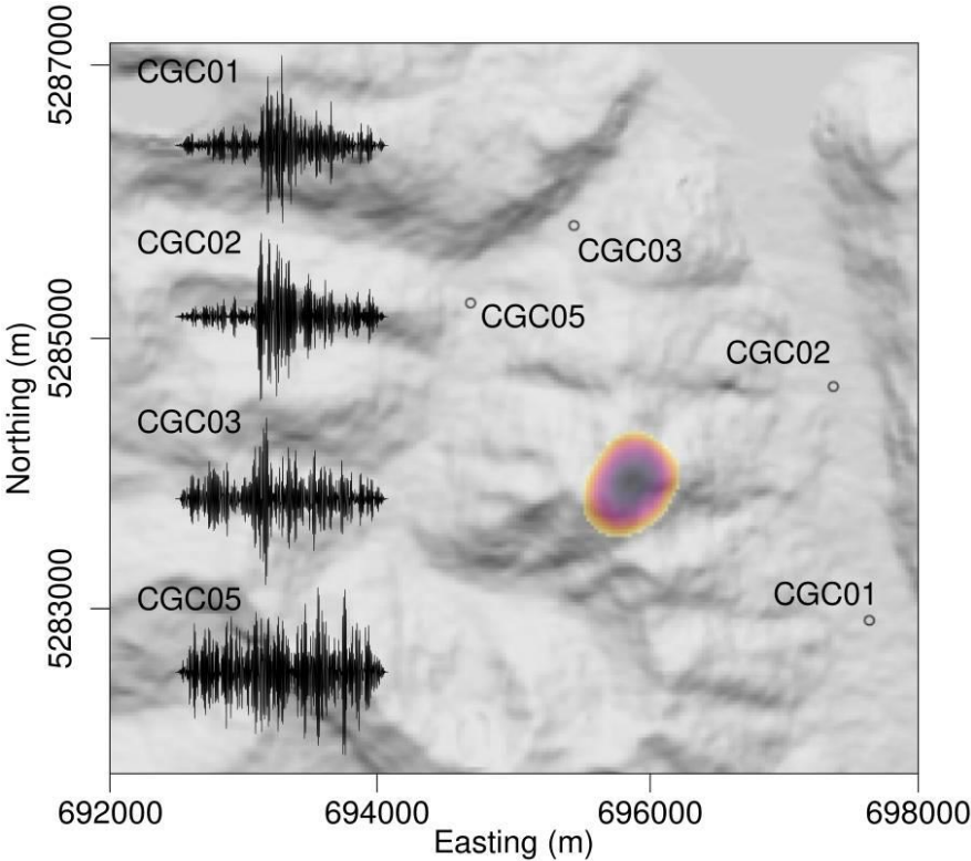
Figure 6. Seismically detected and located hillslope event happening at 2022-03-22 03:59:18. Hillshade map in background shows Caleta Gonzalo catchment and location of the four ground stations used to located the event. Coloured polygon shows the > 99 % confidence area of event location. Seismograms (10–15 Hz bandpass filtered deconvolved waveforms) of 14 s length, with the 7 s lasting event as registered by the four stations. Note that CGC05 close to the waterfall is dominated by the river turbulence signal, in which the mass wasting signature drowns.
