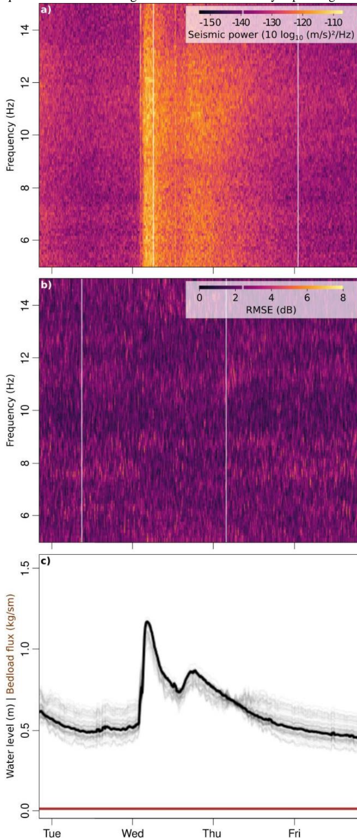
Figure 7. Inversion of seismic power spectra for river dynamics. a) Seismic spectrogram zoomed to analysed frequency range 5–15 Hz with clear broad band power maximum on Wednesday, 23 March 2022. b) Root mean square error matrix of modelled and measured spectra. c) Monte Carlo-based hydrographs (grey lines) and bedload flux time series (brown lines) for n=500 simulations and 5 sample window size. Thick black and brown line depict average results of the former two metrics. Based on UAV imagery, we set river bed particles to range around a D_{50} of 0.2 \pm 0.5 ( \sigma ) and channel gradient to 0.05. Consistent with mostly loose cobble and organic rich material building the river terrace and foot slopes between river and seismometer, we set the Rayleigh wave velocity to 500 m/s, ground quality factor to 23, and the Greens function displacement amplitude parameters between 0.6 and 0.8.
