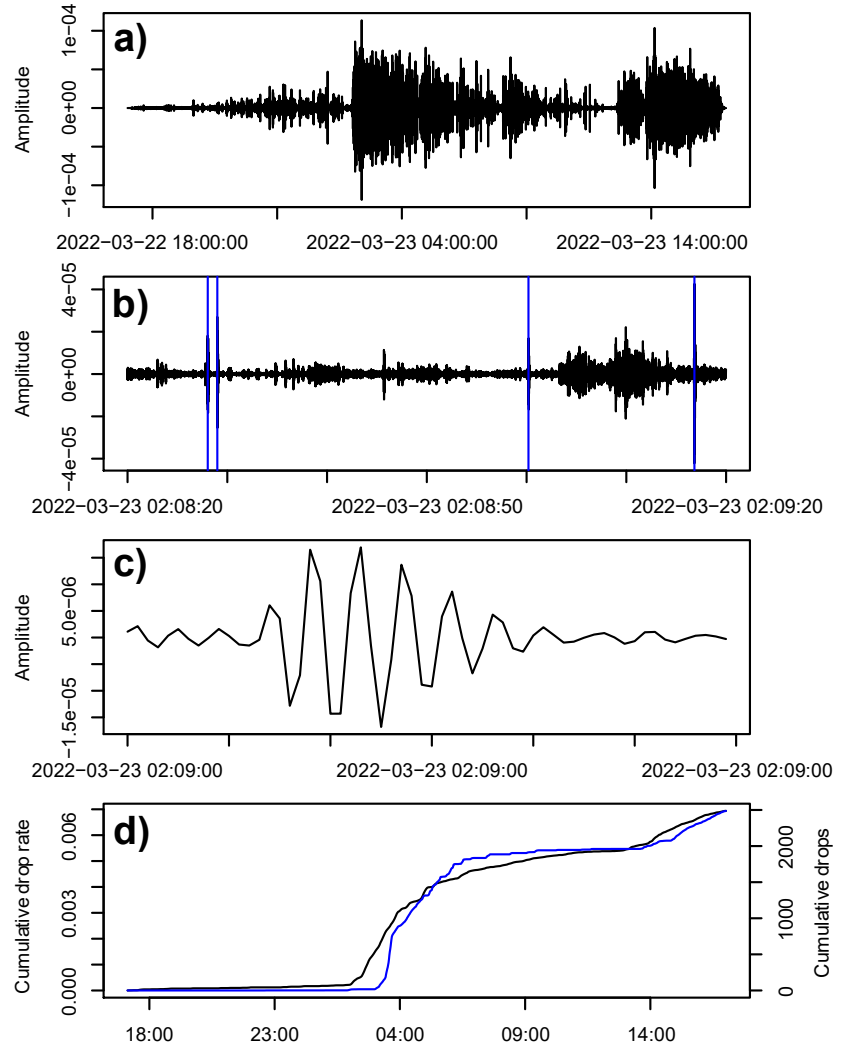
Figure 5. Rain information from seismic sensors. a) 50–60 Hz filtered seismic waveform of station CGC04 during period shown in Figure 9. b) Zoom to one-minute interval with STA-LTA-picked potential rain drop impacts (blue vertical lines) considering short and long term windows of 0.5 s and 300 s, respectively, on-ratio of 3 and off-ratio of 1.1. c) Zoom to a single 0.3 s long interval with a 0.15 s long drop impact signal. d) Cumulative seismic (black line) and weather station derived (blue line) precipitation record.
