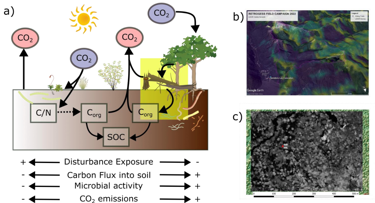
Figure 3. Simplified carbon cycle @Pumalin CZO. a) Ignoring CH 4 , the main route of carbon into soil is via autotrophic C-fixation by pioneer microbial communities on recent landslide scars, diagnostic C/N ratios indicate a qualitative shift on older landslides where carbon fixation is mostly of photosynthetic origin by bacteria and mycorrhizae communities. Yellow box highlights windthrow-induced tree mortality (see also section ‘2.3.1 Tree Mortality by wind throw.’) linking above and below ground C-pools; b) Modeled wind exposure for Caleta Gonzalo Catchment following Buma and Johnson (2015) overlaying data from © Google Earth, and c) LiDAR-based tree identification using TREETOP algorithm (Silva et al., 2022)
