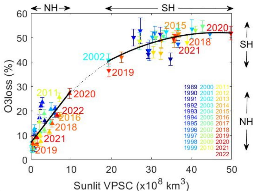
380 Figure 10. Ozone loss as a function of sunlit volume of polar stratospheric clouds (VPSC) for each winter for the Northern and Southern hemispheres. The 68% interpercentile of ozone losses are also represented (see Sect. 3, Methodology). The colour code represents the years. The linear and parabolic fits are represented for the NH and SH, respectively, (black lines) and the 3 rd -order fit considering years for both hemispheres is represented by the black dotted line.
