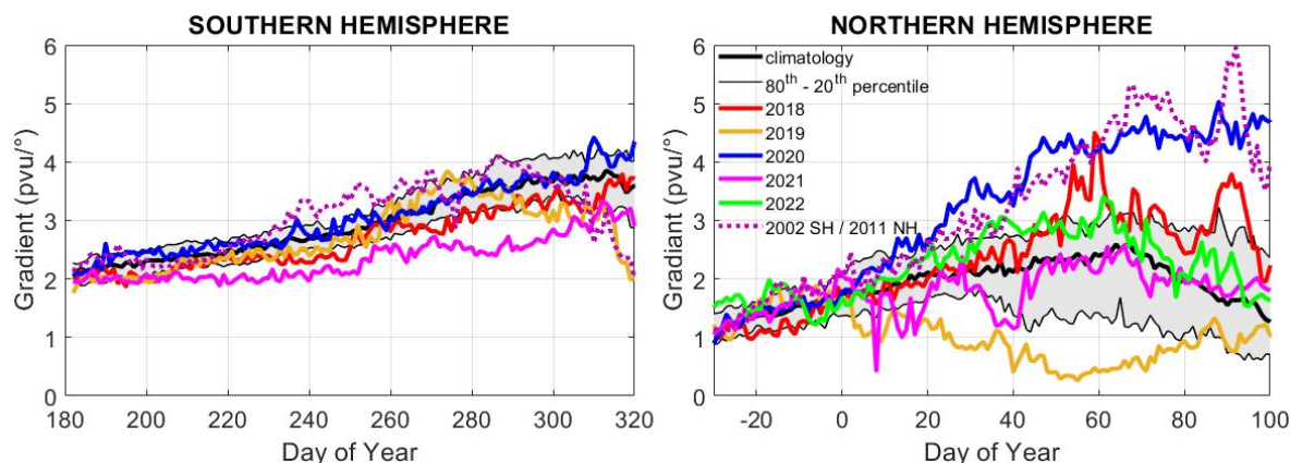
Figure 7. As Fig. 4 but for the PV gradient in the vortex edge as defined in Pazmiño et al. (2018) using ERA5 reanalyses.
