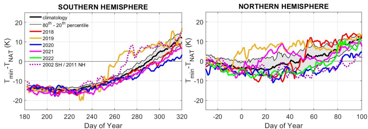
Figure 5. As Fig. 4 but for temperature anomaly at 475 K using ERA5 reanalyses.
