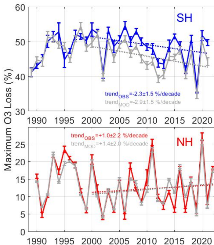
340 Figure 8. Interannual evolution of the maximum ozone loss obtained using the passive tracer method and the merged OBS dataset (colour lines) and model (gray line) in the SH (top panel) and NH (bottom panel). The estimated robust trends since 2000 were added to the figures with the corresponding colour codes.
