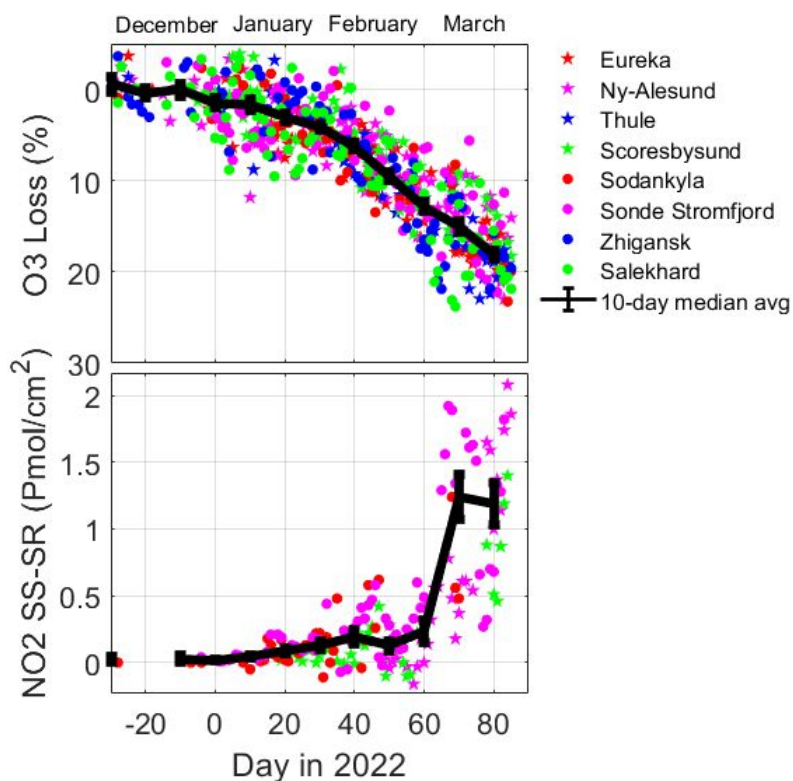
Figure 2. Top panel: time series of observed ozone loss (%) inside the vortex above each SAOZ station for the 2022 NH winter.
