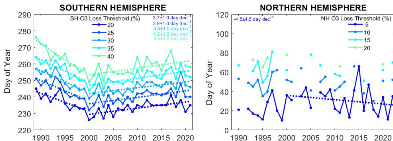
355 Figure 9. Onset day when 10-day averaged ozone loss reach a particular ozone loss value: 20, 25, 30, 35 and 40% for the SH (left panel) and 5, 10, 15 and 20% for NH (right panel). Robust linear fits before and after 2000 are also shown for the SH (dashed lines).
