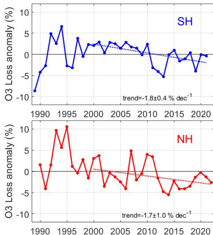
Figure 11. Interannual evolution of Residuals of Ozone Loss with respect to regressed ozone loss values computed following Eq. 1 for the SH (top panel) and NH (bottom panel). Estimated trends since 2000 are represented by dotted lines.
