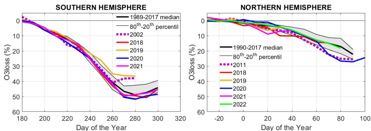
Figure 4. Evolution of ozone loss in recent winters using the merged OBS dataset: SH 2018-2021 (left panel) and NH 2018/19 – 2021/22 (right panel). Unusual winters are also represented by pink dashed lines: weak ozone loss in SH (2002) and 2011 record ozone loss in NH. The median and 20 th –80 th percentile climatological values of previous winters are represented by thick and thin black lines, respectively.
