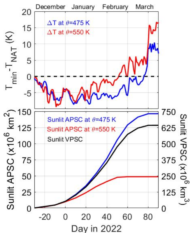
Figure 3. Top panel: time series of difference between minimum temperatures and T_{\text{NAT}} (K) at 475 and 550 K isentropic levels for the 2022 NH winter. Negative values correspond to the period of PSC formation at the corresponding isentropic level. Bottom panel: cumulative time series of sunlit areas of PSC at 475 (blue) and 550 K (red). The sunlit volume of VPSC computed following Rex et al. (2004) is superimposed by a black curve.
