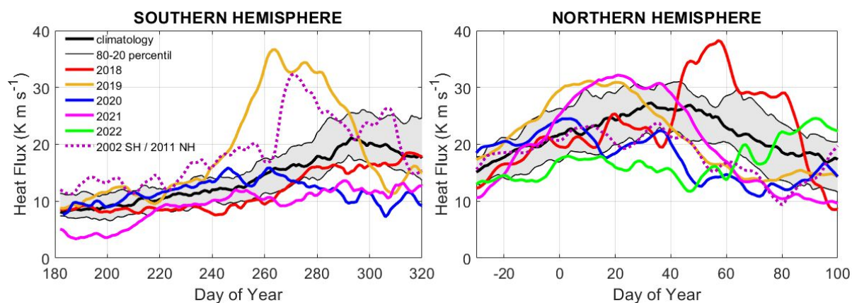
240 Figure 6. As Fig. 4 but for 45-day mean heat flux in the 45°–75° latitude range at 70 hPa from MERRA-2 analyses.
