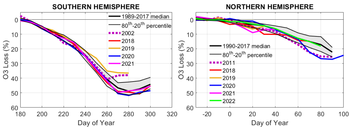
240 Figure 5. Evolution of ozone loss in recent winters using the merged OBS dataset: SH 2018-2021 (left panel) and NH 2018/19 – 2021/22 (right panel). Unusual winters are also represented by pink dashed lines: weak ozone loss in SH (2002) and 2011 record ozone loss in NH. The median and 20 th –80 th percentile climatological values of previous winters are represented by thick and thin black lines, respectively.
