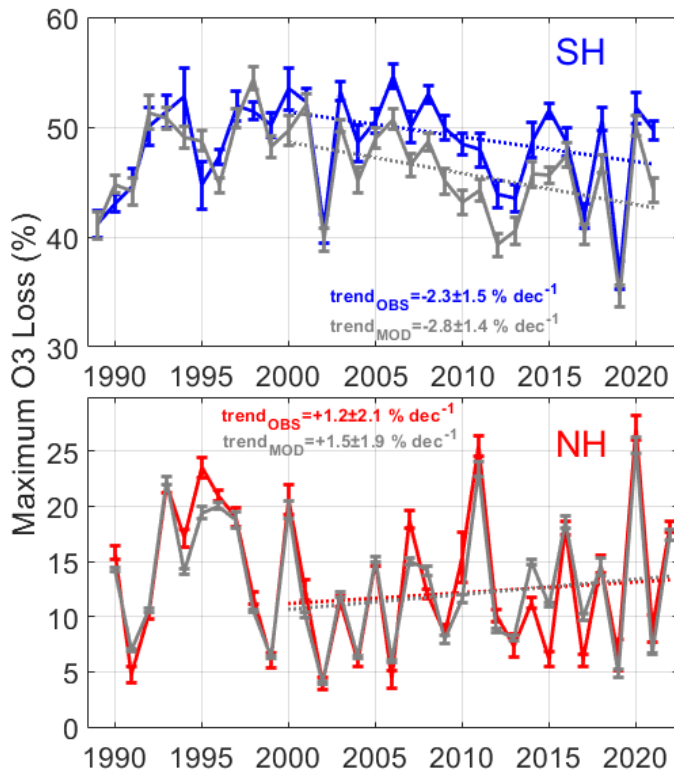
355 Figure 9. Interannual evolution of the maximum ozone loss obtained using the passive tracer method and the merged OBS dataset (colour lines) and model (gray line) in the SH (top panel) and NH (bottom panel). The estimated robust trends since 2000 were added to the figures with the corresponding colour codes.
