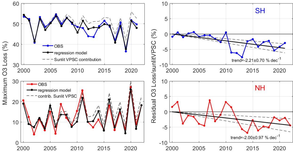
435 Figure 13. Left panels: Interannual evolution of the maximum ozone loss (colour lines) since 2000 for both hemispheres and regression model (black lines). Sunlit VPSC contribution (see Eq. 2 for NH and 3 for SH) is superimposed by dashed lines. Right panels: Interannual evolution of Residuals of Ozone Loss with respect to regressed ozone loss values computed following Eq. 1 to 4 for the SH (top panel) and NH (bottom panel). The estimated trend (thick black line) and uncertainty level values of \pm 1\sigma (dashed black lines) since 2000 are also represented for both hemispheres. 440
