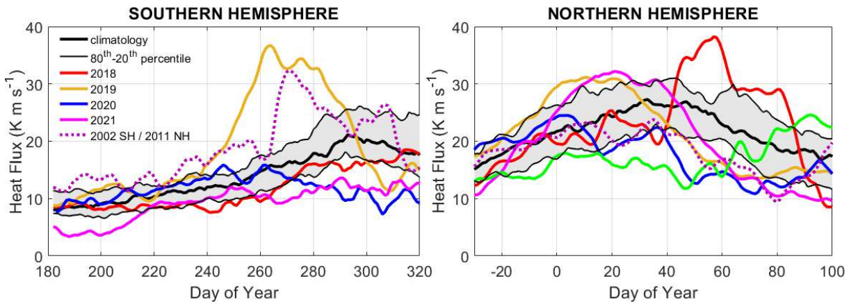
Figure 7. As Fig. 5 but for 45-day mean heat flux in the 45°–75° latitude range at 70 hPa from MERRA-2 analyses.
