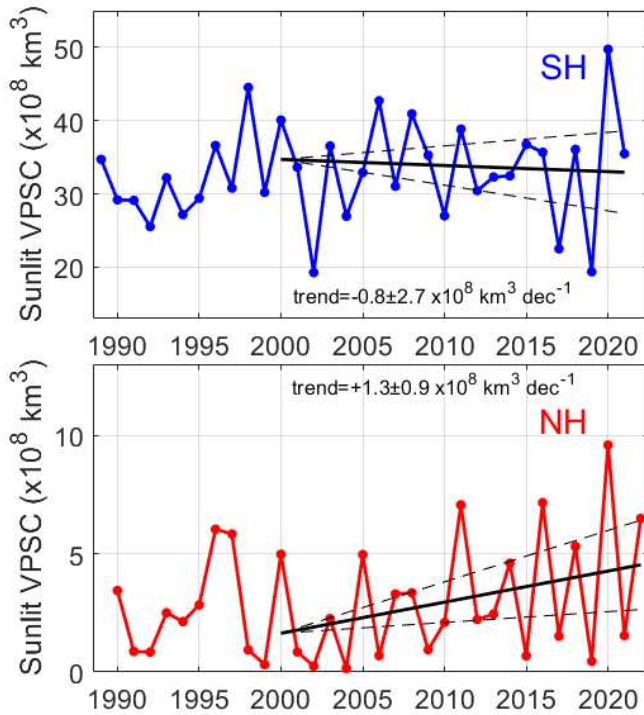
395 Figure 11. Interannual evolution of sunlit volume of polar stratospheric clouds (VPSC) in the SH (top panel) and NH (bottom panel). The estimated robust trend (thick black line) and uncertainty level values of \pm 1\sigma (dashed black lines) since 2000 are added for both regions.
