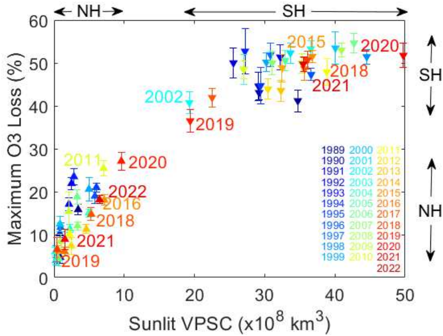
Figure 12. Maximum ozone loss as a function of sunlit VPSC for each winter for the Northern and Southern hemispheres. The 68% inter-percentile range of ozone losses are also represented (see Sect. 3, Methodology). The colour code represents the years.
