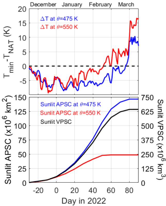
210 Figure 4. Top panel: time series of difference between minimum temperatures and T_{\text{NAT}} (K) at 475 and 550 K isentropic levels for the 2022 NH winter. Negative values correspond to the period of PSC formation at the corresponding isentropic level. Bottom panel: cumulative time series of sunlit areas of PSC at 475 (blue) and 550 K (red). The sunlit volume of VPSC computed following Rex et al. (2004) is superimposed by a black curve.
