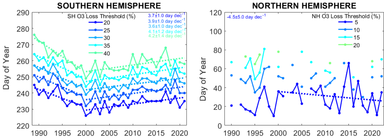
370 Figure 10. Onset day when 10-day averaged ozone loss reach a particular ozone loss value: 20, 25, 30, 35 and 40% for the SH (left panel) and 5, 10, 15 and 20% for NH (right panel). Robust linear fits before and after 2000 are also shown for the SH (dashed lines).
