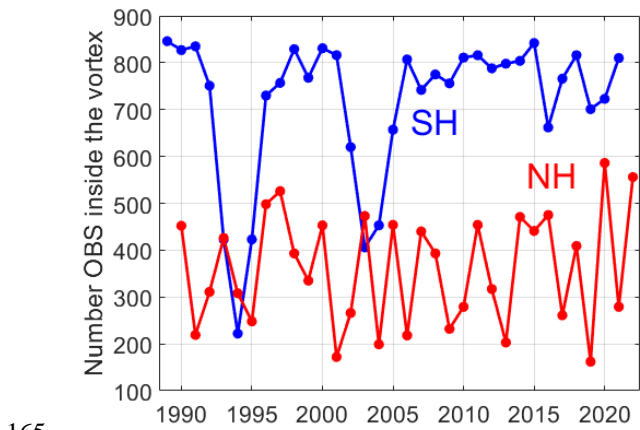
Figure 1. Number of merged data (OBS) inside the vortex for each winter of the SH (blue line) and NH (red line).
