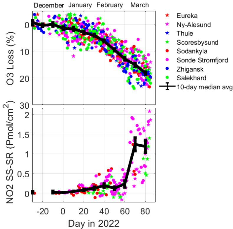
205 Figure 3. Top panel: time series of observed ozone loss (%) inside the vortex above each SAOZ station for the 2022 NH winter. Bottom panel: Time series of the amplitude of the NO_2 diurnal variation ( NO_2 sunset – NO_2 sunrise) inside the vortex above SAOZ stations. The 10-day running median and standard error of the median (IP68/2, see the text) are superimposed by the black line on both panels.
