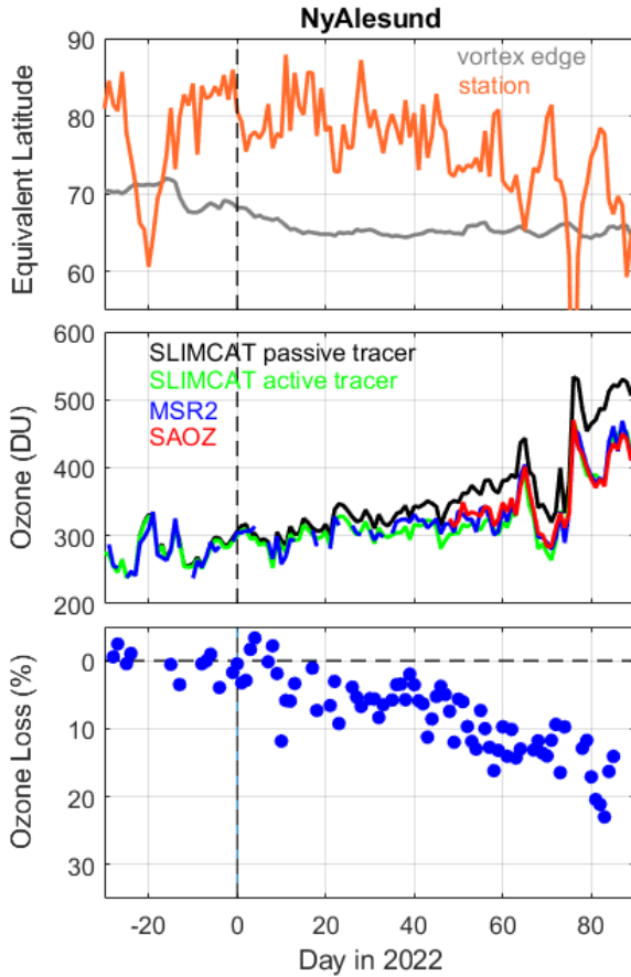
185 Figure 2. Top panel: evolution of the position of the 2021/2022 vortex edge over Ny-Alesund station in equivalent latitude scale at the 475 K isentropic level. Middle panel: evolution of ozone columns at Ny-Alesund from reanalysis MSR2 fields, SAOZ observations and simulated by SLIMCAT in 2021/2022. Bottom panel: evolution of ozone loss (in %) at Ny-Alesund derived from OBS merged dataset (see the text) and the SLIMCAT passive tracer in 2021/2022 winter.
