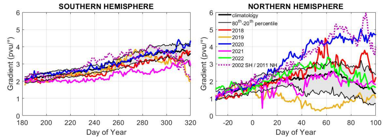
255 Figure 8. As Fig. 5 but for the PV gradient in the vortex edge as defined in Pazmiño et al. (2018) using ERA5 reanalyses.
