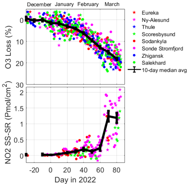
205 Figure 3. Top panel: time series of observed ozone loss (%) inside the vortex above each SAOZ station for the 2022 NH winter. Bottom panel: Time series of the amplitude of the \text{NO}_2 diurnal variation ( \text{NO}_2 sunset – \text{NO}_2 sunrise) inside the vortex above SAOZ stations. The 10-day running median and standard error of the median (IP68/2, see the text) are superimposed by the black line on both panels.
