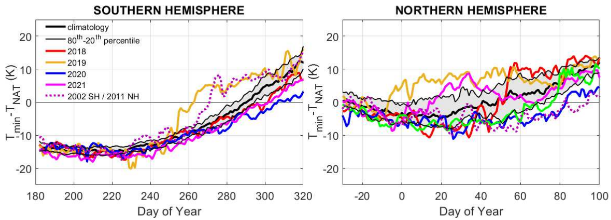
250 Figure 6. As Fig. 5 but for temperature anomaly at 475 K using ERA5 reanalyses.
