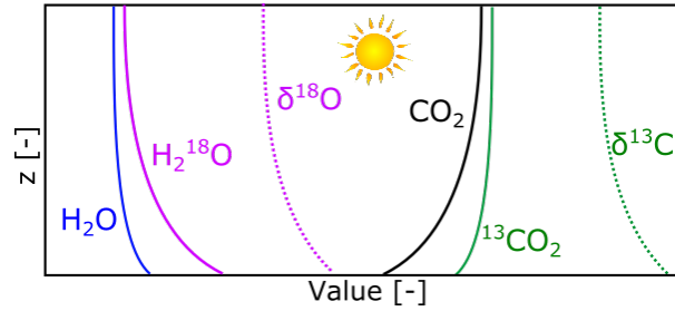
Figure 1. Conceptual view of the idealized gradients of mole fractions and \delta -values in the atmospheric surface layer (ASL) during midday ( z/L_{ob} < 0 ) over a vegetated area.
