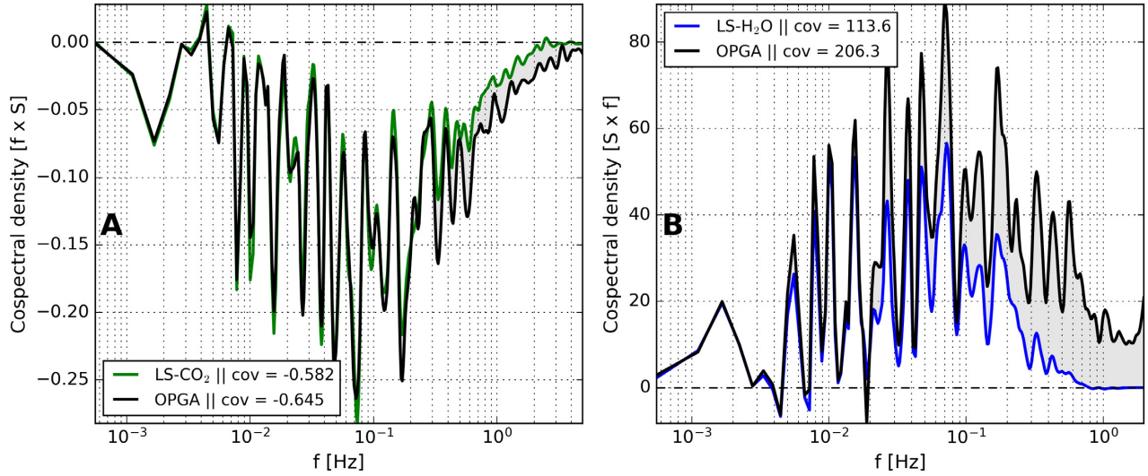
Figure 5. Comparison of the cospectra of w' and q' from both the closed path laser spectrometers and the OPGA of the Eddy Covariance station. Panel A represents the \text{CO}_2 - w cospectra, and panel B the \text{H}_2\text{O} - w cospectra. The spectra are based on a 30-minute data interval taken during the measurement period starting at 12:00 on July 25 th 2021.
