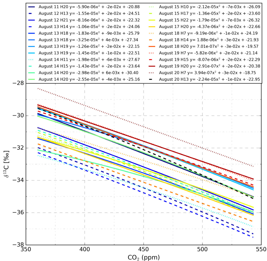
Figure A3. Mole fraction dependence of the CO 2 laser spectrometer during operation at another measurement site. As during the measurement period described in this document the isotopic composition measurements were unstable at timescales of tens-of-minutes due to instrument instability. Even though the absolute isotopic composition varied strongly over hourly timescales, mole fraction dependencies remained relatively constant during the 9 day period. The calibrations shown were made using a system that traps a calibration sample in the instruments sample cell. After flushing the sample cell with calibration gas 4 times, the final gas sample was trapped and measured for 5 minutes. Data from the last 3 minutes was averaged and used to fit calibration lines. The 3-minute plateaus were all stable below \sigma -CO 2 of 1 \mu\text{mol mol}^{-1} . This process was repeated at 4 CO 2 concentration levels to derive one of the plotted calibration lines.
