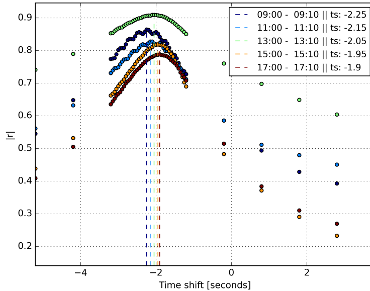
Figure 4. Example of the correlation coefficient ( r ) based time shifts algorithm. In this case the shift between the EC station and the Picarro L2130-i is determined using the \text{H}_2\text{O} mole fraction measurements of both instruments. The different colors each represent a 10-minute section of data on July 25 th , as indicated in the legend. Each dashed vertical line indicates the optimal time shift of the two 10-minute data sections. The derived time shift values are provided in the legend. A negative time shift indicates that the laser spectrometer is delayed compared to the EC system. Note that during this period the instrument clocks were drifting approximately linearly with respect to each other.
