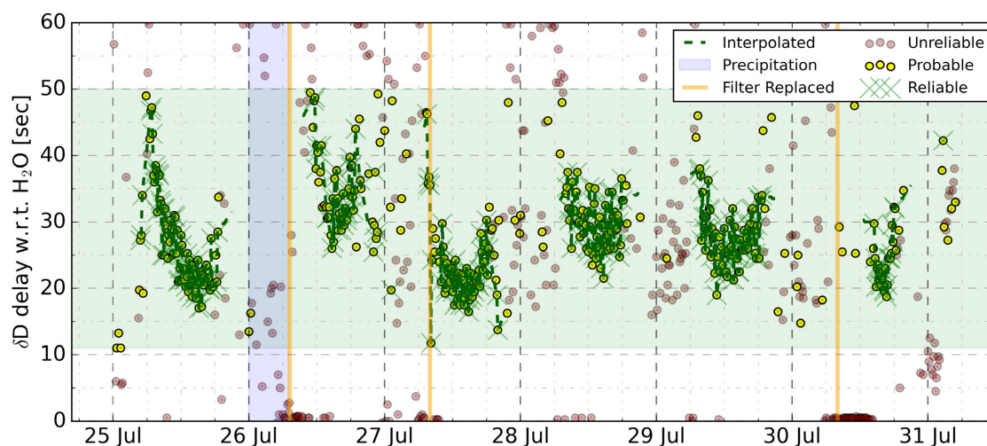
Figure 7. Time shifts between the \delta D and H 2 O signals of the L2130-i analyzer. All symbols represent a 10 minute interval for which a time shift was derived. The red symbols indicate those intervals where the time shift was based on a low correlation coefficient ( r < 0.25 ) and/or unlikely magnitude. The yellow symbols indicate that the time shift has a magnitude fitting within the general pattern of time lags (empirically set light green window) and an r > 0.25 (See Fig. 4). The green symbols indicate the data points which are part of a sequence of reliable "yellow" points. The dashed green line fitted through the green symbols was used to align the \delta and H 2 O signals.
