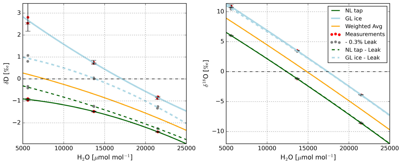
Figure A2. Mole fraction dependency fitted to standard measurements taken after the campaign period (see Fig.3). Note that the measurements are offset to be approximately zero on the y-axis to be able to display both standards in one figure. The solid green and blue lines indicate the fitted dependencies of each standard. To show that the discrepancy between both lines, especially for \delta D , is likely caused by a leak of ambient air, the dashed lines show a simulated mole fraction dependency when an ambient air leak of 0.3% is subtracted from the calibration gas flow. In this simulation, we assumed an ambient H_2O mole fraction of 20000 \mu\text{mol mol}^{-1} , and used the isotopic compositions of the standards and the atmospheric air given in Tab. 1. The magnitude of the ambient air leak was chosen so that it compensates for the suspected real ambient air leak and results in similar mole fraction dependencies for either calibration standard. Note that these corrected dependencies are similar to the Weighted Avg dependency we derived. The larger mole fraction dependence in \delta^{18}O , combined with a smaller absolute difference between the delta values of the calibration standards and ambient air (see Tab. 1), results in a much less pronounced effect of the leak in \delta^{18}O - H_2O
