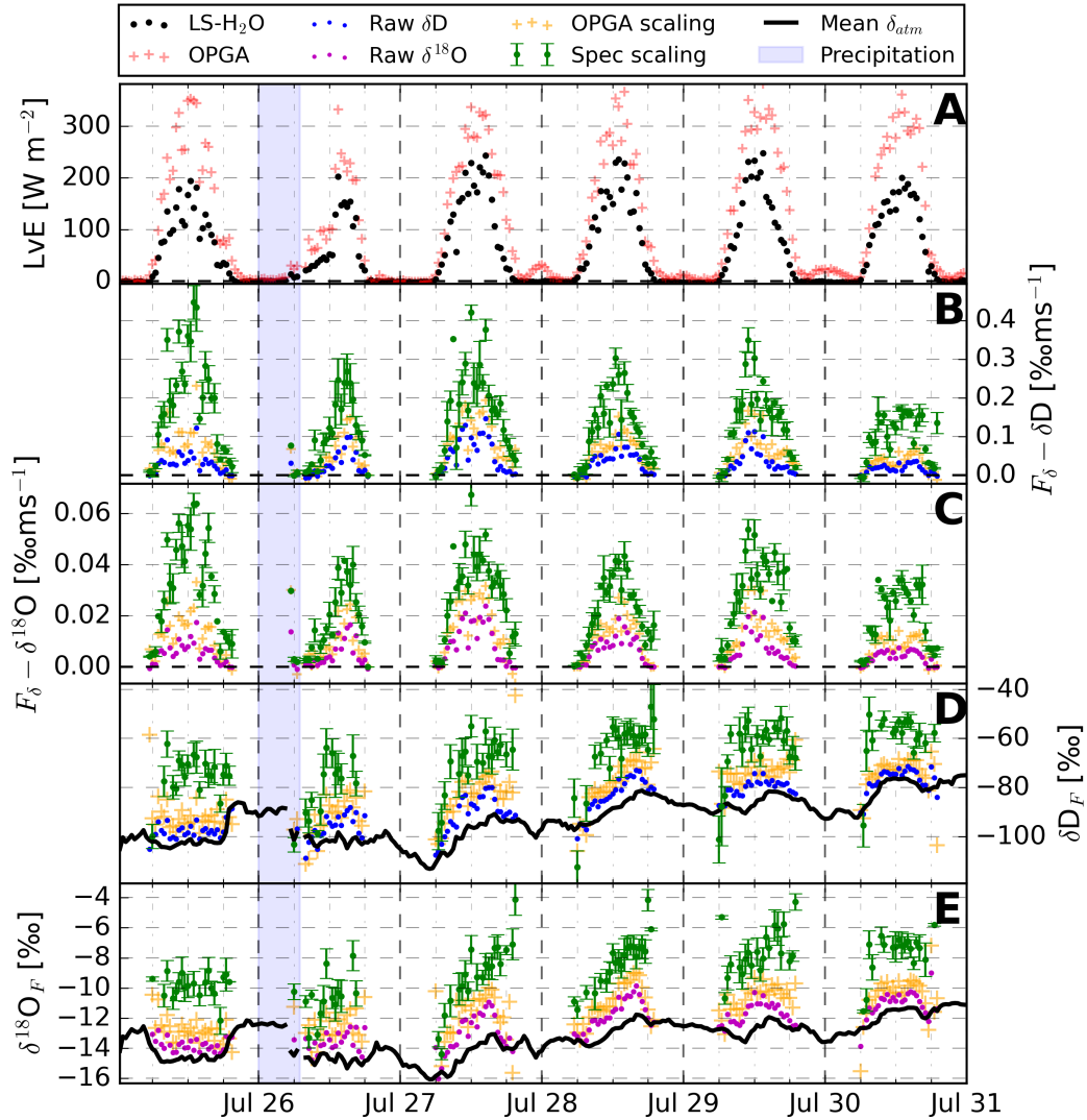
Figure 9. 30-minute \text{H}_2\text{O} exchange fluxes over the 6-day measurement period in Spain near Mollerussa. Panel A shows the evolution of L_vE measured by the LS- \text{H}_2\text{O} and OPGA. Panel B and C display the \delta -flux derived using Eq. (2), including the uncertainty estimate propagated from a 68% confidence interval in fitting the spectral scaling method (Sect. 4.4). Panel D and E indicate the isotopic composition of the vertical flux ( \delta^h X_F ) and the atmospheric background ( \delta^h X_{atm} , black line), including the propagated 1\sigma errors in the fluxes. Panels B through E all contain three different symbols. The full circles represent the raw \delta -fluxes or \delta^h X_F , while the yellow and green markings indicate the corrected ones. These corrections are based on OPGA scaling like is common in isotope flux research (yellow), or on the Spectral scaling technique we detail in Sect. 4.3.2 (green).
