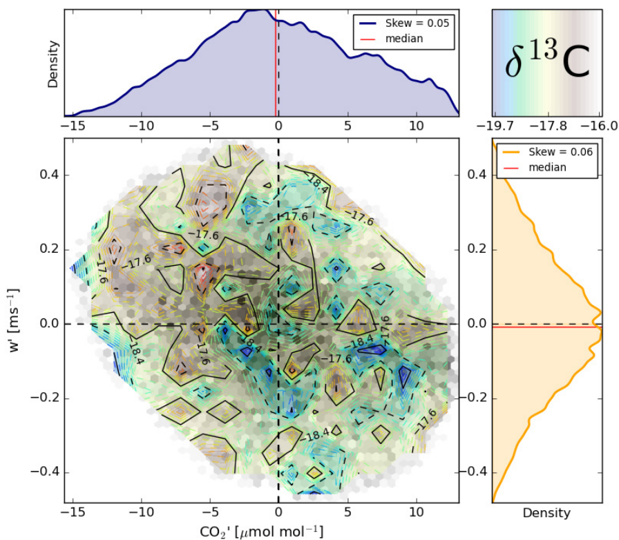
Figure 10. The land-atmosphere exchange of CO 2 within one 30 minute interval including the effect on \delta^{13}\text{C} . The interval was taken from July 25 th at 14:30 UTC. The isotopic composition is indicated as a coloured contour plot over the w' and \text{CO}_2' parameter space which itself is plotted in black. Note that only the 90 th percentile contour of the quadrant figure is shown to allow for increased detail around the relevant dense center of the plot and prevent outliers in isotopic composition, CO 2 concentration and vertical wind speed to become dominant. Additionally, note that the absolute value of \delta^{13}\text{C} is off.
