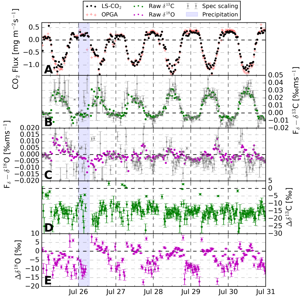
Figure 8. 30 minute \text{CO}_2 exchange fluxes over the 6 day measurement period above an alfalfa crop field near Mollerussa, Spain. Panel B and C display the \delta -flux derived using Eq. (2), including the uncertainty estimate propagated from a 68% confidence interval in fitting the spectral scaling method (Sect. 4.4). Panel D and E show the difference in isotopic composition between the vertical exchange flux and atmosphere ( \delta^h X_F - \delta^h X_{atm} ), including the propagated 1\sigma uncertainty. The difference is plotted instead of both variables separately to eliminate the effect of instrument drift (see Sect. 4.1 on calibrations).
