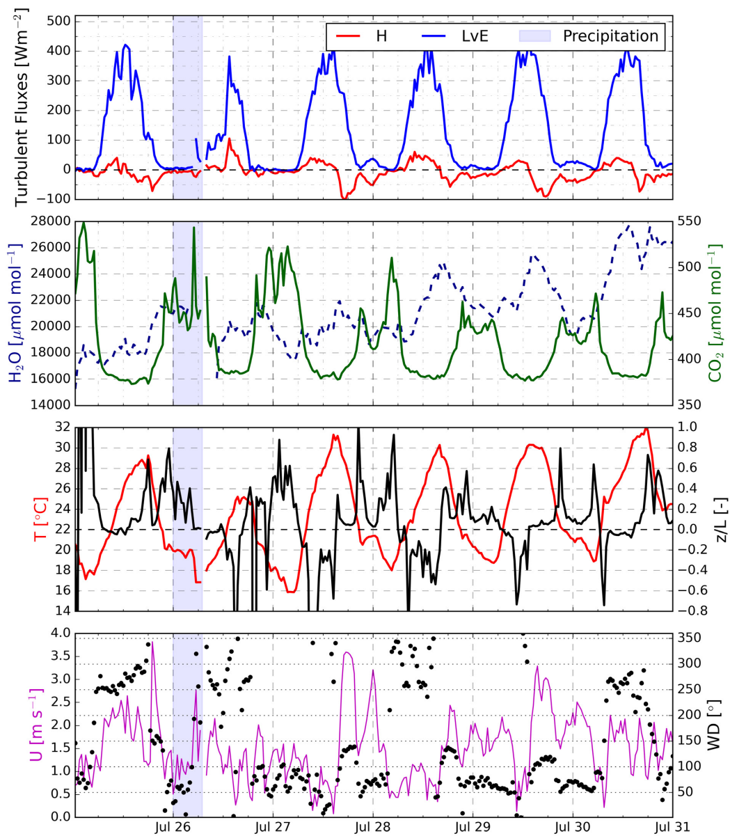
Figure A1. Basic meteorological variables measured using the EC-system and the OPGA. Except for the precipitation event on the 26 th , relatively steady flux, stability and wind regimes can be seen. The \text{H}_2\text{O} mole fraction is least stable, and increases steadily from 18000 to 26000 \mu\text{mol mol}^{-1}
