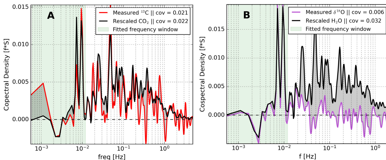
Figure 6. Cospectral flux comparison of \delta^{18}\text{O} (of \text{H}_2\text{O} ) with \text{H}_2\text{O} (from EC) in panel A, and of \delta^{13}\text{C} with \text{CO}_2 (from EC) in panel B. All cospectra were calculated with respect to w' . The \text{CO}_2 and \text{H}_2\text{O} spectra were re-scaled to match the isotopic exchange spectra at timescales longer than 100 seconds. The spectra are based on a 30 minute data interval taken during the measurement period starting at 14:00 on July 25 th 2021.
