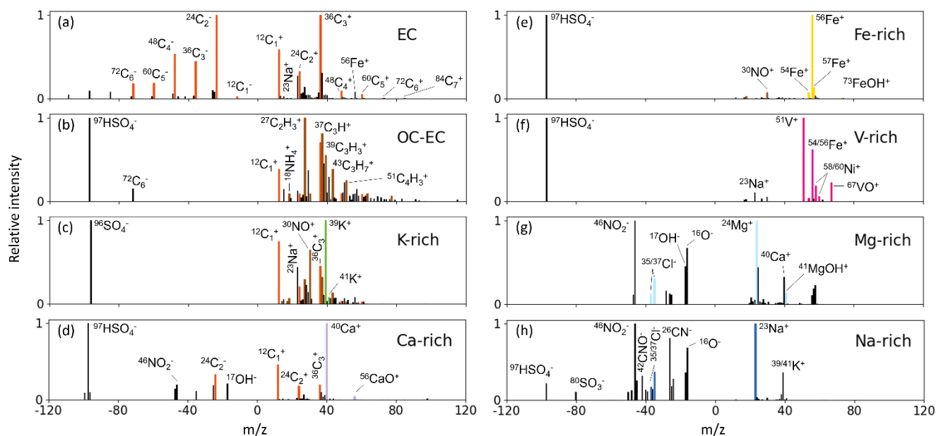
210 Figure 1: Representative mass spectra of aerosol particles, attributed to one of eight classes of our labeled dataset. The positive and negative mass spectra are normalized separately according to their highest ion peaks. The highlighted ion signals are the signature peaks to distinguish different particles.
