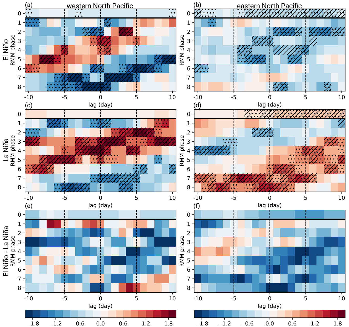
Figure 4. Same as Fig. 3, but for (a) the western and (b) eastern North Pacific during El Niño, and (c) the western and (d) the eastern North Pacific during La Niña, and the difference between El Niño and La Niña for (e) the western and (f) the eastern North Pacific.
