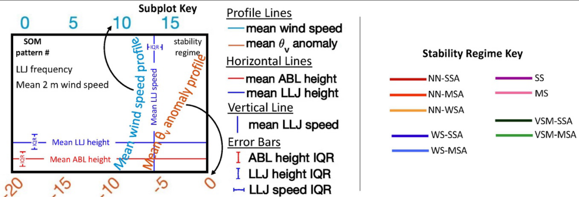
450 Figure 4. As in Fig. 2, but with mean virtual potential temperature ( \theta_v ) anomaly profile (orange line, bottom x-axis) and mean wind speed profile (baby blue line, top x-axis) for all radiosonde profiles mapped to each SOM pattern. The 455 horizontal red line in each subplot is the average ABL height, with the red error bar indicating the interquartile range (IQR). The horizontal blue line in each subplot is the average LLJ core height, with the vertically oriented error bar indicating the IQR. The vertical blue line in each subplot is the average LLJ core speed, with the horizontally oriented error bar indicating the IQR. Each subplot also has written the frequency of LLJs and average 2 m wind speed for that SOM pattern, written below the pattern number.
