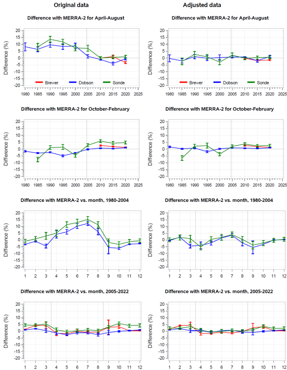
5 Figure 3. (left) Differences between MERRA-2 data and Dobson (blue), Brewer (red), and ozonesonde (green) total ozone in percent as a function of the year ( two upper panels) and month of year ( two bottom panels) for original data. Comparison was done for two seasons: April-August and October-February and for two intervals: 1980–2004 and 2005–2022. (right) The same, but for the data after adjustments were applied to MERRA-2, ozonesonde, and Brewer data . The vertical lines indicate the period from April to August. The error bars correspond to two standard errors of the mean.
