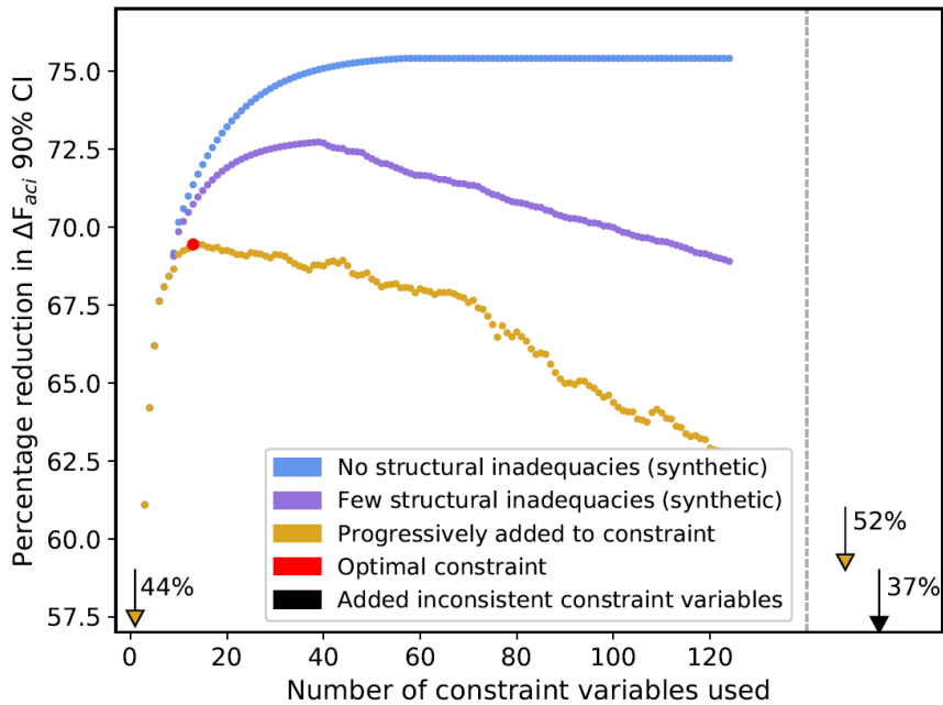
Figure 6: Constraint of \Delta F_{aci} and the effect of varying the number of constraint variables used. We show the effect of progressively adding constraint variables with the greatest influence on \Delta F_{aci} uncertainty (orange), alongside synthetic examples of how the constraint might improve with very few, or no structural model inadequacies (purple and blue respectively). In each case, only the first 125 of 225 N_d -pairwise consistent constraint variables are shown. Arrows indicate the constraint of \Delta F_{aci} using the single strongest constraint variable (44%), all 225 N_d -pairwise consistent constraint variables (52%) and all 450 constraint variables (37%), including those associated with identified structural inadequacies at the regional level (e.g. Fig. 4 and 5).
