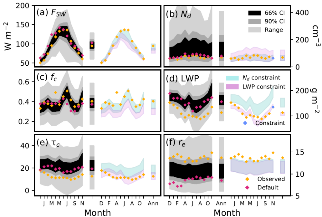
495 Figure 4: Seasonal cycles of North Atlantic mean radiative fluxes and cloud properties before and after observational constraint using a single month of observations. Model output for individual months spanning December 2016 to November 2017 are followed by the annual mean. Credible intervals for the full set of model variants are shown (grey shading) along with satellite-derived observations and the default UKESM1-A model values. Each panel also shows the range (shading) of values from the November N_d constraint (green) and the November LWP constraint (pink; arrows 500 show constraint variable). The orange data point shows the observed variable and month used for the constraint.
