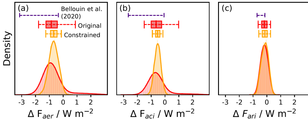
Figure 2. Probability density functions for global, annual mean effective radiative forcings from 1850 to 2014. a) \Delta F_{\text{aer}} , b) \Delta F_{\text{aci}} and c) \Delta F_{\text{ari}} in the original 1 million member sample and after optimal constraint (see Sect. 3.3.2). Box plots show the 5 th , 25 th , 50 th , 75 th and 95 th percentiles. The 5 th and 95 th percentiles from Bellouin et al., (2020) are also shown.
