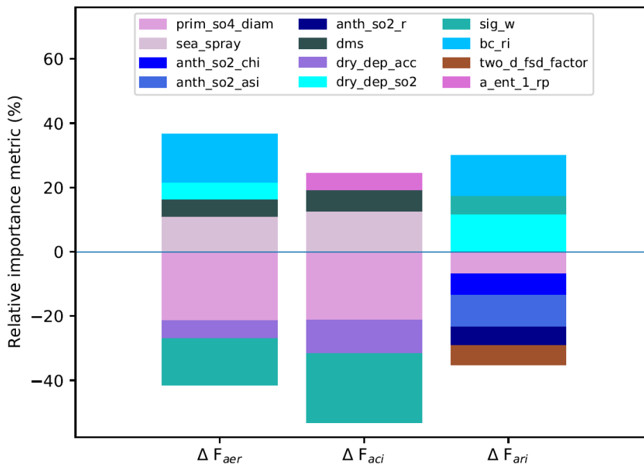
380 Figure 3: Relative importance of model parameters as causes of uncertainty in global mean \Delta F_{\text{aer}} and its components \Delta F_{\text{aci}} and \Delta F_{\text{ari}} . Only parameters with a relative importance of 5% or larger are shown. Positive values correspond to parameters where increasing the parameter value causes median values of \Delta F_{\text{aer}} , \Delta F_{\text{aci}} or \Delta F_{\text{ari}} to become weaker (less negative) across the set of 1 million model variants.
