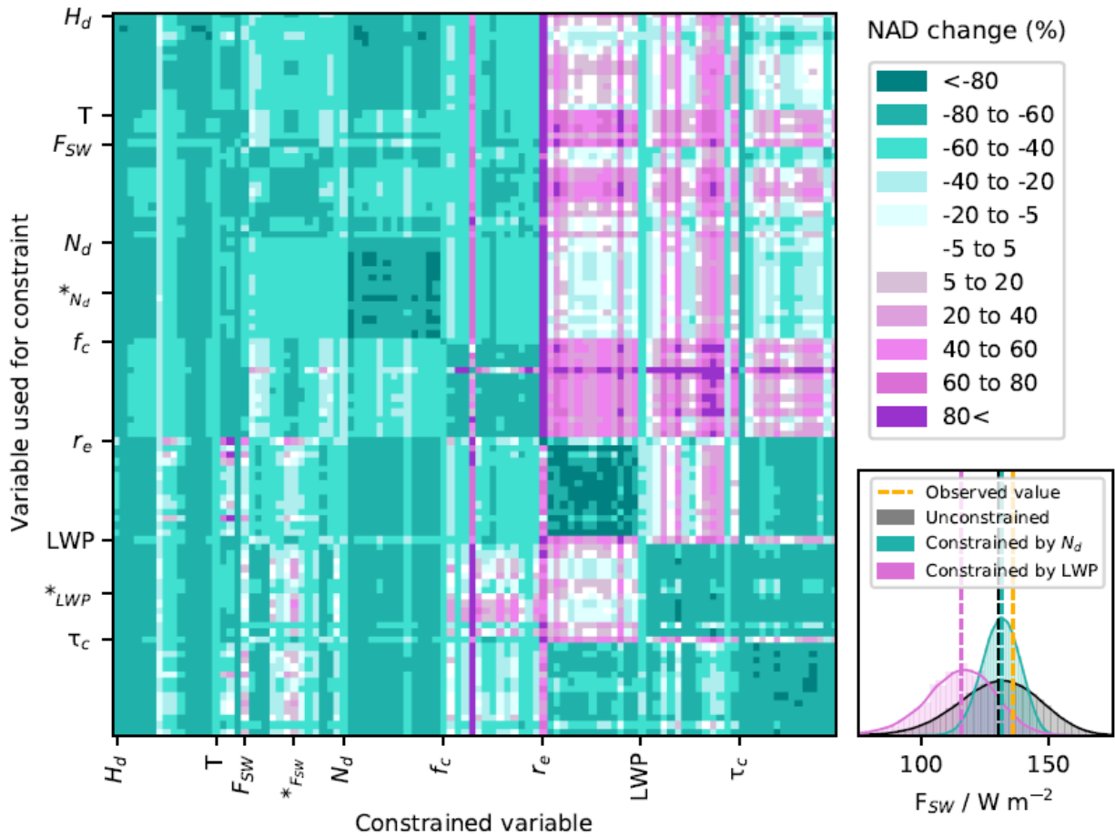
535 Figure 5: Pairwise comparisons of North Atlantic constraint variables (and hemispheric difference, H_d ) showing how constraint of one variable affects all others. The y-axis labels refer to variables used to constrain the model output and the x-axis labels refer to variables whose values have been consequently constrained. For each state variable, the pixels in the first row/column are the seasonal amplitude, followed by individual months from January to December and the annual mean. Transect variables are within the section labelled “T”. Shading indicates the percentage change in 540 average NAD after constraint. In the bottom-right panel we exemplify the effect of constraint on average NAD in two pixels in terms of probability density functions of July F_{SW} in the unconstrained set of model variants (black), in the set constrained to match July N_d observations (green), and in the set constrained to match July LWP (pink). Vertical dashed lines represent the observed F_{SW} value and median values in the unconstrained and constrained sets of model variants.
