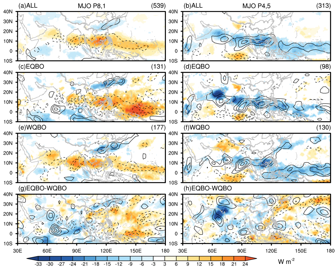
Figure 1. Composite OLR (shadings; units: W m^{-2} ) and 200-hPa divergence (contours; units: s^{-1} ; interval: 3 \times 10^{-6} ) anomalies at the Madden-Julian oscillation (MJO) phases (left) 8-1 and (right) phases 4-5 for (a, b) total days, (c, d) easterly QBO days, (e, f) westerly QBO days and (g, h) EQBO-WQBO difference (dashed lines show convergence anomalies). Only the composite anomalies that are statistically significant at 95% confidence level are shown according to the t-test. The number of days used for each composite map is printed at the top-right corner. The ERA5 reanalysis is shown. The composite OLR and 200-hPa divergence anomalies based on the NCEP/NCAR reanalysis are shown in Figure S17.
