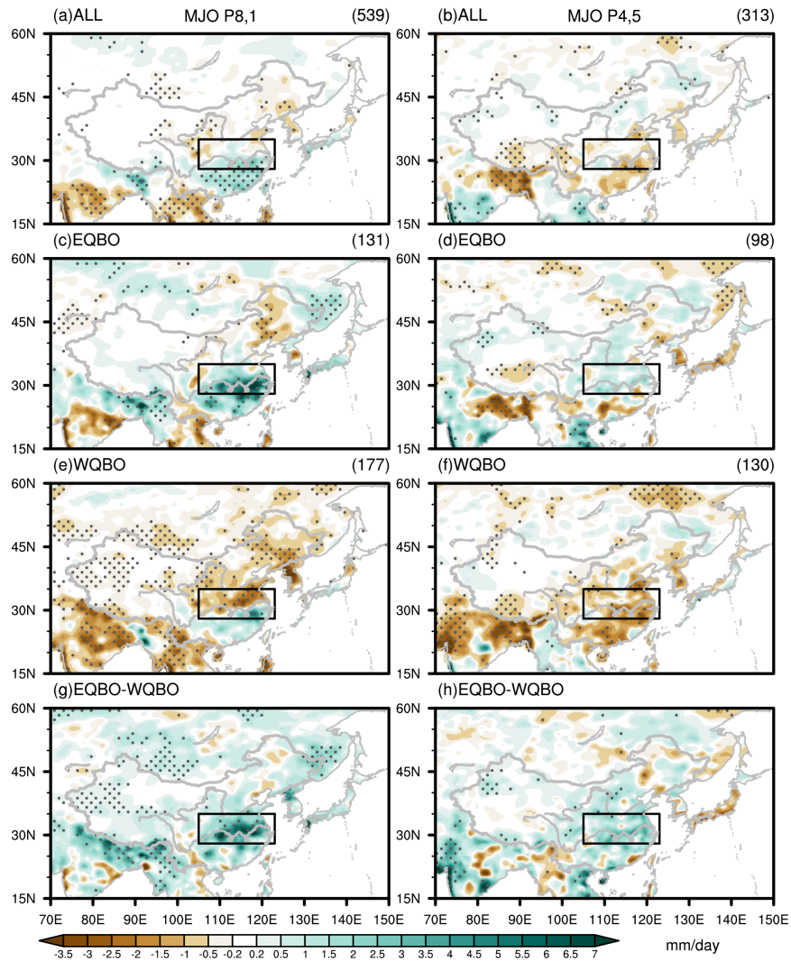
145 Figure 2. Composite rainfall anomalies (shadings; units: mm/day) at the MJO phases (left) 8-1 and (right) phases 4-5 for (a, b) total days, (c, d) easterly QBO days, (e, f) westerly QBO days and (g, h) EQBO-WQBO difference. The dots denote the composite anomalies at 95% confidence level are shown according to the t-test. The number of days used for each composite map is printed at the top-right corner. The composite rainfall anomalies with the interannual ENSO signals removed are shown in Figure S1.
