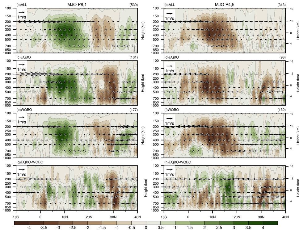
255 Figure 5. Composites latitude-pressure cross section of meridional circulation anomalies (vectors; units: m/s, Pa/s) and vertical velocity anomalies (shadings; units: 0.01 Pa/s) averaged from 110–120°E during the MJO phases (left) 8-1 and (right) phases 4-5 for (a, b) total days, (c, d) easterly QBO days, (e, f) westerly QBO days and (g, h) EQBO-WQBO difference (brown denotes upward motion). The vertical velocity anomalies have been multiplied by -10 to better show the vectors. The ERA5 reanalysis is shown. The composite meridional circulation anomalies based on the NCEP/NCAR reanalysis are shown in Figure S20.
