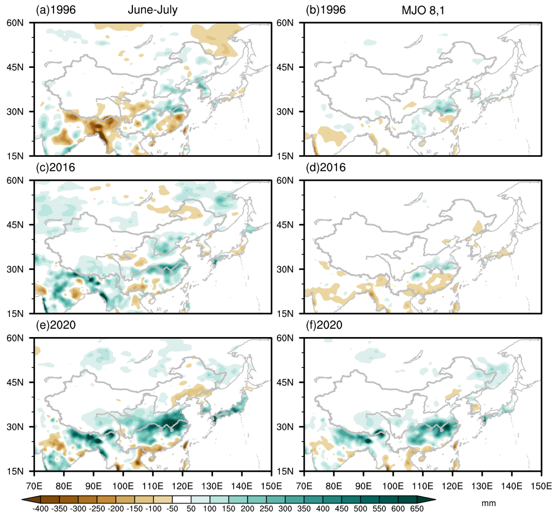
305 Figure 7. Total precipitation anomalies (units: mm) in June-July (left) and contributions by MJO phases 8-1 (right) for (a, b) 1996, (c, d) 2016, and (e, f) 2020.
