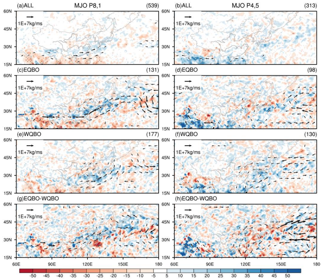
Figure S19. Composites vertically integrated moisture flux (VIMF) anomalies (vectors; units: 10^7 \text{ kg m}^{-1} \text{ s}^{-1} ) and the VIMF horizontal convergence (VIMFC) anomalies (shadings; units: \text{kg m}^{-2} \text{ s}^{-1} ) using the ERA5 reanalysis during the MJO phases (left) 8-1 and (right) phases 4-5 for (a, b) total days, (c, d) easterly QBO days, (e, f) westerly QBO days and (g, h) EQBO-WQBO difference. Note that only the VIMF anomalies larger than 0.5 \times 10^7 \text{ kg m}^{-1} \text{ s}^{-1} are shown. The VIMFC anomalies that are statistically significant at the 95% confidence level are dotted.
