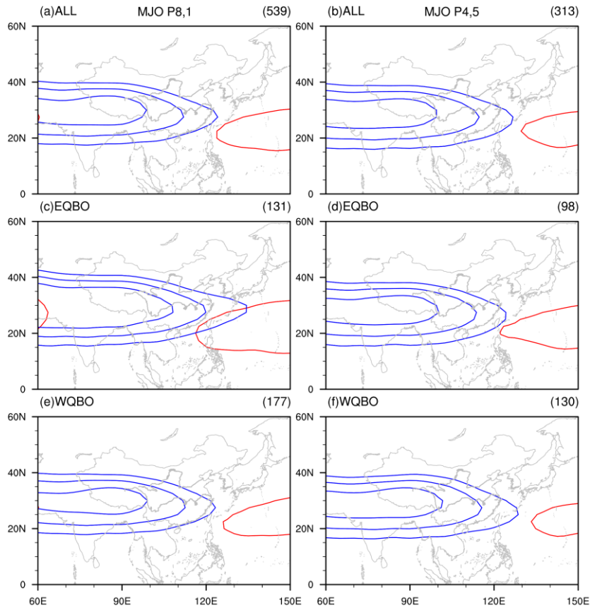
Figure S18. Composites South Asia High (SAH) at 100 hPa and western Pacific high (WPH) at 500 hPa using the NCEP-NCAR reanalysis during the MJO phases (left) 8-1 and (right) phases 4-5 for (a, b) total days, (c, d) easterly QBO days, and (e, f) westerly QBO days. Three height contours (16720, 16760, 16800 gpm) are plotted for the SAH, and one contour (5880 gpm) is plotted for the WPSH.
