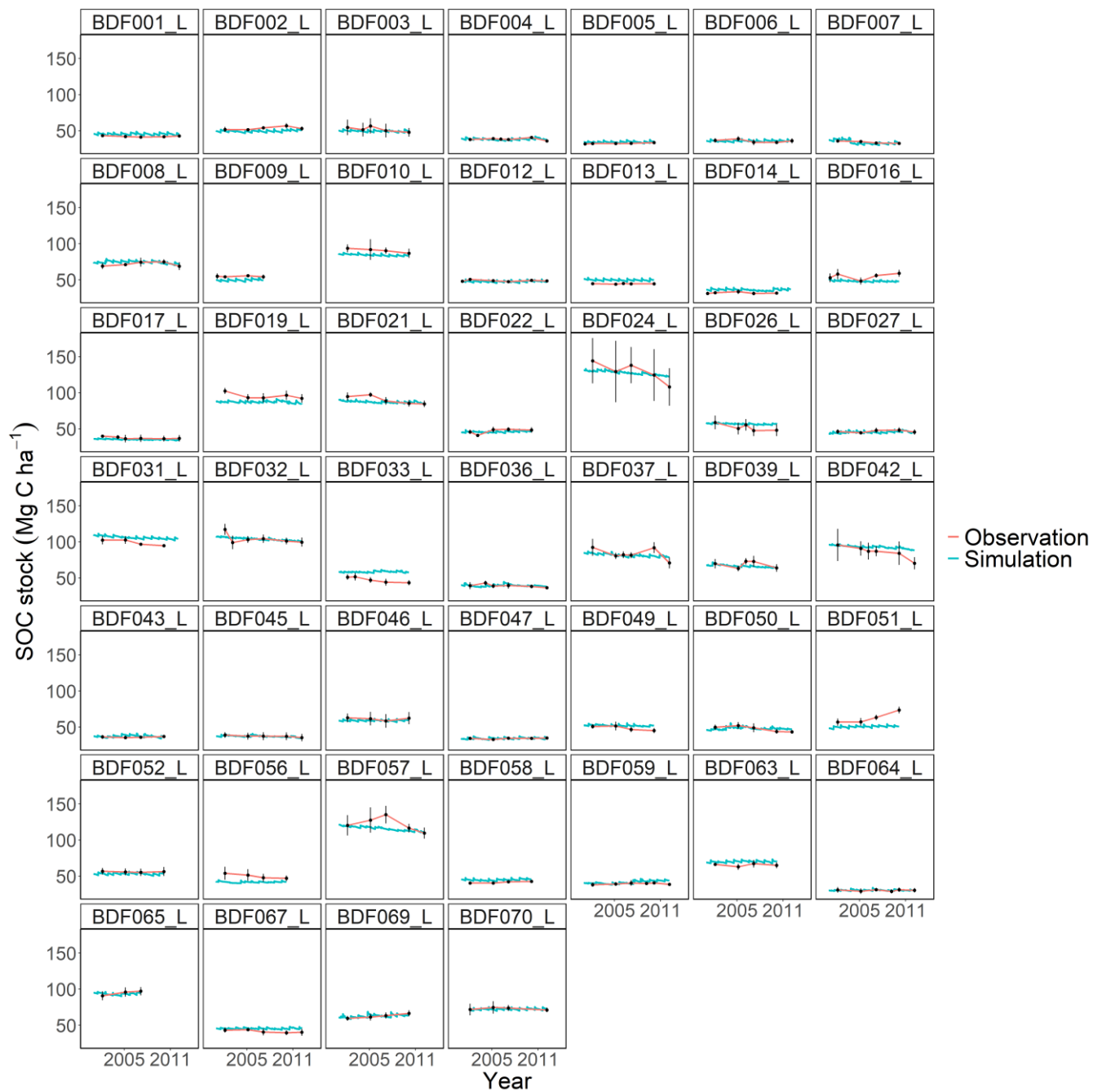
590 Figure 12. Performance of the modified and calibrated MONICA model for each individual site. The first 10 measured years were excluded.
