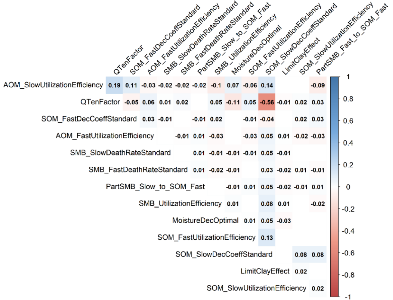
575 Figure H1. Correlation matrix quantifying the statistical relationship between the prior probability distributions of the SOM submodel parameters.
