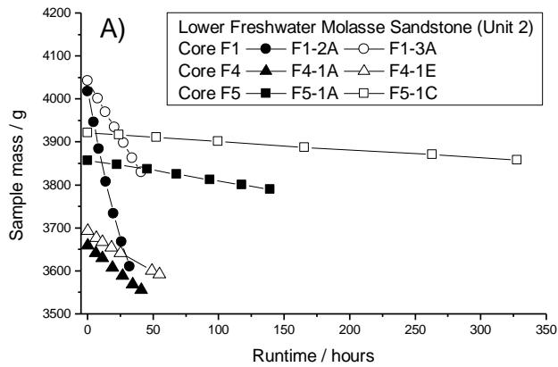
Figure 4: A) Mass evolution over six runs of six samples from the Lower Freshwater Molasse (Unit 2). Two samples each were tested from three cores, all sourced from the same site. Erosion rates vary considerably, by a factor of up to 63 between cores and up to 2.5 between samples from the same core. B) Mass evolution over six runs of three samples from the Hauptrogenstein oolitic limestone (Unit 5), cut from two different cores. Here, much less variability has been observed, with a factor of up to 2.3 between cores, and 1.8 between samples from the same core.
