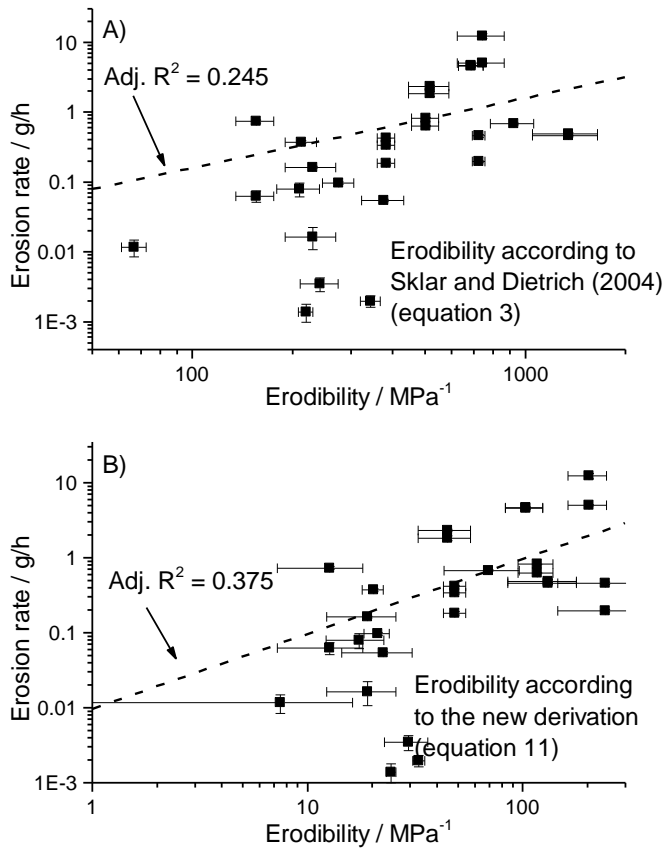
380 Figure 9: Erosion rates measured in the mills compared to theoretical predictions. The dashed lines show a linear fit to the logarithmized data, with the slope fixed to one, corresponding to a proportional relationship. A) Erodibility according to Sklar and Dietrich (2004), based on Engle's (1978) theory of brittle fracture (eq. 3). The fit gives an adjusted R 2 of 0.245 and a prefactor of 1.58 \times 10^{-3} . B) Erodibility according to the extended model (eq. 11). The fit gives an adjusted R 2 of 0.375 and a prefactor of 9.66 \times 10^{-3} . For the plots, the rock resistance coefficients k_{\zeta a} and k_{\zeta} were set to one.
