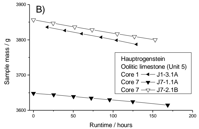
Figure 4: A) Mass evolution over six runs of six samples from the Lower Freshwater Molasse (Unit 2). Two samples each were tested from three cores, all sourced from the same site. Erosion rates vary considerably, by a factor of up to 63 between cores and up to 2.5 between samples from the same core. B) Mass evolution over six runs of three samples from the Hauptrogenstein oolitic limestone (Unit 5), cut from two different cores. Here, much less variability has been observed, with a factor of up to 2.3 between cores, and 1.8 between samples from the same core.
