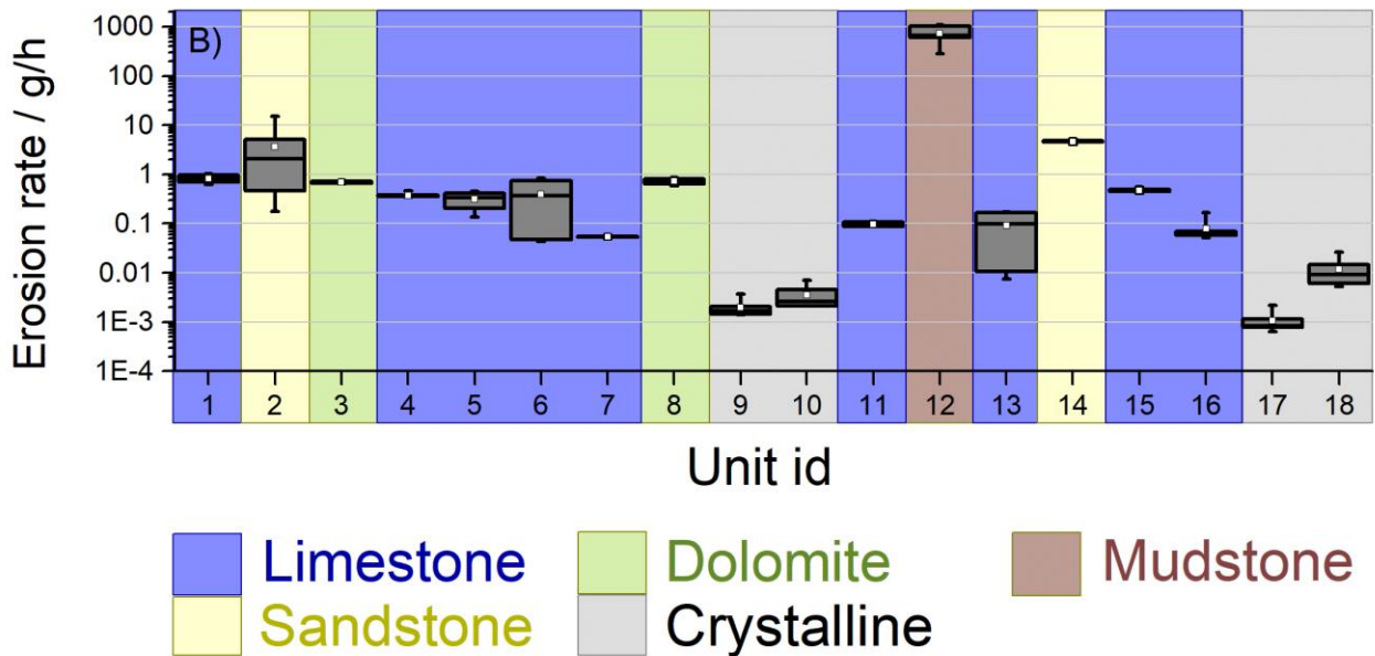
Figure 3: Measured mill erosion rates for all samples (A) and lithological units (B). Gray boxes show the median (central horizontal line), and the 25 th and 75 th percentiles (bottom and top of the box). White squares show the mean, and whiskers the maximum and minimum erosion rates. The display follows the order of Table 1 (core ids, numerical unit id). Colouring denote lithology classes. Sample ids are composed of the leading core id, followed by a letter indicating the position of the sample within the core. Measured erosion rates vary over approximately six orders of magnitude across the different lithologies.
