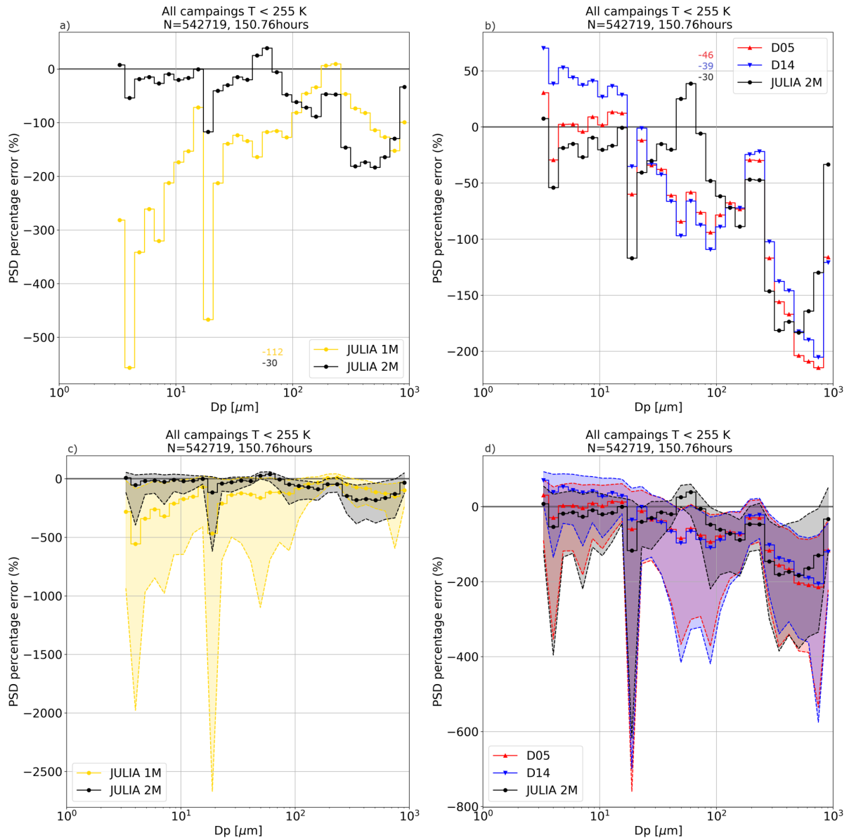
Figure 4. Median of the difference percentage error between the single parameterized-observed PSDs and their corresponding observed parameterized PSDs. (a, c) Comparison between one mode (JULIA 1M: yellow) and two mode parameterization (JULIA 2M: black); (b, d) comparison between parameterizations from the literature (D05: red, D14: blue) and the two-modes parameterization (JULIA 2M: black) of this study. The shadow region in the lower panels correspond to 1-\sigma . y-axis is the median of the difference in number concentration region between the observed (from JULIA database) percentile 25 and the parameterized PSDs in and the percentile 75 . x-axis represent the size bins in \mu\text{m} . A detailed overview of the coefficients of each parameterization is given in Table 3. The numbers inside the panels correspond to the median percentage error over the complete size
