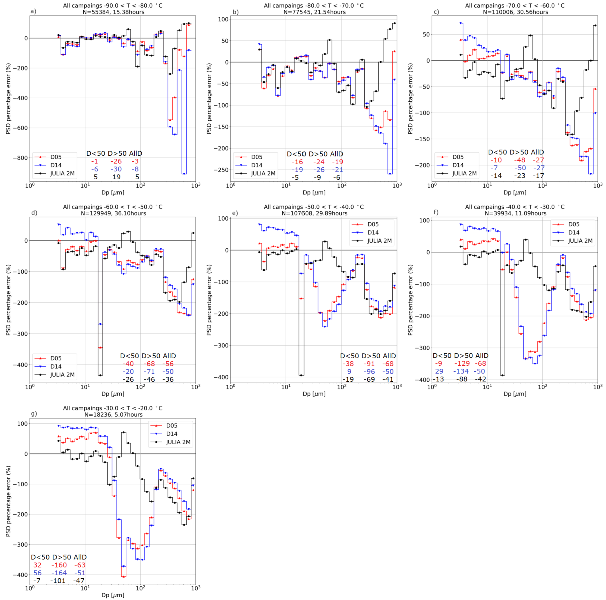
Figure 5. Median of the difference percentage error between the single observed PSDs of all campaigns and their corresponding parametrized PSDs, as in Fig. 4c, but for 10K-10 K temperature ranges. The parameterizations from the literature are: D05 in red and D14 in blue. JULIA 2M (in black) is the proposed new bimodal parameterization. y-axis is the median of the difference in number concentration between the observed and the parametrized PSDs in and the x-axis is the size bins in \mu\text{m} . A detailed overview of the coefficients of each parameterization is given in Table 3. The numbers inside the panels correspond to the median percentage error over the specified size range.
