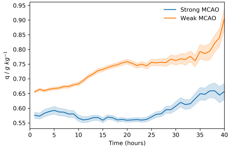
Figure S1. The specific humidity at 750 hPa for strong (MCAO > 3.9 K, blue) and weak (0 K < MCAO < 1.5 K, orange) outbreak events moving away from the ice edge.
