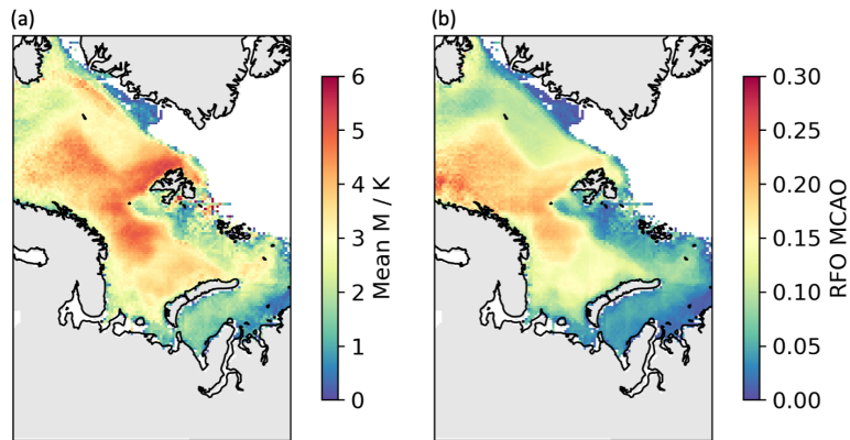
Figure 3. MCAO index ( M ) calculated from ERA5 data for March-October 2008-2014, filtered to only include MCAO events ( M > 0 ) (a) and relative frequency of occurrence for outbreaks (b). Grey represents the land and white represents no data due to sea ice coverage .
