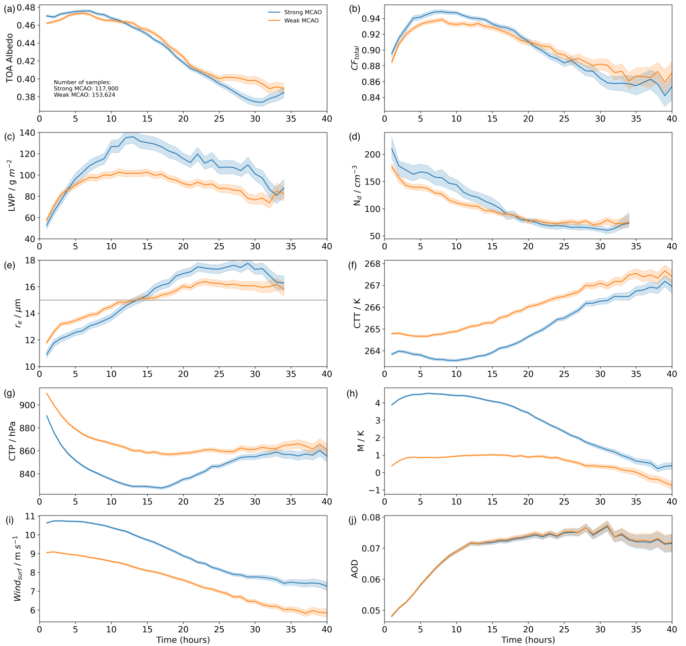
Figure 7. As Figure 6, but for strong ( MCAO-M > 3.9\ K , blue) and weak ( 0\ K < MCAO-M < 1.5\ K , orange) outbreak events moving away from the ice edge.
