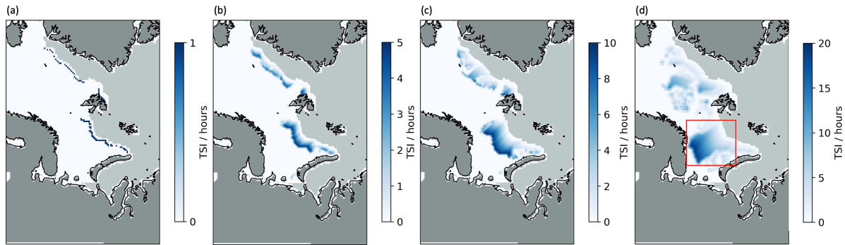
Figure 4. Map-Snapshot of the average ‘time since ice’ trajectory generation for trajectories-generated-(a) one (b) five (c) ten and (d) twenty hours since moving from the ice edge. Dark and light grey represent land and sea ice pixels, respectively. The scale varies between March-October-2008-2014 subplots. The red box in (d) indicates air moving off the ice edge that developed into a marine cold air outbreak. The data is from 1st April 2014.
