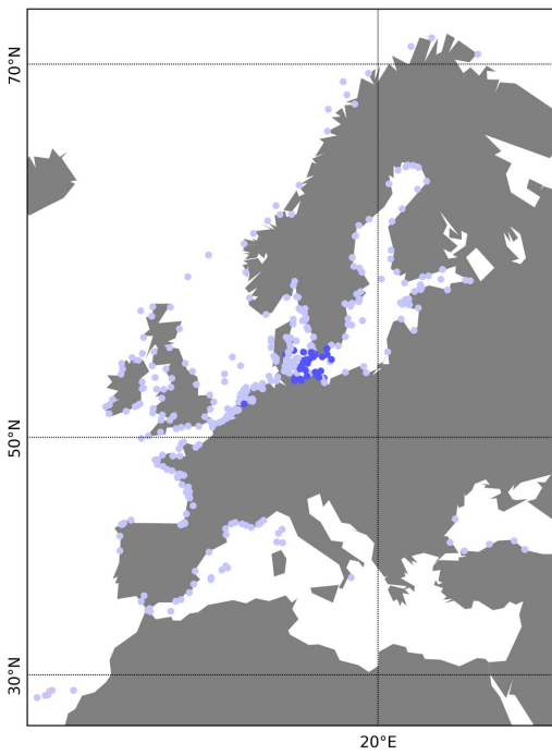
Total sea level: Relative minimum in fall
