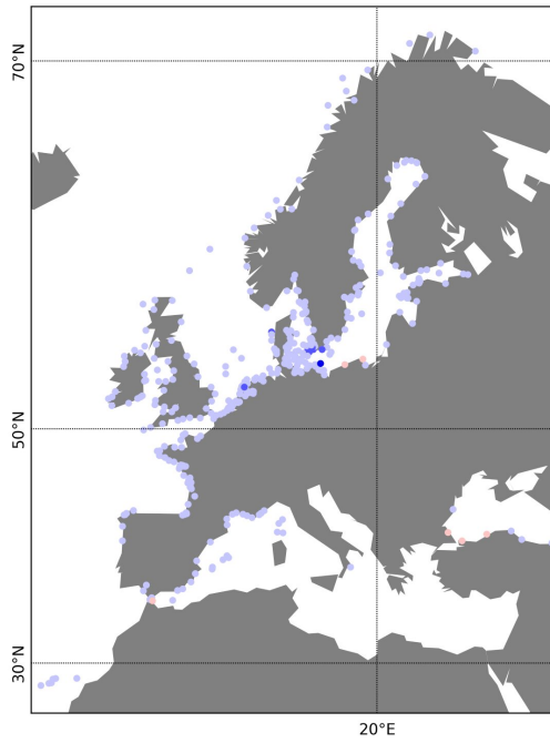
Total sea level: Relative minimum in spring
