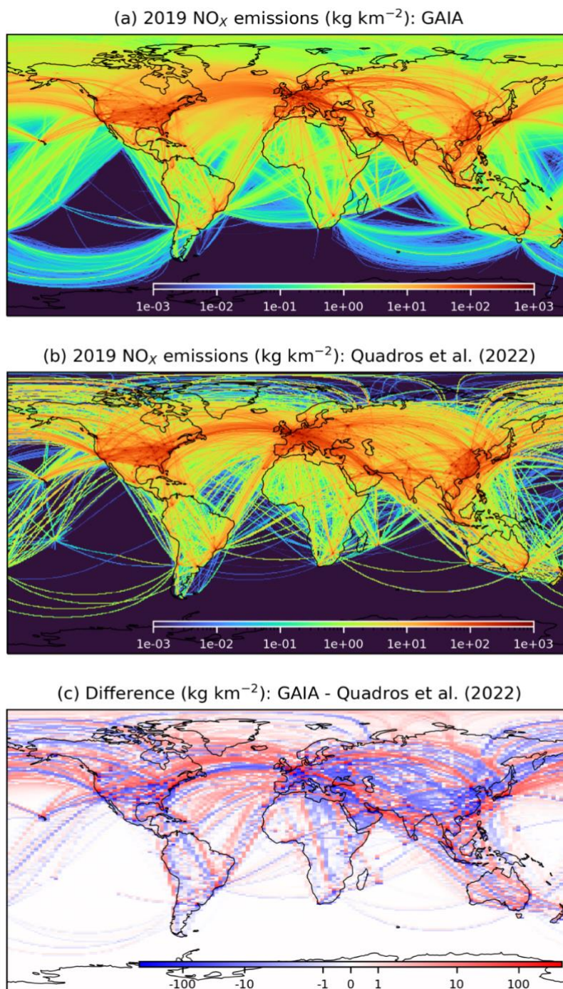
300 Figure 4: Spatial distribution of the 2019 column-integrated \text{NO}_x emissions from (a) GAIA with actual flight trajectories versus (b) estimates from Quadros et al. (2022) which used monthly-averaged flight trajectories, and (c) the absolute difference in column-integrated \text{NO}_x emissions between (a) and (b). Basemap plotted using Cartopy 0.21.1 © Natural Earth; license: public domain.
