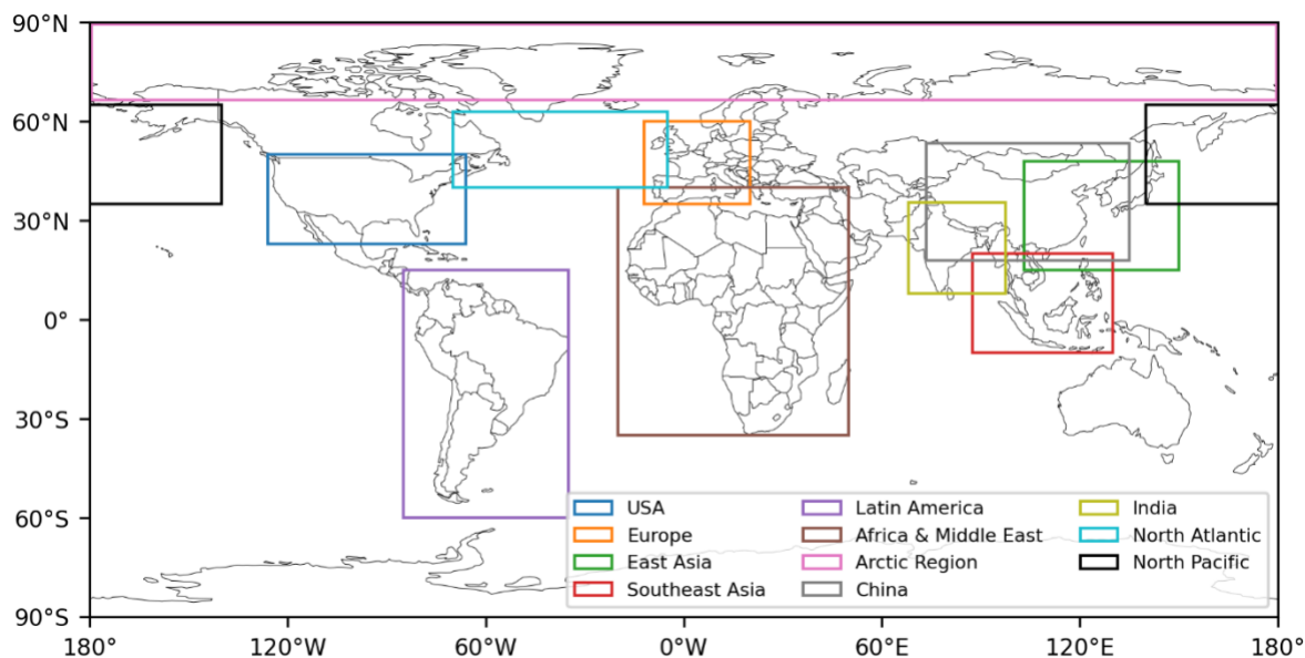
Figure 1: Spatial bounding boxes of the key regions of interest that is used to estimate the regional aviation activity and emissions. The specific dimensions of the bounding boxes are listed in Table 2. Basemap plotted using Cartopy 0.21.1 © Natural Earth; license: public domain.
