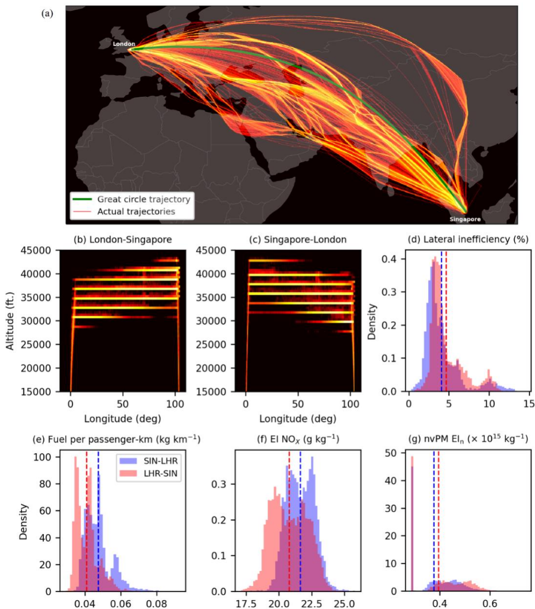
Figure 7: The (a) lateral and (b – c) vertical trajectory that is flown by flights between London Heathrow Airport (LHR) and Singapore Changi Airport (SIN) between 2019 and 2021 ( n = 8705 ), and probability density function of the (d) lateral inefficiency, (e) fuel consumption per passenger-km; (f) EI \text{NO}_x ; and (g) \text{nvPM EI}_n for westbound (SIN–LHR, in blue) and eastbound flights (LHR–SIN, in red). Basemap plotted using Cartopy 0.21.1 © Natural Earth; license: public domain.
