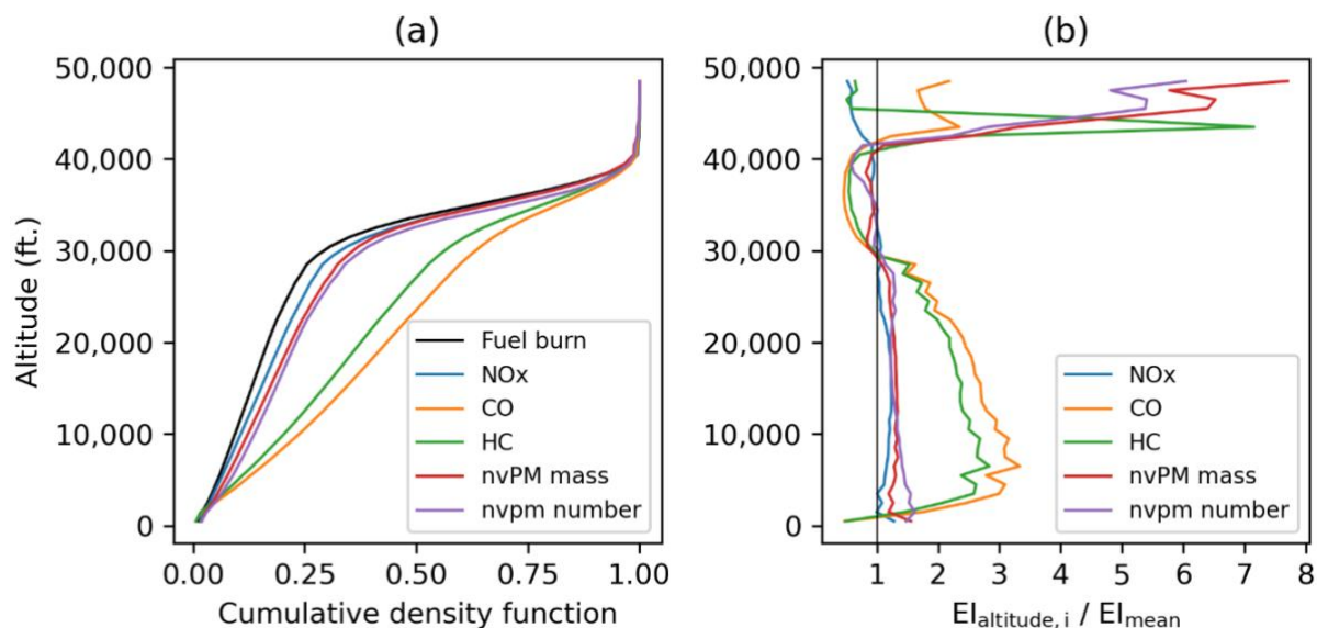
295 Figure 3: (a) Cumulative density function of the 2019 annual fuel burn by altitude, and (b) the ratio of emission indices (EI) for nitrogen oxide (NO x , in blue), carbon monoxide (CO, in orange), hydrocarbons (HC, in green) and nvPM mass (in red) and number (in purple) at different altitudes relative to their respective global mean EI's.
