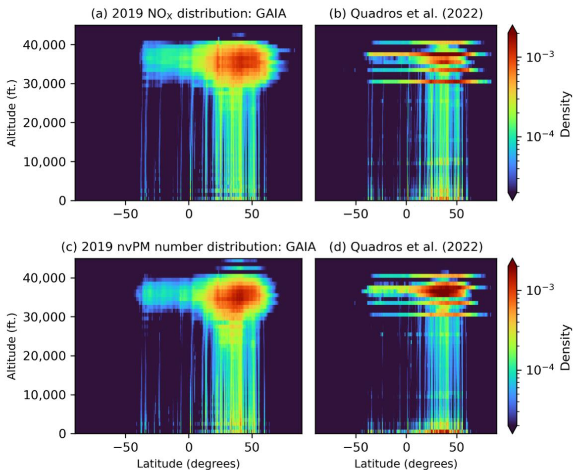
Figure 5: Distribution of the 2019 NO x and nvPM number emissions by latitude and altitude from GAIA with actual flight trajectories (subplots a and c) versus estimates from Quadros et al. (2022) with monthly-averaged flight trajectories (subplots b and d).
