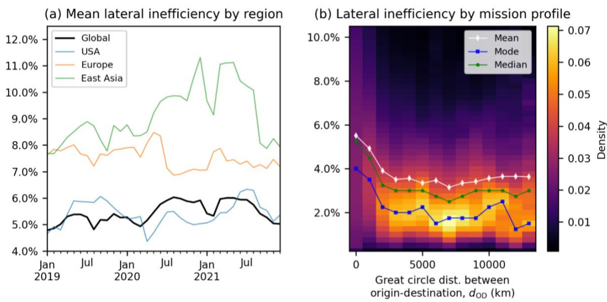
365 Figure 6: The (a) mean lateral inefficiency of flights in different spatial domains (global, USA, Europe, and East Asia); and (b) distribution of lateral inefficiency when flights are categorised by mission profile, defined by the great circle distance between their respective origin and destination airports. These lateral inefficiency statistics excludes the 1.5% of flights, where their erroneous trajectories were replaced with the great-circle path between the origin-destination airport (SI §S1.2).
