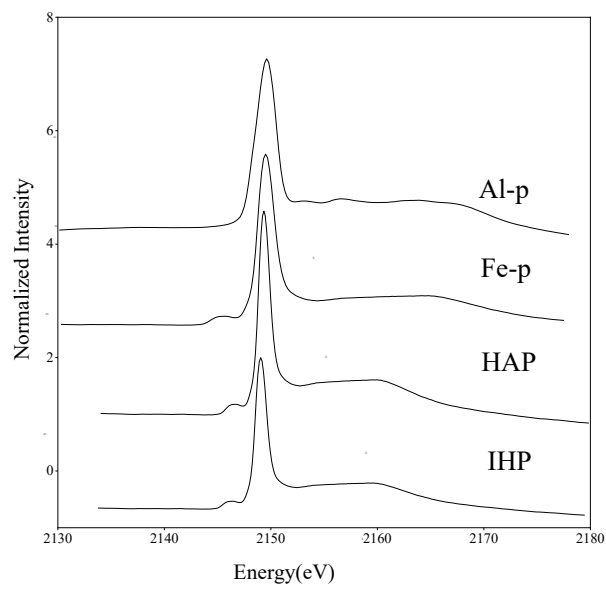
Figure S1. Phosphorus K-edge XANES spectra of P reference compounds
