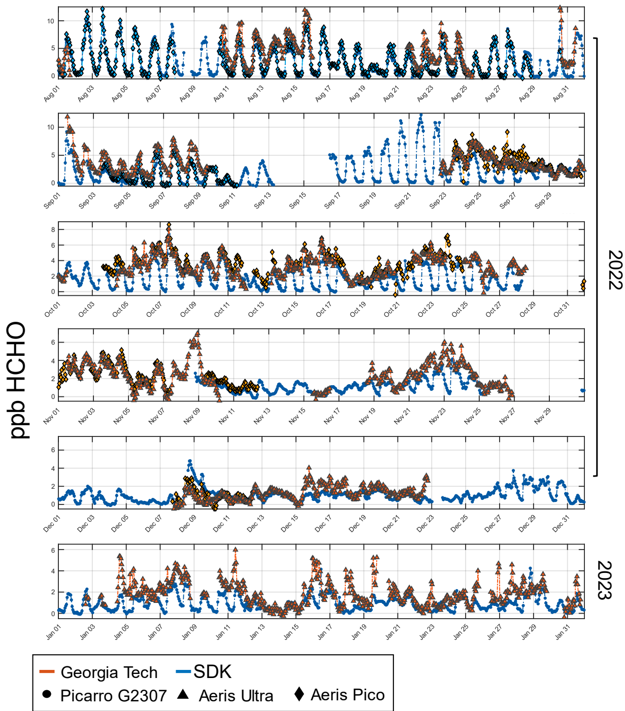
545 Figure 10 – 1 h averaged HCHO time series from Picarro G2307, Aeris Ultra, and Aeris Pico from Aug. 2022 through Jan 2023. Observations at GT show less defined diurnal amplitudes than the SDK site and are on average higher regardless of time of year. Aeris Pico data is sparse past 18 Oct. 2022 as it was periodically dedicated to other experiments.
