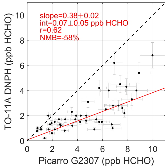
530 Figure 9 – 8 h TO-11A DNPH observations compared to Picarro G2307 observations at the SDK site from June through August 2022. Error bars represent the 10% uncertainty associated with the TO-11A and G2307 measurements.
