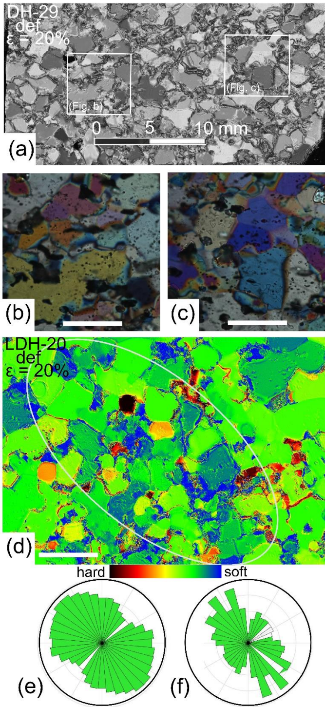
685 Figure 7: Images from thin sections of ice samples showing post-deformation microstructures. (a) Greyscale image through portion of DH-29def showing location of enlargements (b) and (c). (b, c) Plane polarized images illustrating irregular grain structures in DH-29def. White bar scales = 2 mm. (d) A grain softness map (Peternell et al., 2019) of portion of LDH-20def. The blue areas preferentially located along grain boundaries represent Mix-2 + Mix-1 and H 2 O and are soft areas that can accommodate easy glide in the ice in contrast to the hard grains (green and brown). (e) Rose diagrams 690 illustrate the grain shape preferred orientation outside the white ellipse (f) Rose diagram of grain shape within a shear band corresponding to the elliptical area in LDH-20 and is dominated by soft grains and grain boundaries (Peternell et al., 2019).
