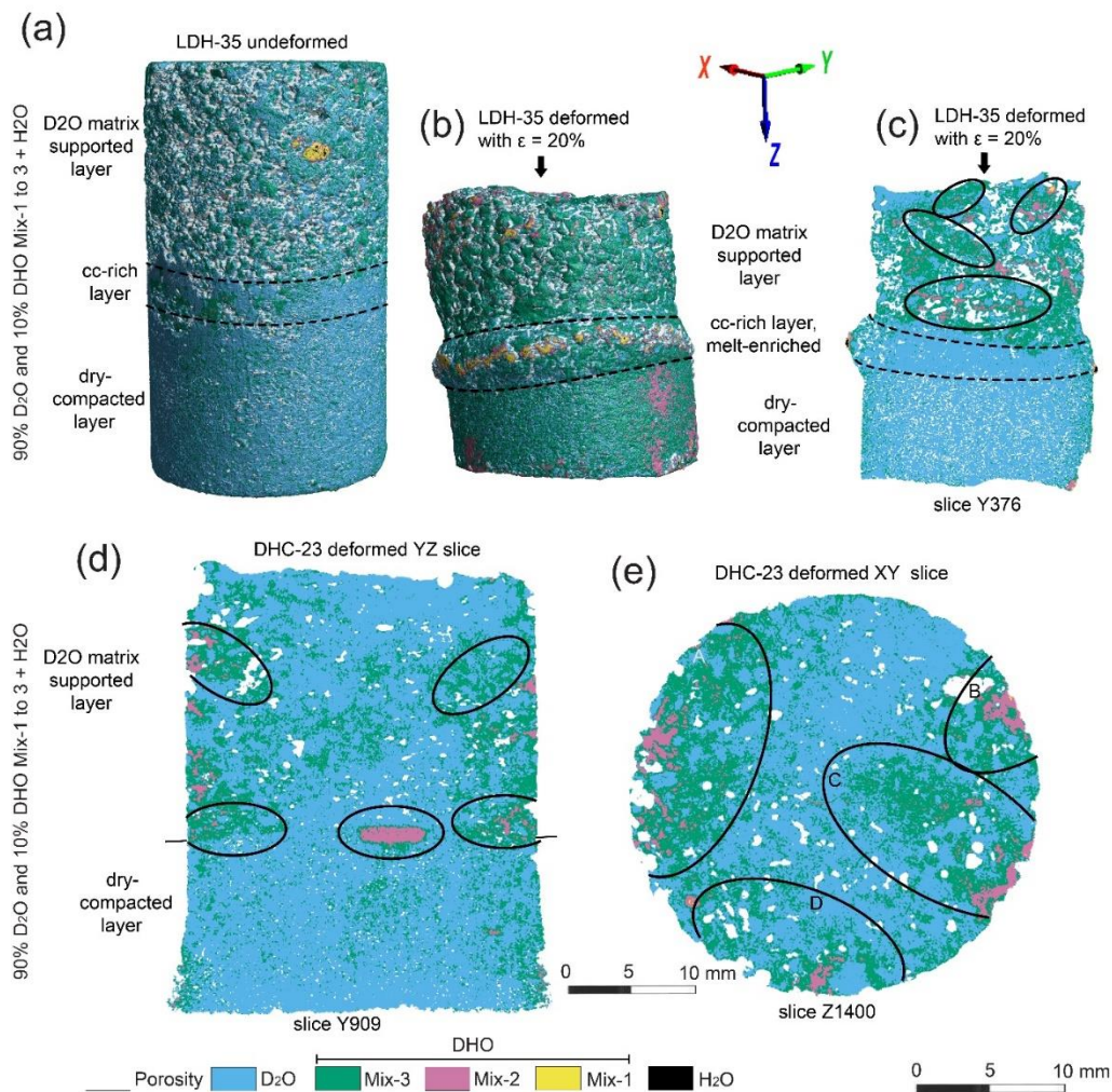
690 Figure 43: Visualization of melt distributions from tomographic images in LDH-35 and DHC-23. (a) 3D surface rendering of water and deuterium phases in the undeformed sample. The legend shows the transition of increasing proton exchange between deuterium-rich to hydrogen-rich ice. (b) Three-dimensional visualization of phase distributions on the outer surface of LDH-35def. The ellipse identifies a melt-enriched band of Mix-1 + Mix-2 along boundary of calcite(cc)- rich layer. The arrow shows the orientation of the compression axis during deformation. (c) segmentation along slice Y376 695 of deformed sample and ellipses show distribution of Mix-2 at oblique angles to the compression direction and on the boundary of the calcite-rich layer. (d) Two-dimensional segmentation along slice Y909 in DHC-23def with conjugate shear bands containing Mix-2 in the upper DH portion of the sample with horizontal concentrations at the interface with the dry- compacted ice; which forms the lower half of the sample. (e) XY slice of DHC-23def showing concentrations at A-D of Mix-2 adjacent to the outer edge of the deformed sample.
