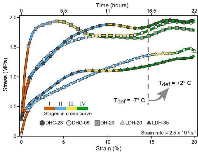
725 Figure 76: Nature of the stress-strain relationships. Over a temperature range of -7^{\circ}\text{C} during the first 14.6% shortening was followed by a temperature increase for a remaining 5.4% shortening. All experiments were undertaken at a constant displacement-rate ( 2.5 \times 10^{-6} \text{ s}^{-1} ). The maximum variation in stress for each curve is < 2 \text{ MPa} . After the increase in temperature there is a minor increase in stress, which we reconcile with an expansion of the aluminium of the rigid deforming indenter.
