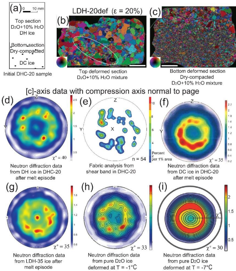
710 Figure 65: Microstructure and textural changes in samples deformed at a displacement-rate ( \dot{\epsilon} ) of 2.5 \times 10^{-6} \text{ s}^{-1} . (a) Sketch of initial DHC-20 sample with dimensions, width 24.7 mm, top section composed of DH ice (length 27.7 mm) and bottom section (length 17 mm) with DC ice. (b) Final microstructure of deformed top half of sample, colour of each pixel shows crystal [c]-axis direction perpendicular to the paper. The inset colour wheel image indicates [c]-axis directions in respect to vertical compression axis. The ellipse encloses a melt-enriched band identified by finer grain size at oblique angle to the compression direction. Bar scale = 5 mm. (c) Final microstructure of deformed bottom half of sample composed of dry compacted. (d-i) Pole figures showing a cluster of [c]-axes around the centre of the pole figure corresponding to compression axis (X). The polar angle \chi is the angle between the compression axis ( \chi = 0^\circ ) and the maximum contour for the [c]-axes. (e) Fabric analyser [c]-axis orientations from the elliptical area shown in (b) n = number of [c]-axes measured. Minima and maxima of density are indicated to the right of each pole figure.
