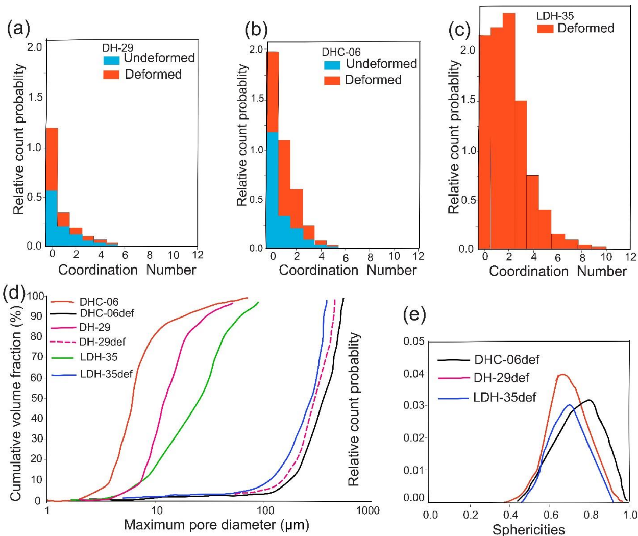
Figure 54: Plots comparing the pore network data of undeformed and deformed samples. (a-c) Probability distribution plots of coordination number of pores. We report the median values in Table 1. (d) Comparison between pore size distribution versus cumulative volume fraction (%) are plotted for both before and after deformation. The cumulative pore curves were determined to allow the geometrical pore size distribution to be interpreted in terms of micro- and macro-pore contributions to the total volume. (e) Distribution of sphericities in deformed samples. Pore sphericity is a volume-normalized, dimensionless measure of how close a particular component of the pore space is to an ideal sphere (with a sphere having a value of 1.0).
