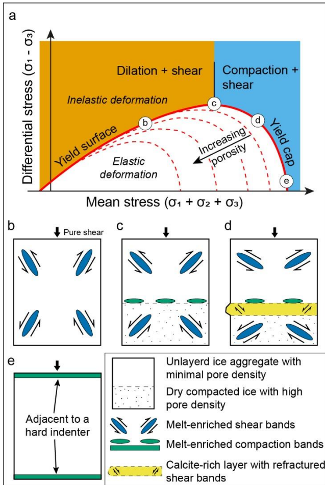
Figure 110: Schematic representation of a Mohr-Coulomb failure criterion with a capped yield surface with deformation modes identified in these experiments. (a) Nature of the yield surface or Mohr-Coulomb envelope and cap, which depends on porosity, grain size and the low (0.04–0.02) coefficient of friction for the ice (adapted from Reiweger et al., 2015, and Fossen et al., 2007). With decreasing cohesive strength and increasing porosity the shear failure envelope moves to a lower pore-fluid factor and differential stress. The various Two-dimensional modes of yielding identified in the deformed cylindrical samples (b – e) are shown with a vertical stress \sigma_1 . (b) Samples with no differences in material properties, dominated by conjugate shear bands. (c) Samples with weaker dry-compacted (DHC) and stronger water-rich ice (DH) with localized shear bands and a melt-enriched compaction band between the two ice types. (d) Triple layered samples with stress \sigma_1 normal to the interface between a calcite-rich layer, bounded by weaker material on either side. (e) Compaction bands developed at interface with indenting piston and no stress refraction occurs.
