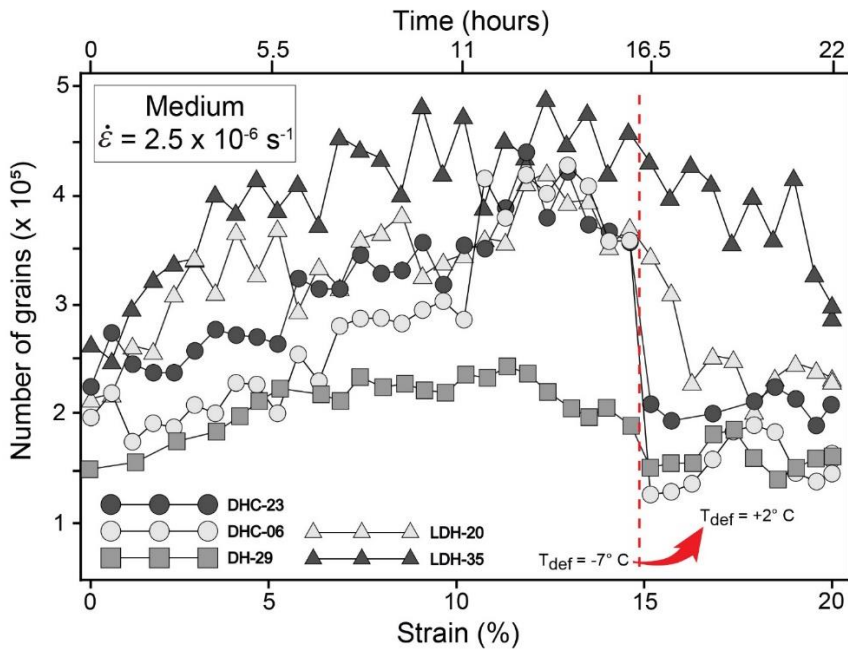
Figure 9: A grain number evaluation at different stages during deformation. The error in the grain number determination is approximately \pm 500 . The initial deformation temperature is -7^\circ\text{C} until 14.6% shortening, the temperature is then raised to +2^\circ\text{C} , which is accompanied by a decrease in grain numbers. At 20% shortening the temperature is decreased to -10^\circ\text{C} and any water phase freezes. The method of obtaining these grain numbers is described in Wilson et al. (2019).
