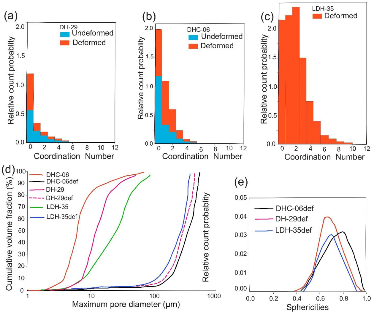
675 Figure 4: Plots comparing the pore network data of undeformed and deformed samples. (a-c) Probability distribution plots of coordination number of pores. We report the median values in Table 1. (d) Comparison between pore size distribution versus cumulative volume fraction (%) are plotted for both before and after deformation. The cumulative pore curves were determined to allow the geometrical pore size distribution to be interpreted in terms of micro- and macro-pore contributions to the total volume. (e) Distribution of sphericities in deformed samples. Pore sphericity is a volume- 680 normalized, dimensionless measure of how close a particular component of the pore space is to an ideal sphere (with a sphere having a value of 1.0).
