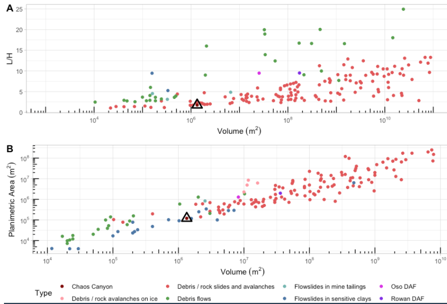
Figure 13. Landslide mobility indices. Panel A. The commonly used maximum landslide travel path (L) over landslide height (H) versus landslide volume. The Chaos Canyon landslide (marked as red dot with black triangle) has a low L/H \approx 1.8 and falls within the field of other debris slides, rock slides, and rock avalanches (Iverson et al., 2015). Panel B. The Chaos Canyon landslide inundated an area consistent with power law relationship between landslide area and volume discussed in Griswold and Iverson (2008).
