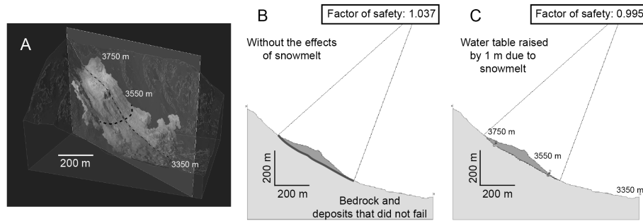
Figure 11. Output from limit equilibrium slope stability analysis. A) View of the pre-collapse topography in three-dimensions. The pre-collapse deposit is shown in gray. See appendix figure A6 for a color version. The thick dashed line represents the lower edge of the piece of the deposit that failed on June 28th, which is also shown in B and C. The thin dashed line shows the cross section also shown in B and C. B) Limit equilibrium analysis showing the global minimum slip surface and factor of safety for the simulated pre-slide deposit (purple) using the program Slide2. The failure surface (see the red line) is located at the transition between the purple body that moved during the collapse and the underlying material. C) Limit equilibrium analysis showing the global minimum slip surface and factor of safety for the simulated pre-collapse deposit with the effects of a water table 1 m above the contact between the pre-collapse deposit and the underlying bedrock.
