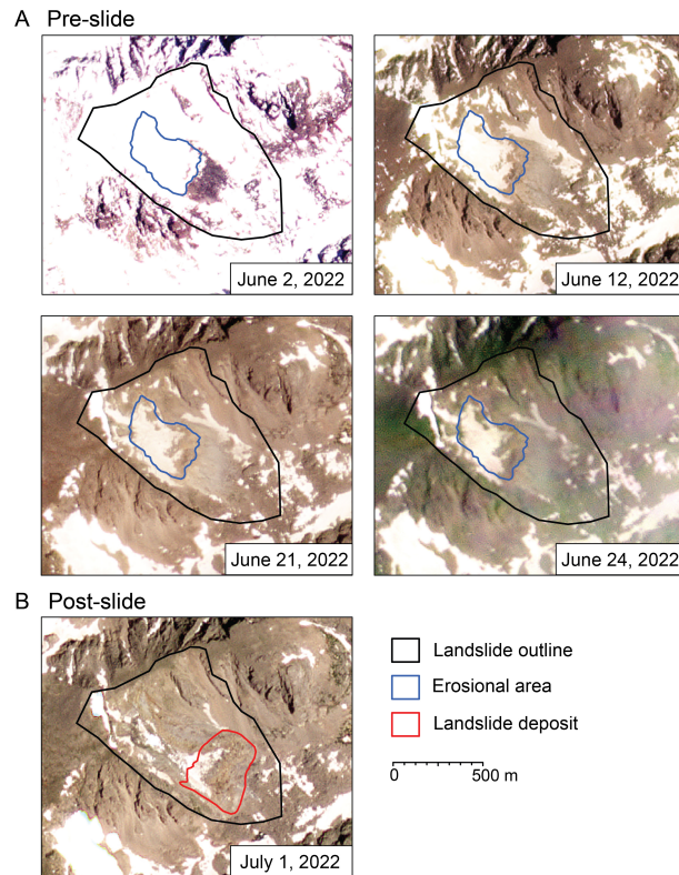
Figure 8. Planet imagery of upper Chaos Canyon in the days preceding the collapse. A Pre-collapse) Images from June 2nd, 12th, 21st, and 24th. Frames show decrease in snow coverage. Frames are also referenced in 7B. Satellite imagery further supports analysis that landslide collapse took place during a period of rapid snowmelt. B Post-collapse) The landslide deposit after the June 28th collapse is highlighted. Pieces of the permanent snowpatch have been translated with the landslide. Imagery thanks to Planet-Team (2017).
