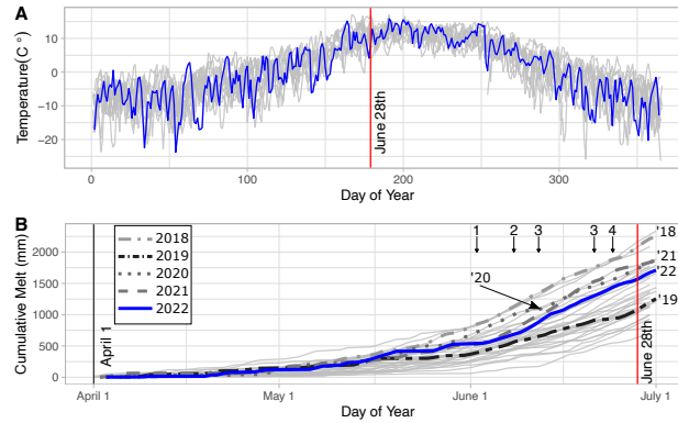
Figure 7. Climate analysis of the Chaos Canyon landslide. A) The mean daily temperature series estimated for ~3668 m, the elevation at the top of the slide. 2022 is highlighted blue. 1990 thru 2021 temperature series are gray lines. The collapse occurred on June 28th, 2022. B) The calculated cumulative snowmelt for the past 32 springs. 2022 is the blue line with 1990-2021 snowmelt seasons shown in gray. Inset numbers highlight dates for frames from Planet Imagery in Figure 8. The snowmelt curves for the previous four years (2018, 2019, 2020, and 2021) are also highlighted.
