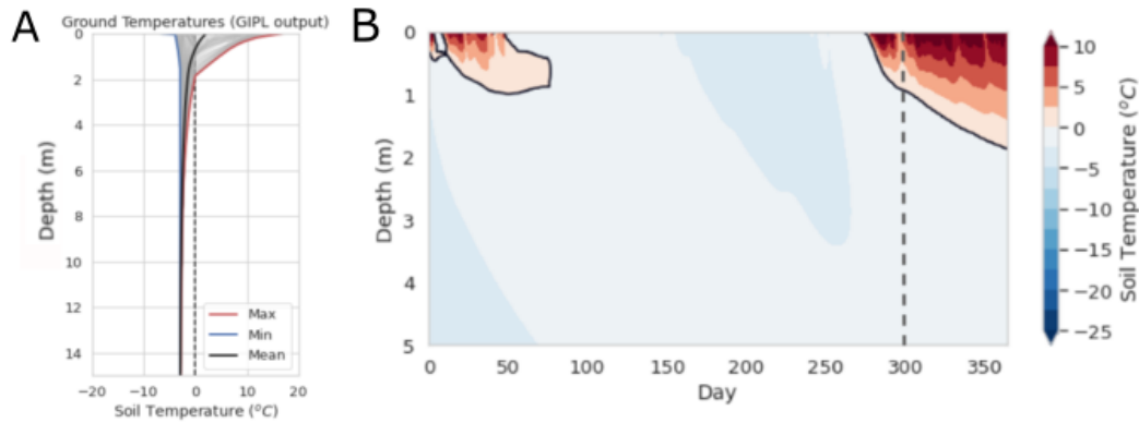
Figure 10. Simulation results of the combined snow and soil temperature model over the water year Oct 2020-Oct 2021 . Panel A. Shows soil temperature as a function of depth, with even maximum temperatures below \sim 2 m depth never reaching above 0^{\circ}\text{C} . Panel B. Shows soil temperatures with depth at the Chaos Canyon landslide across a single water year. This result mirrors the depth of the active layer shown in A. The dashed vertical line is June 28th. Note the days are based on zero as October 1, the start to the water year.
