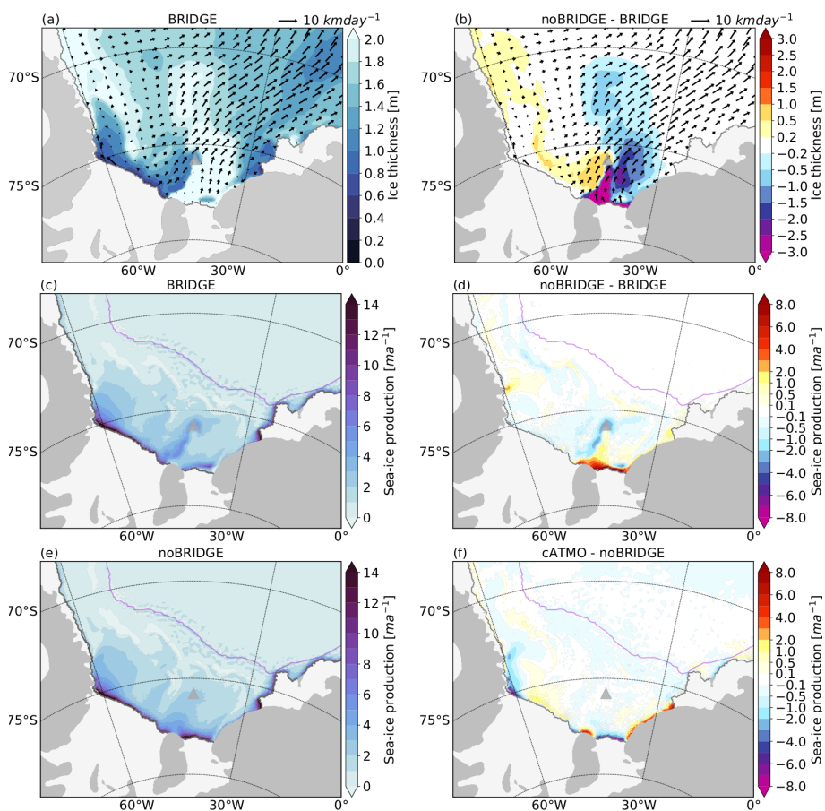
Figure 5. a) Sea-ice thickness and velocity from BRIDGE, and b) thickness difference between noBRIDGE and BRIDGE, with the velocity from noBRIDGE in August 2009. c) Mean sea-ice growth rates (2002–2017) from BRIDGE, and d) difference between noBRIDGE and BRIDGE. e) Mean sea-ice growth rates (2002–2017) from noBRIDGE, and f) difference between cATMO and noBRIDGE. The location of the grounded iceberg A23-A (2002–2017) is marked by a triangle. The 2500 m isobath is indicated by violet contour.
