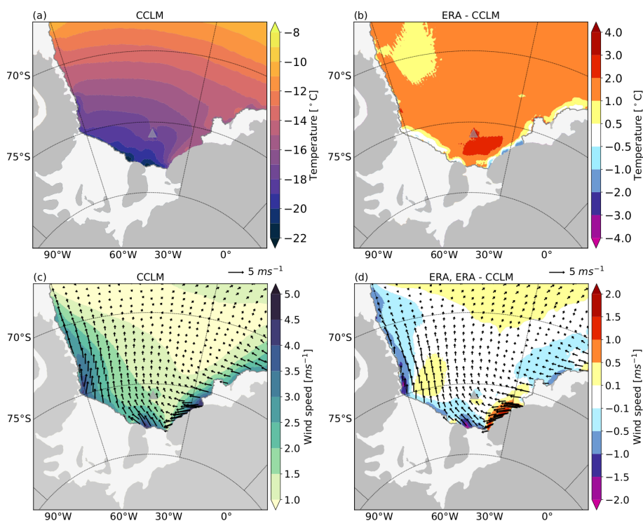
Figure 3. a) Mean air temperature (2002–2017) from CCLM, and b) air temperature difference between ERA-Interim and CCLM. c) Mean wind field (2002–2017) from CCLM and d) ERA-Interim, with wind speed difference between ERA-Interim and CCLM. Data is shown only over the ocean. Antarctic continent is drawn in grey, ice shelves are marked in light grey. The location of the grounded iceberg A23-A (2002–2017) is marked by a triangle.
