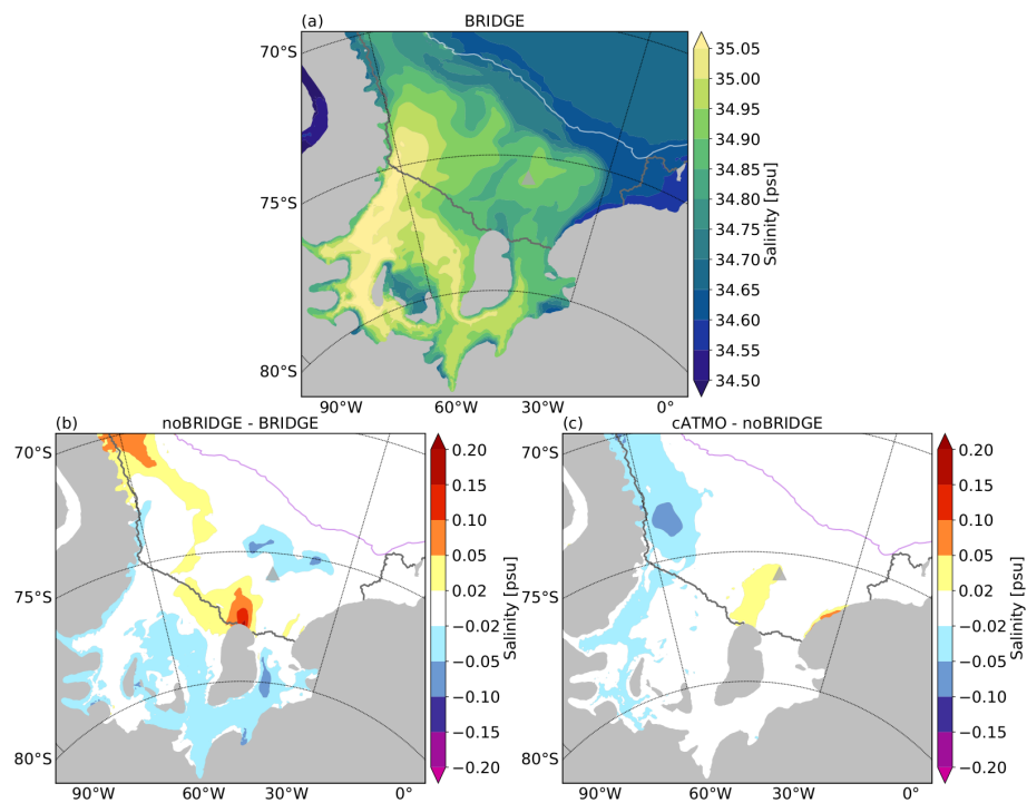
Figure 7. a) Mean bottom salinity (2002–2017) from BRIDGE. The ice shelf edge is indicated by gray contour, and the 2500 m isobath is marked by white contour. Difference in the mean bottom salinity (2002–2017) between b) noBRIDGE and BRIDGE, and c) cATMO and noBRIDGE. The ice shelf edge is indicated by gray contour, and the 2500 m isobath is marked by violet contour. The location of the grounded iceberg A23-A (2002–2017) is marked by a triangle in all panels.
