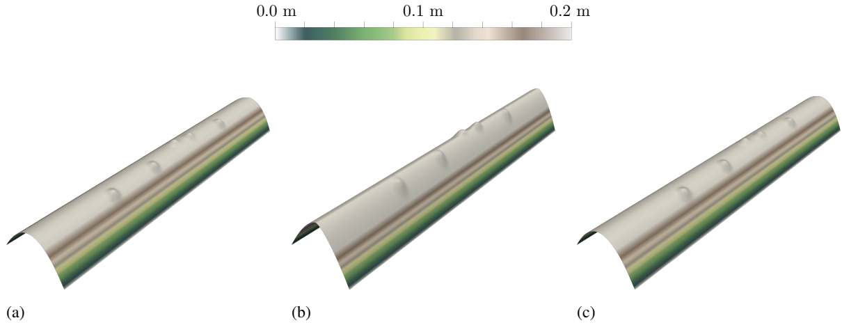
Figure 5. Sediment height h_s^{ex} of the analytic solution for the case k_g = 5 \text{ km}^2 \cdot \text{My}^{-1} and k_w = 1 \text{ km}^2 \cdot \text{My}^{-1} . a: r_s = 1 , p_s = 0 , b: r_s = 3/2 , p_s = 1 , c: r_s = 2 , p_s = 0
