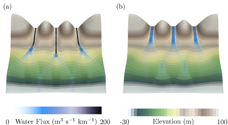
Figure 23. Comparison of models (4) and (23) on the “three rivers” test case for \alpha = 2.2 km and \Delta_{xy} = 2 km
