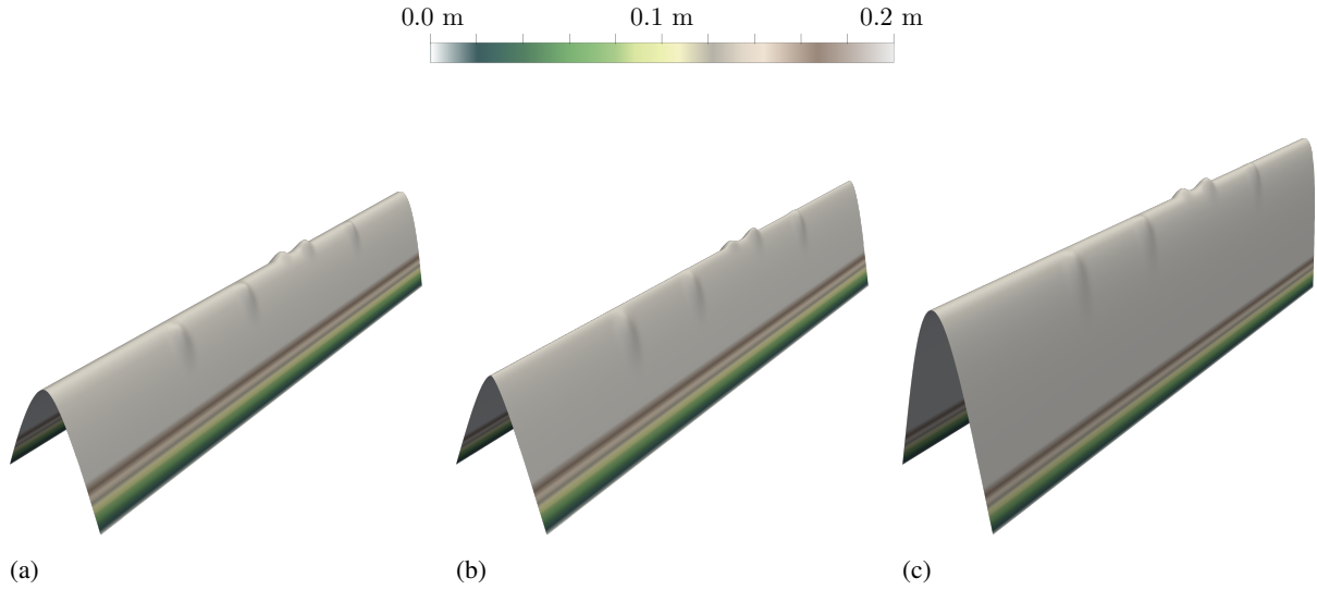
Figure 7. Sediment height h_s^{ex} of the analytic solution for the case k_g = 1 \text{ km}^2 \cdot \text{My}^{-1} and k_w = 5 \text{ km}^2 \cdot \text{My}^{-1} . a: r_s = 1, p_s = 0 , b: r_s = 3/2, p_s = 1 , c: r_s = 2, p_s = 0
