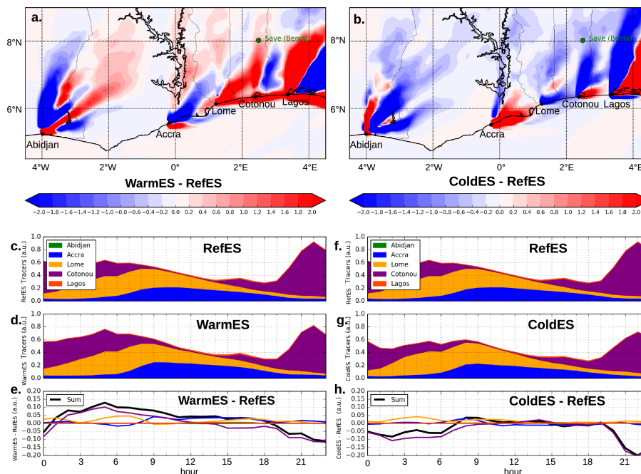
Figure 9. Upper panels: Difference maps of urban tracer transport modelled with a. WarmES - RefES and with b. ColdES - RefES using a constant release of urban tracers from five major coastal cities of the Gulf of Guinea (black dots): Abidjan (Ivory Coast), Accra (Ghana), Lomé (Togo), Cotonou (Benin) and Lagos (Nigeria), taking into account the city population (see Deroubaix et al. 2019 for details). Lower panels: hourly diurnal cycle of the urban tracer concentrations at the DACCIWA super site of Savè in Benin (green dot on upper panels) averaged over the period from June 25th to July 8th modelled with c. RefES (also in f.), d. WarmES or g. ColdES. Differences: e. WarmES - RefES and h. ColdES - RefES. Note that the green colors associated with Abidjan are not visible because the pollution of Abidjan (studied by the tracers emitted in Abidjan) does not reach the city of Savè for any of the three ensembles.
