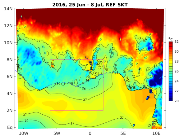
Figure 2. Jun 25th to Jul 8th, 2016: skin temperature (SKT in °C, shading) from the Reference ensemble simulation (RefES). The red frame highlights the sub-region of 6°W-2°E/2°N-8°N shown in Figures 4, 7, 8 and 10. The black contours represent the isotherms of 26°C and 27°C.
