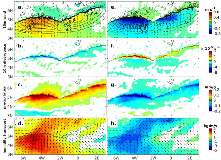
Figure 6. June 25th to July 8th, 2016: differences between WarmES and RefES simulations (left) and between ColdES and RefES simulations (right). a.,e.: 10m-wind (speed in shading, \text{m}\cdot\text{s}^{-1} ) and surface temperature (black contours, intervals of 0.1^\circ\text{C} ). b.,f.: divergence of 10m-wind (shading, \text{s}^{-1} ). c., g.: total precipitation ( \text{mm}/\text{h} ). d., h.: humidity transport integrated between 1000 and 850 hPa ( \text{kg}\cdot\text{m}^{-1}\cdot\text{s}^{-1} ). Only difference values passing a two sampled t-test at the 5 % confidence level are shaded.
