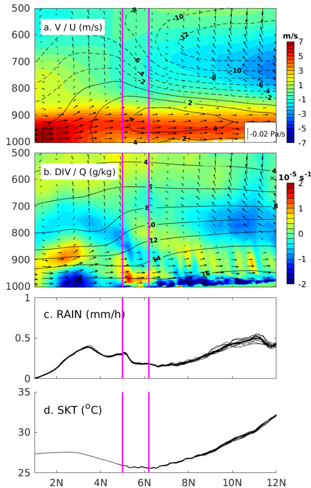
Figure 4. Jun 25th to Jul 8th, 2016, RefES, within the region 6^{\circ}\text{W} - 2^{\circ}\text{E} : a. meridional and vertical velocity (arrows), meridional velocity (shading) and zonal velocity (black contours, plain for positive, dashed for negative, intervals of 1 \text{ m}\cdot\text{s}^{-1} , null velocity in heavy black), b. meridional and vertical velocity (arrows), horizontal divergence (shading) and specific humidity (black contours, \text{g}/\text{kg} ), c. precipitation and d. surface temperature profiles (black profiles, average in thick line). The vertical pink lines frame the coastline between 6^{\circ}\text{W} and 2^{\circ}\text{E} . Vertical scale for arrows indicated in a.
