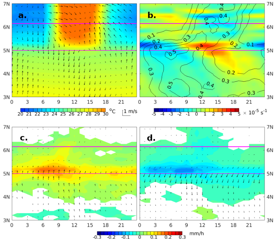
Figure 8. June 25th to July 8th, 2016: time-latitude diagram (diurnal cycle) within the region 6^{\circ}\text{W}-2^{\circ}\text{E} . In RefES: a. diurnal cycle of SKT (shading) and diurnal anomalies of 10-m wind (arrows), b. diurnal anomalies of 10-m wind divergence (shading) and diurnal cycle of precipitation (black contours, intervals of 0.1 mm/h). Differences between WarmES (c.) or ColdES (d.) and RefES of diurnal cycles of precipitation (shading) and 10-m surface wind (arrows). Only precipitation and velocity anomalies passing a two sampled t-test at the 5 % confidence level are plotted. The horizontal scale of the vectors represents a velocity, despite being aligned in the direction of time.
