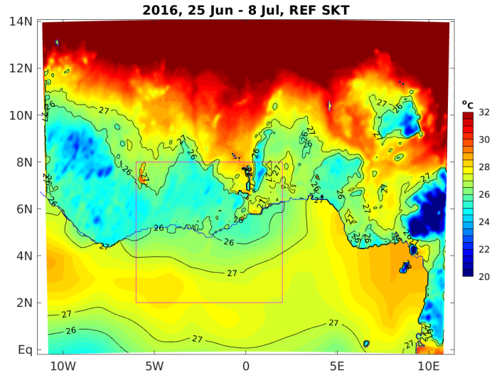
Figure 2. Jun 25th to Jul 8th, 2016: skin temperature (SKT in °C, shading) from the Reference ensemble simulation (RefES). The red frame highlights the sub-region of 6°W-2°E/2°N-8°N shown in Figures 4, 7, 8 and 10. The black contours represent the isotherms of 26°C and 27°C.
