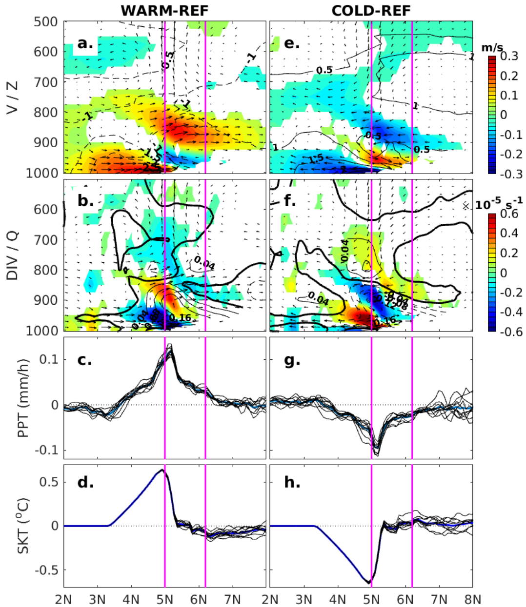
Figure 7. June 25th to July 8th, 2016: differences between WarmES and RefES (left column) and between ColdES and RefES (right column) within the region 6°W-2°E. a.,e.: meridional-vertical circulation (black arrows, meridional velocity (shading) and geopotential height anomalies (black contours, dashed for negative, plain for positive, intervals of 0.2 m). e., f.: meridional-vertical circulation (black arrows), horizontal divergence (shading) and specific humidity (black contours, plain for positive, dashed for negative, intervals of 0.4 g/kg). c.,g.: precipitation (blue, mm/h). d.,h.: SKT (blue, °C). In c.-h., 10 time series are shown (black) out of 100 possible time series from WarmES minus RefES or ColdES minus RefES, roughly indicating their dispersion. The coast latitude is framed by vertical pink lines. Only difference values of meridional velocity and horizontal divergence that pass a two sampled t-test at the 5 % confidence level are shown as shaded areas.
