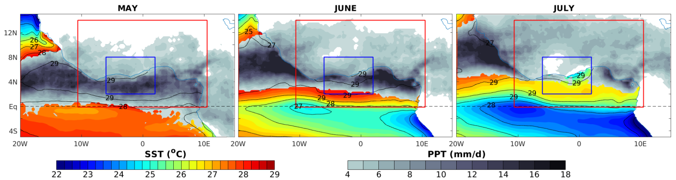
Figure 1. Observations from May (left), June (center) and July (right) 2008-2017: sea surface temperature (SST, black contours with 1^{\circ}\text{C} intervals and red-green-blue shading) and Tropical Rainfall Measuring Mission (TRMM) precipitation exceeding 4\text{ mm/d} (gray shading). The red and blue frames show the simulation coverage and the sub-region under scrutiny 6^{\circ}\text{W}-2^{\circ}\text{E} / 2^{\circ}\text{N}-8^{\circ}\text{N} .
