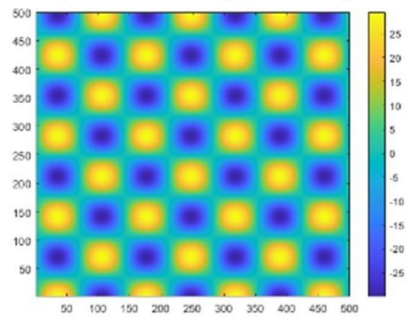
example wind field from two interfering modes ("checkers pattern")
