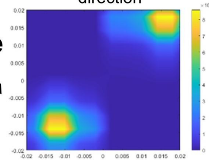
2D Fourier spectrum filtered by propagation direction
