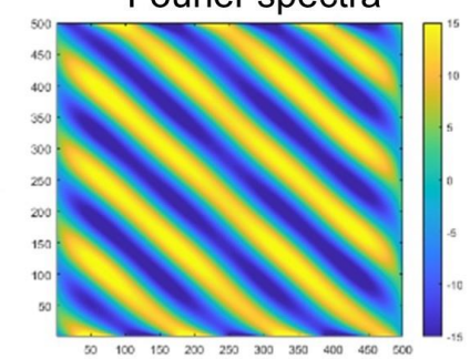
wind fields from retransformed filtered Fourier spectra
