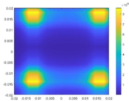
2D Fourier spectrum
