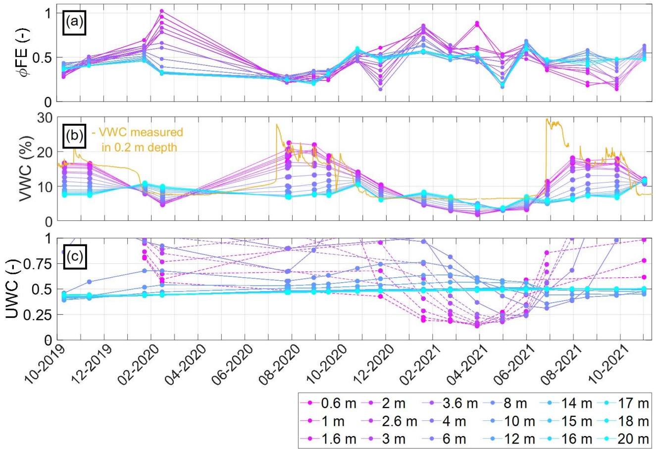
Figure 11: Temporal changes in (a) \phi FE , (b) measured and estimated volumetric water content (VWC) and (c) unfrozen water content (UWC) at the borehole location at various depths (0.6 - 20 m). The cementation exponent was estimated for a given measurement of VWC (baseline date in October 2019) within the debris layer ( \Phi = 0.6 ). Porosity, fluid resistivity ( \rho_\omega = 220 \Omega_m ), cementation exponent ( m = 2.2 ) and saturation exponent ( n = 2 ) were kept constant over time and VWC was calculated using Equations 7, 9 and 10. To obtain the UWC (Equ. 12), the parameter b was fitted for each depth according to the exponential behavior of the corresponding resistivity data at 0.5 Hz using Equ. 11 with \rho_0 = 9.331 \Omega_m and T_F = -0.17^\circ C .
