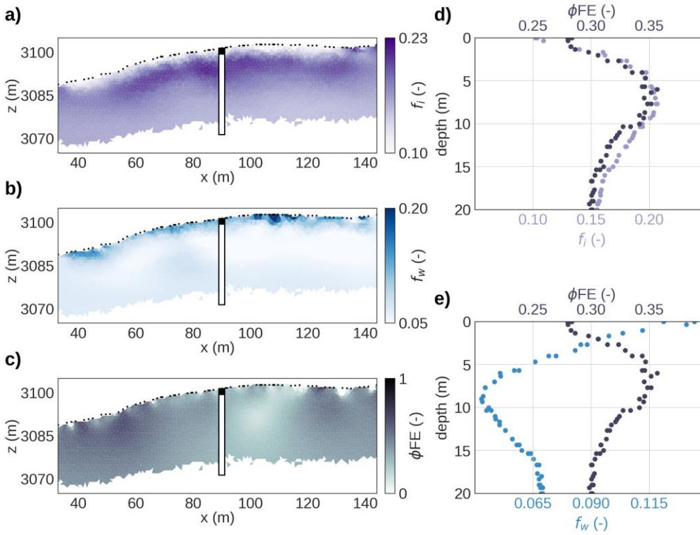
530 Figure 8: (a-c) Calculated \phi_{FE} for the phase of the complex resistivity imaging results between 75 Hz and 0.5 Hz and visualized for the whole tomogram for the SIP monitoring profile (between profile meter 33 and 141) and comparison with water and ice content estimates from PJI results. (d) Vertical 1D logs of the \phi_{FE} and the ice content and (e) water content extracted at the borehole location from 2D sections.
