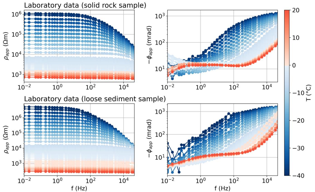
845 Figure B1: Broadband SIP laboratory measurements on a solid rock sample and a loose sediment sample collected at the site close to the monitoring profile. Apparent resistivity and phase values are shown in a frequency range between 10 mHz and 45 kHz during controlled freeze-thaw cycles (+20°C to -40°C to +20°C).
