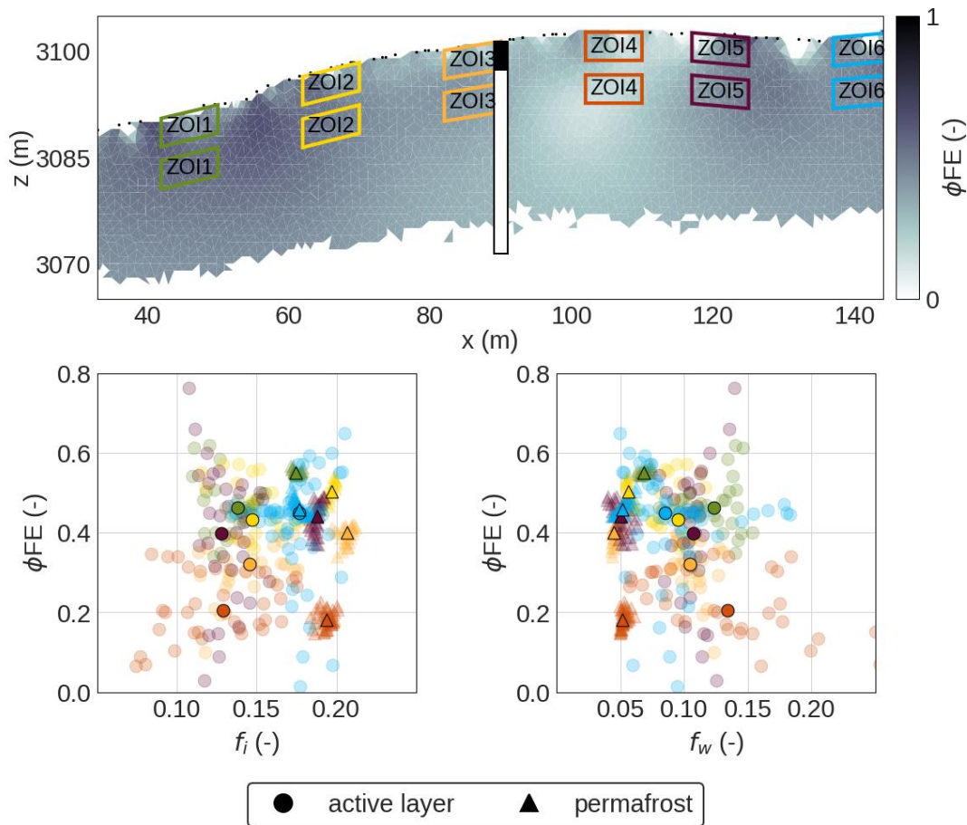
Figure 14: Correlation between PJI-derived ice and water content estimates and the phase frequency effect for selected zones of interest (ZOIs) within the active layer and the permafrost body along the SIP monitoring profile.
