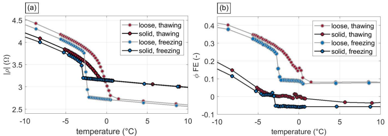
Figure 7: Temperature dependence of a) the impedance magnitude (at 0.5 Hz) and b) for the \phi FE (calculated between 70 and 0.5 Hz) measured on solid rock (solid) and loose sediment (loose) samples during freezing (blue) and thawing (red) in the laboratory (same experiments as shown in Fig. 6).
