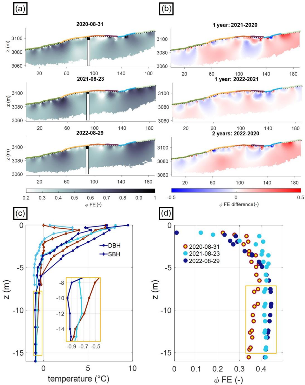
Figure 13: (a) The phase frequency effect ( \phi FE ) and (b) the difference in \phi FE (i.e., \phi FE difference = \phi FE Aug22 – \phi FE Aug20) is visualized between August 2020 and August 2022 for the entire imaging plane (borehole position and thaw depths are highlighted). (c) Borehole temperature data of SBH and DBH and the (d) \phi FE extracted at the borehole position for the dates of the respective SIP measurements.
