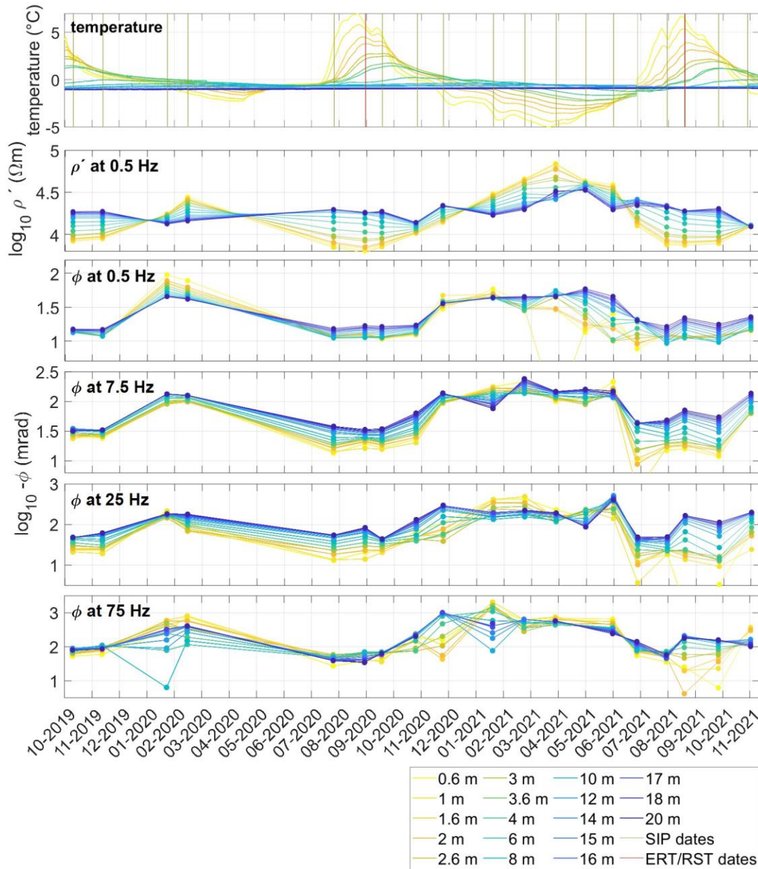
550 Figure 9: Comparison of borehole temperatures with complex resistivity results at different frequencies (0.5, 7.5, 25, 75 Hz) extracted at borehole position in the borehole temperature sensor depths.
