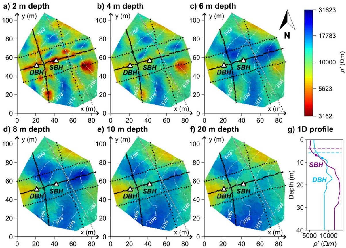
415 Figure 4: Spatial characterization of the Cime Bianche monitoring site based on the 3D electrical resistivity inversion results from five profiles collected in September 2020 (dotted black lines). Panels a)-f) represent slices parallel to the surface in six different depths. The borehole location of the SBH and the DBH are marked and white contour lines represent the surface elevation. The coordinates of the SIP monitoring profile are shown in addition (dotted grey line), but these data were not used for inversion due to a differing measurement date (October 2020). Panel g) represents the resistivity-depth profiles at the location of the two boreholes 420 with the measured thaw depth (dashed lines) and the inflection point in the resistivity data (dots).
