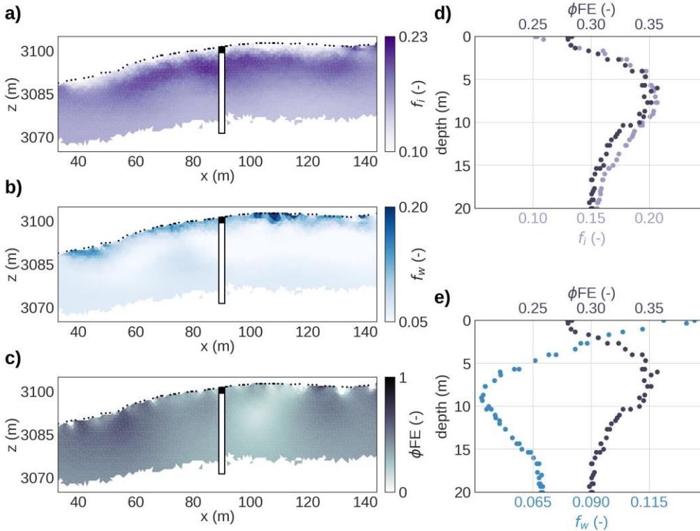
Figure 8: (a-c) Calculated \phi FE for the phase of the complex resistivity imaging results between 75 Hz and 0.5 Hz and visualized for the whole tomogram for the SIP monitoring profile (between profile meter 33 and 141) and comparison with water and ice content estimates from PJI results. (d) Vertical 1D logs of the \phi FE and the ice content and (e) water content extracted at the borehole location from 2D sections .
