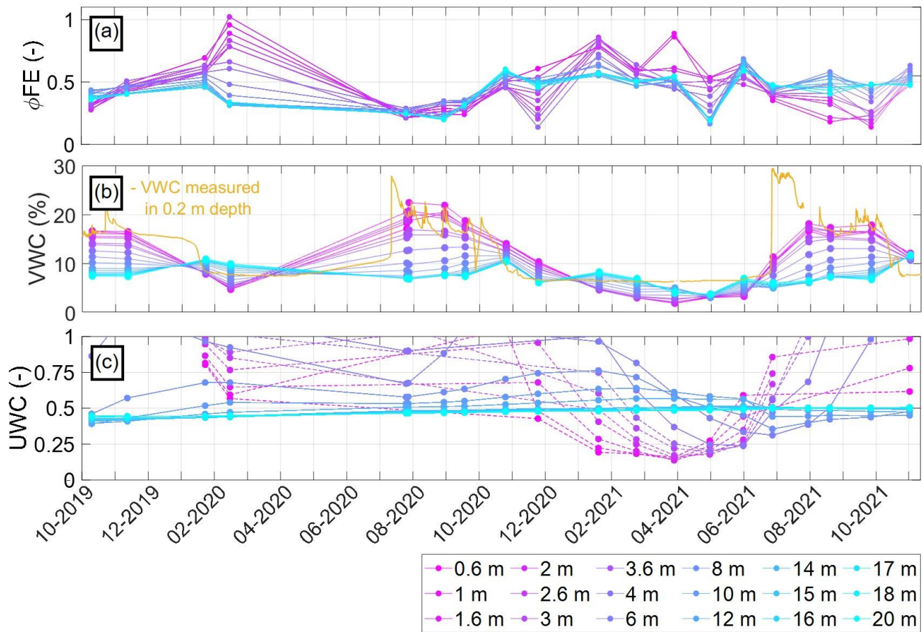
Figure 12: Temporal changes in (a) \phi FE , (b) measured and estimated volumetric water content (VWC) and (c) unfrozen water content (UWC) at the borehole location at various depths (0.6 - 20 m). The cementation exponent was estimated for a given measurement of VWC (baseline date in October 2019) within the debris layer ( \Phi = 0.6 ). Porosity, fluid resistivity ( \rho_{\omega} = 220 \Omega_m ), cementation exponent ( m = 2.2 ) and saturation exponent ( n = 2 ) were kept constant over time and VWC was calculated using Equations 7, 9 and 10. To obtain the UWC (Equ. 12), the parameter b was fitted for each depth according to the exponential behavior of the corresponding resistivity data at 0.5 Hz using Equ. 11 with \rho_0 = 9.331 \Omega_m and T_F = -0.17^\circ C .
