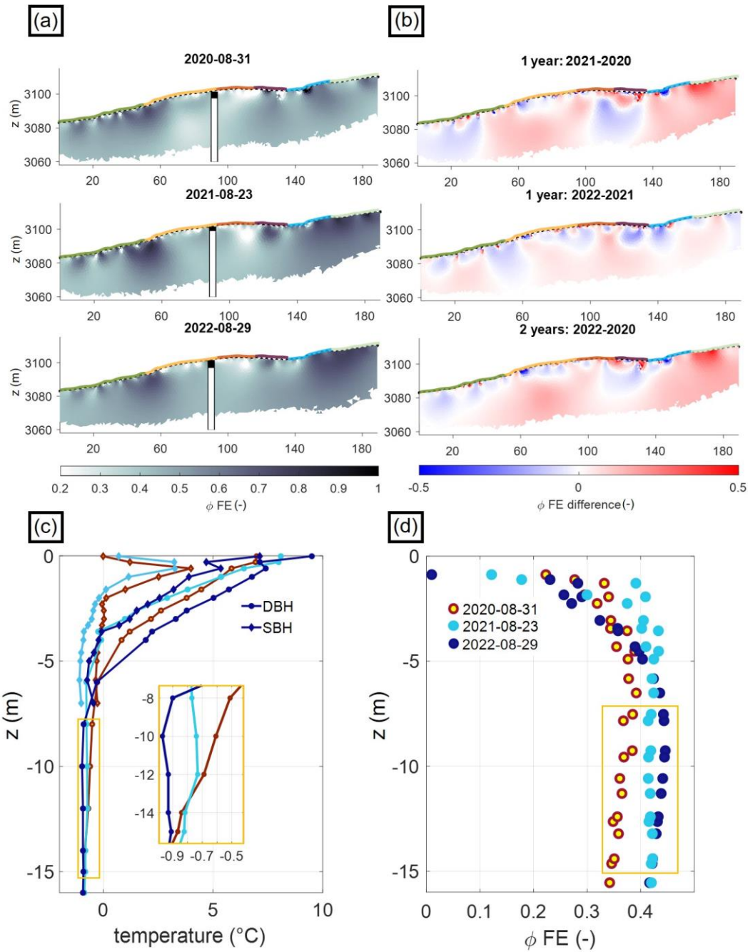
Figure 13: (a) The phase frequency effect ( \phi FE ) and (b) the difference in \phi FE (i.e., \phi FE difference = \phi FE_{\text{Aug22}} - \phi FE_{\text{Aug20}} ) is visualized between August 2020 and August 2022 for the entire imaging plane (borehole position and thaw depths are highlighted). (c) Borehole temperature data of SBH and DBH and the (d) \phi FE extracted at the borehole position for the dates of the respective SIP measurements.
