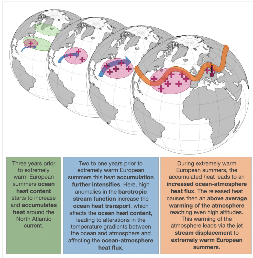
Figure 5. New Figure Schematic sketch illustrating the described mechanism. The blue arrows illustrate the increasing North Atlantic current; the pink crosses indicate the increase of ocean heat content and accumulation of heat; and the orange belt illustrates the jet stream. The thermometer at lag 0 illustrates the extremely warm European summers.
