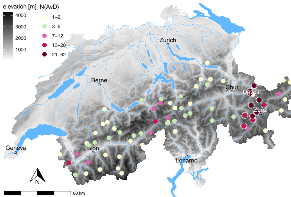
Figure 2. Map of Switzerland showing the location of the automated weather stations (dots). The coloring indicates the number of avalanche days (AvD) per station [.. 22 ], summed up over all aspects and over the three winter seasons 2019/2020 - 2021/2022. Stations in the Davos-Zuoz area, which had N \geq 13 AvDs per station were combined in a subset «Davos-Zuoz» (marked with white circles), all other stations as «elsewhere». For illustration purposes, the major rivers and lakes are shown in blue, and the elevation in grey. (Digital elevation model - source: Federal Office of Topography swisstopo)
