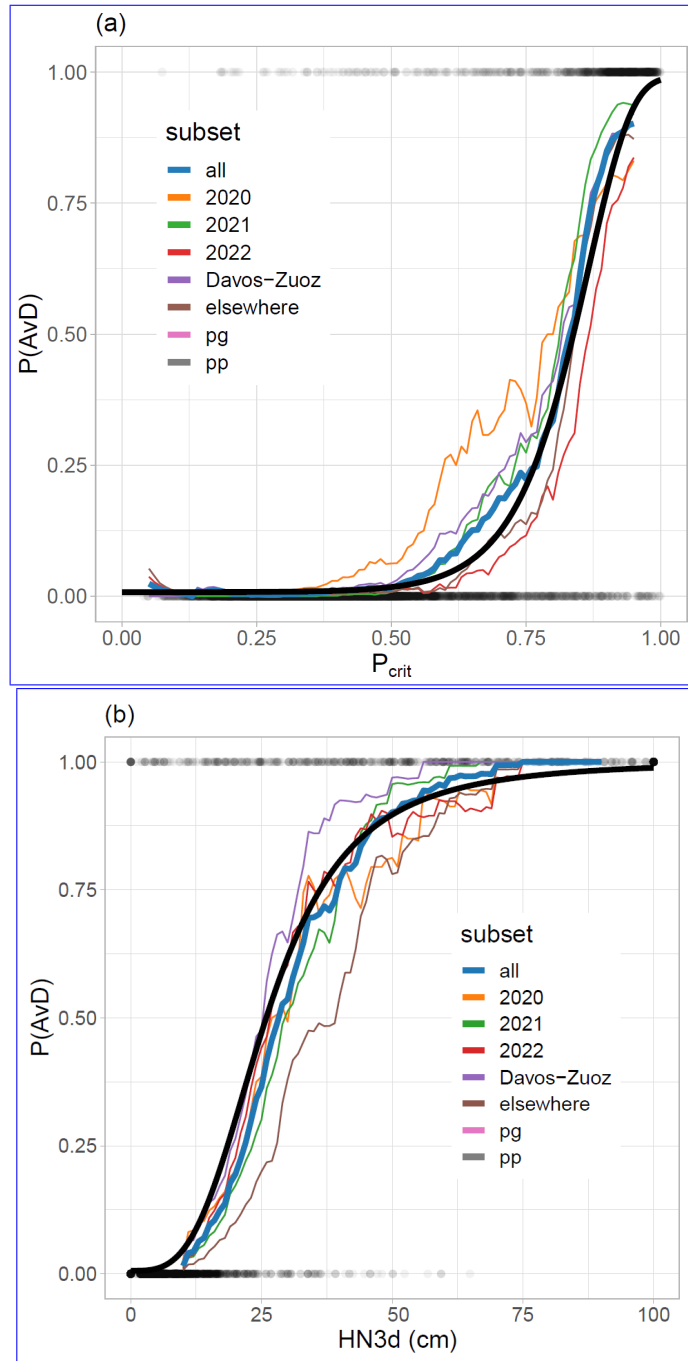
Figure 5. Probability that a day is an avalanche day ( P(\text{AvD}) ) as a function of (a) P_{\text{crit}} and (b) \text{HN3d} for the data subsets shown in Table 3. The subsets are binned with bin-size being 0.1 in (a) and 10 cm in (b). The best-fitting function describing all data is shown in black.
