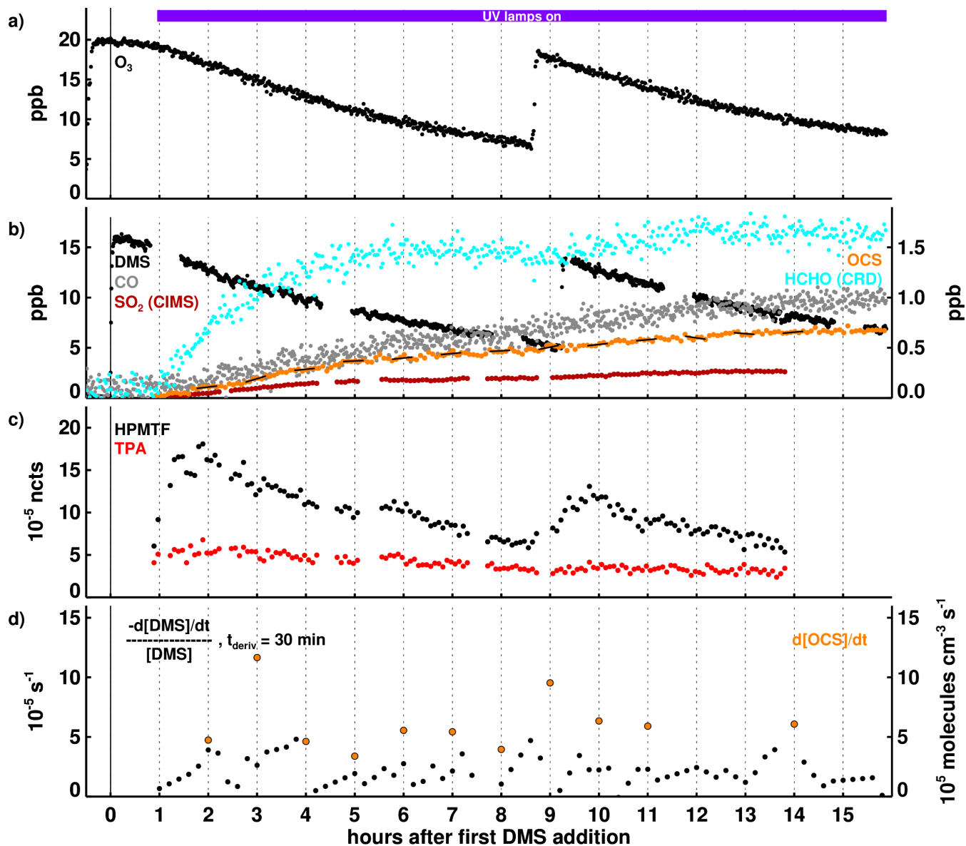
590 Figure 2 Time series of selected parameters in Experiment II, with time in hours after the first DMS injection and the period with the UV lamps turned on indicated by the coloured bar on the top of panel a). In panels a) and b), mixing ratios for trace gases are shown with the position of the labels indicating which axis refers to which species. In panel c), HPMTF and TPA are shown as normalized counts (see Section 2.3). In panel d), the first order DMS decay rate is determined for each individual point by a linear least squares fit of the DMS concentration data within \pm 15 minutes of this point. OCS production rates given in panel d) are calculated by linear least squares fitting of the OCS concentration data marked with the black lines in panel b), each encompassing 30 minutes of data (the time periods were chosen to 595 avoid data gaps and periods where the production rate changed significantly within 30 minutes). Both DMS loss and OCS formation rates shown are corrected for the loss induced by the replenishment flow in the SAPHIR.
