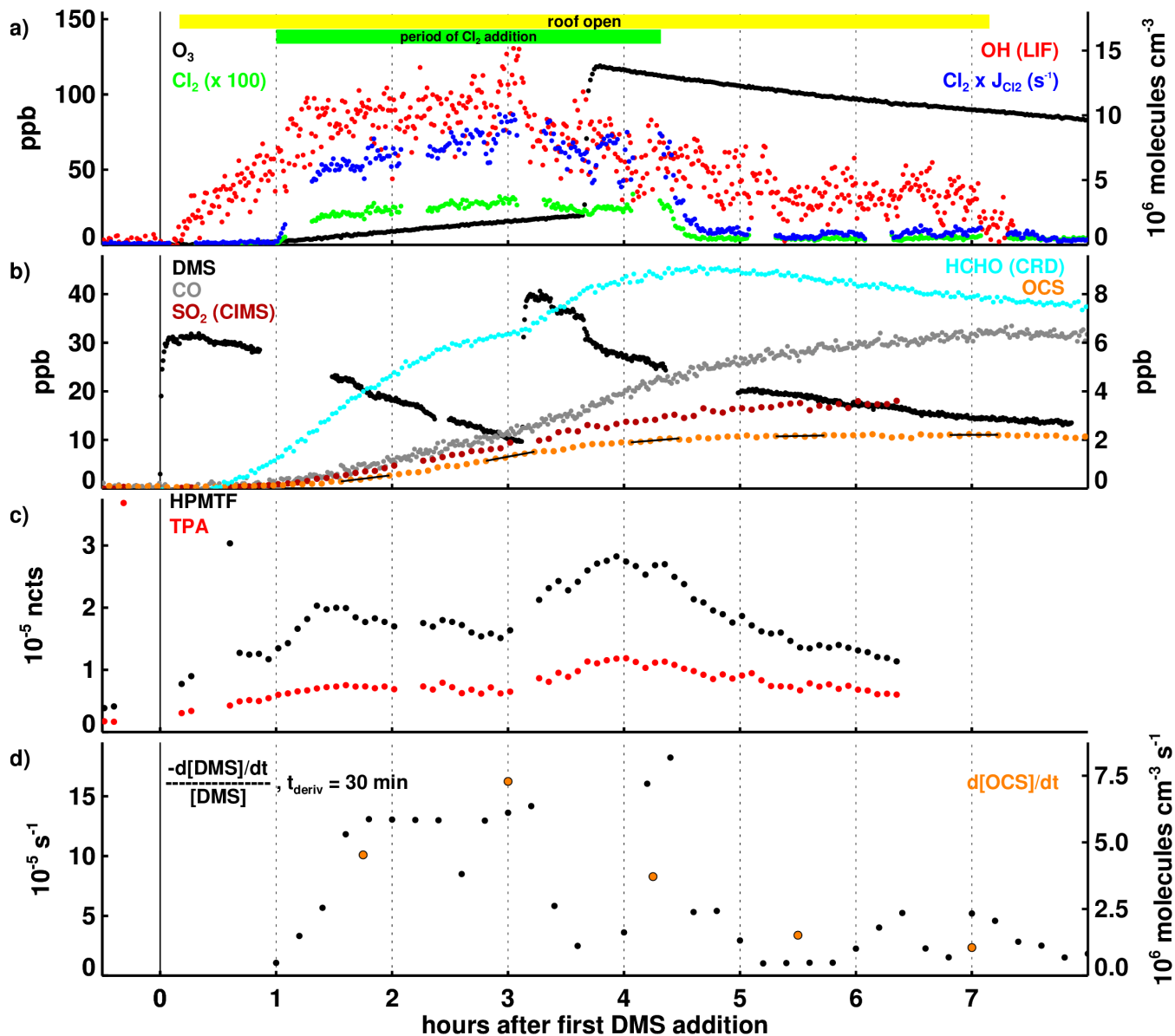
600 Figure 3 Time series of selected parameters in Experiment III, with time in hours after the first DMS injection and the periods of daylight irradiation and continuous \text{Cl}_2 injection indicated by the coloured bars on the top of panel a). In panels a) and b), mixing ratios for trace gases, the OH concentration and the product of the \text{Cl}_2 concentration and its photolysis rate are shown with the position of the labels indicating which axis refers to which species. In panel c), HPMTF and TPA are shown as normalized counts (see Section 2.3). In panel d), the first order DMS decay rate is determined for each individual point by a linear least squares fit of the DMS concentration data within \pm 15 minutes of this point. OCS production rates given in panel d) are calculated by linear least squares fitting of the OCS concentration data marked with the black lines in panel b), each encompassing 30 minutes of data (the time periods were chosen to avoid data gaps and periods where the production rate changed significantly within 30 minutes). Both DMS loss and OCS formation rates shown are corrected for the loss induced by the replenishment flow in the SAPHIR. 605
