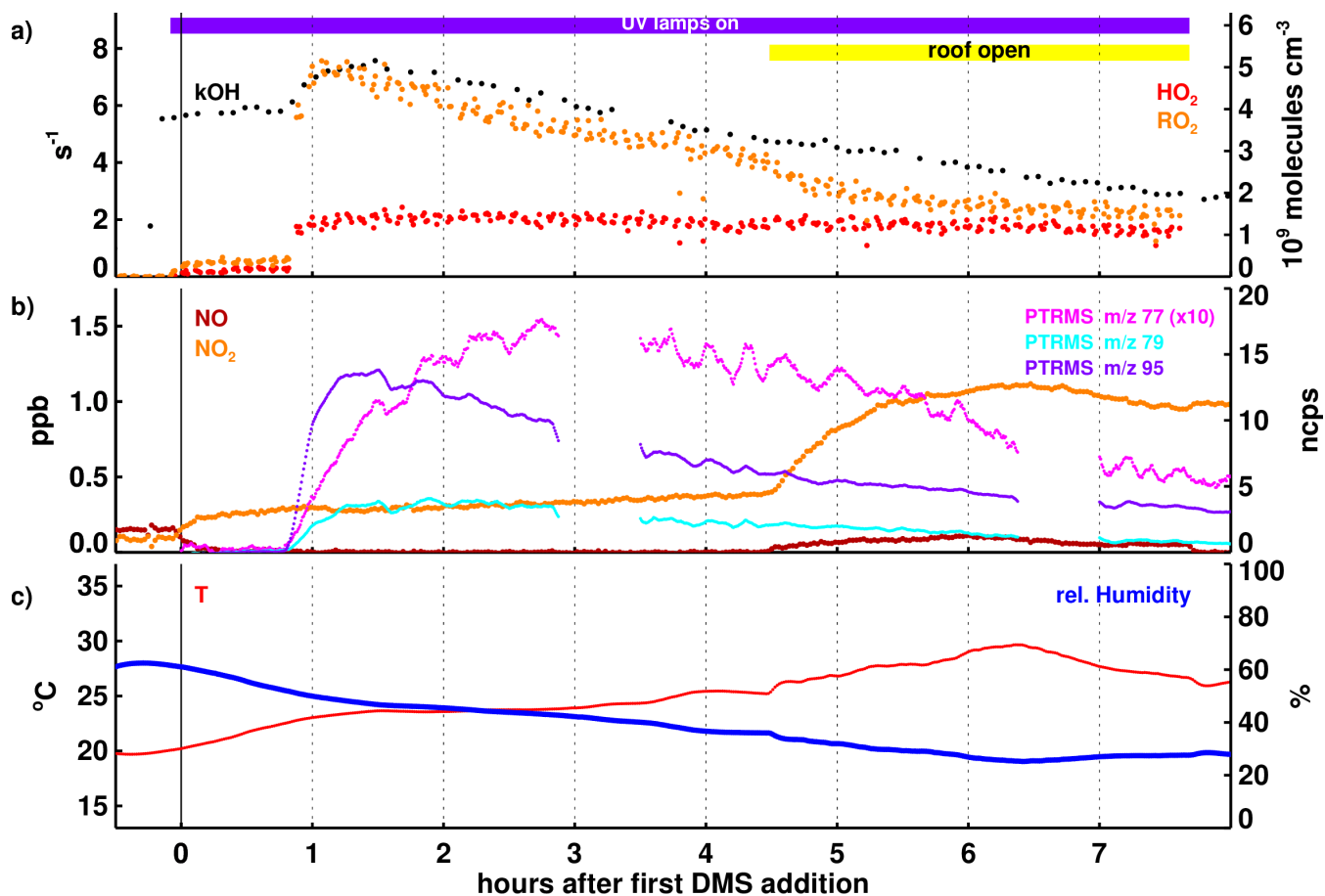
670 Figure S4 Additional parameters in Experiment IV, with time in hours after the first DMS injection and the periods with the UV lamps turned on and the roof being open indicated by the coloured bar on the top of panel a. In panel a) k_{OH} and radical concentrations are shown with the position of the labels indicating which axis refers to which species. In panel b), NO and NO_2 mixing ratios are given, together with raw PTRMS signals at m/z ratios that are potentially related to relevant products and intermediates ( m/z 77: CH_3SCHO ; m/z 79: DMSO ; m/z 95: DMSO_2 or CH_3SCH_2OOH ; see Section 2.3 of the article). In panel c), temperature and humidity in the SAPHIR chamber are shown.
