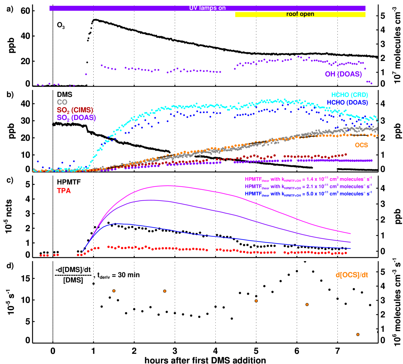
Figure 4 Time series of selected parameters in Experiment IV, with time in hours after the first DMS injection and the periods with the UV lamps turned on and the SAPHIR daylight shutters being open indicated by the coloured bars on the top of panel a). In panels a) and b), mixing ratios for trace gases and the OH concentration are shown with the position of the labels indicating which axis refers to which species. In panel c), observed HPMTF and TPA are shown as normalized counts (left side axis) and estimated (see text in Section 3.4) HPMTF mixing ratios (right side axis) are shown for k_{\text{HPMTF}+\text{OH}} = 1.4 \times 10^{-11} \text{ cm}^3 \text{ molecules}^{-1} \text{ s}^{-1} (Jernigan et al., 2022, magenta), k_{\text{HPMTF}+\text{OH}} = 2.1 \times 10^{-11} \text{ cm}^3 \text{ molecules}^{-1} \text{ s}^{-1} (Ye et al., 2022, purple) and k_{\text{HPMTF}+\text{OH}} = 5 \times 10^{-11} \text{ cm}^3 \text{ molecules}^{-1} \text{ s}^{-1} (blue.) In panel d), the first order DMS decay rate is determined for each individual point by a linear least squares fit of the DMS concentration data within \pm 15 minutes of this point. OCS production rates given in panel d) are calculated by linear least squares fitting of the OCS concentration data marked with the black lines in panel b), each encompassing 30 minutes of data (the time periods were chosen to avoid data gaps and periods where the production rate changed significantly within 30 minutes). Both DMS loss and OCS formation rates shown are corrected for the loss induced by the replenishment flow in the SAPHIR.
