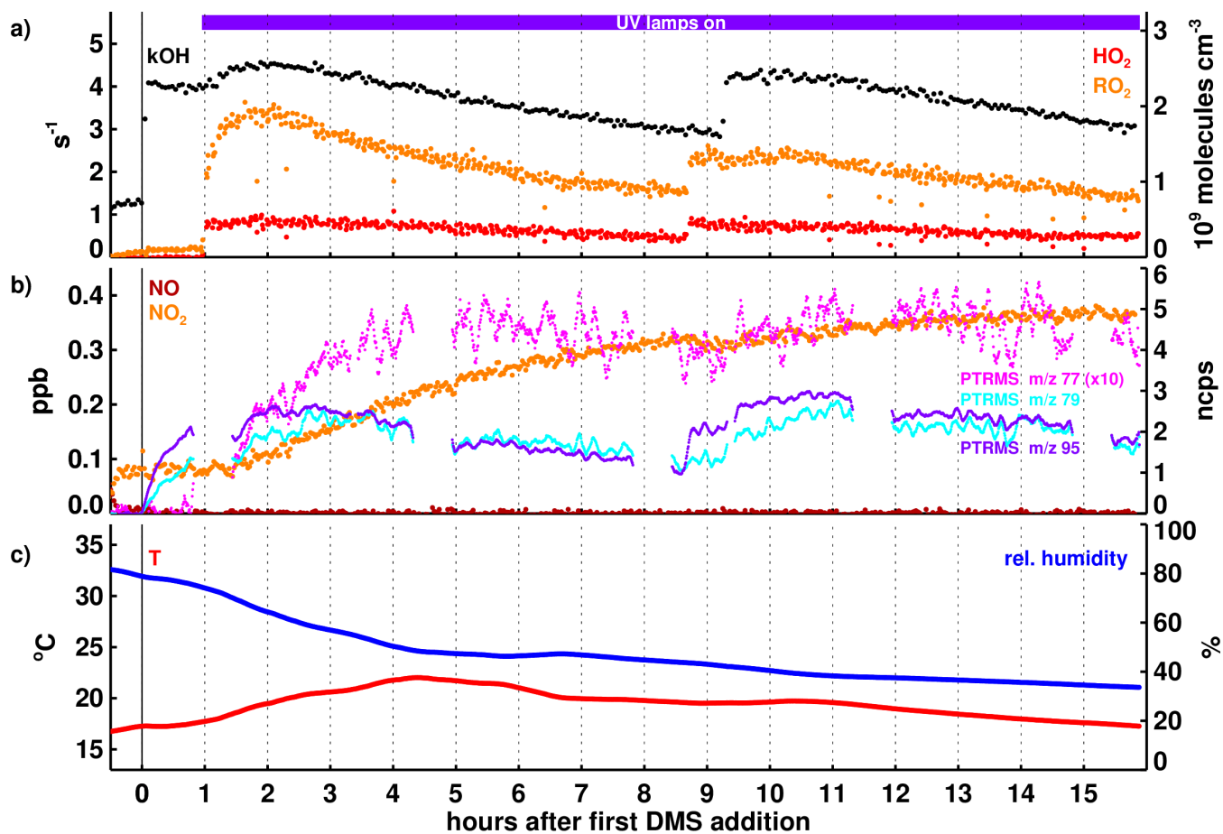
655 Figure S2 Additional parameters in Experiment II, with time in hours after the first DMS injection and the period with the UV lamps turned on indicated by the coloured bar on the top of panel a. In panel a) k_{OH} and radical concentrations are shown with the position of the labels indicating which axis refers to which species. In panel b), NO and NO 2 mixing ratios are given, together with raw PTRMS signals at m/z ratios that are potentially related to relevant products and intermediates ( m/z 77: CH 3 SCHO; m/z 79: DMSO; m/z 95: DMSO 2 or CH 3 SCH 2 OOH; see Section 2.3 of the article). In panel c), temperature and humidity in the SAPHIR chamber are shown.
