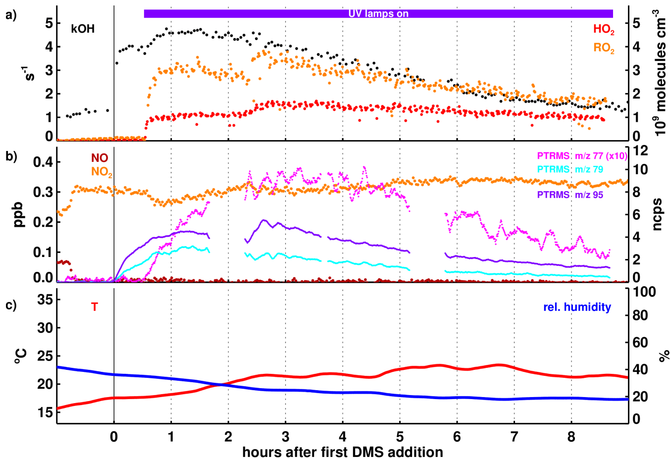
645 Figure S1 Additional parameters in Experiment I, with time in hours after the first DMS injection and the period with the UV lamps turned on indicated by the coloured bar on the top of panel a. In panel a) k_{\text{OH}} and radical concentrations are shown with the position of the labels indicating which axis refers to which species. In panel b), NO and NO 2 mixing ratios are given, together with raw PTRMS signals at m/z ratios that are potentially related to relevant products and intermediates (m/z 77: CH 3 SCHO ; m/z 79: DMSO ; m/z 95: DMSO 2 or CH 3 SCH 2 OOH ; see Section 2.3 of the article). In panel c), temperature and 650 humidity in the SAPHIR chamber are shown.
