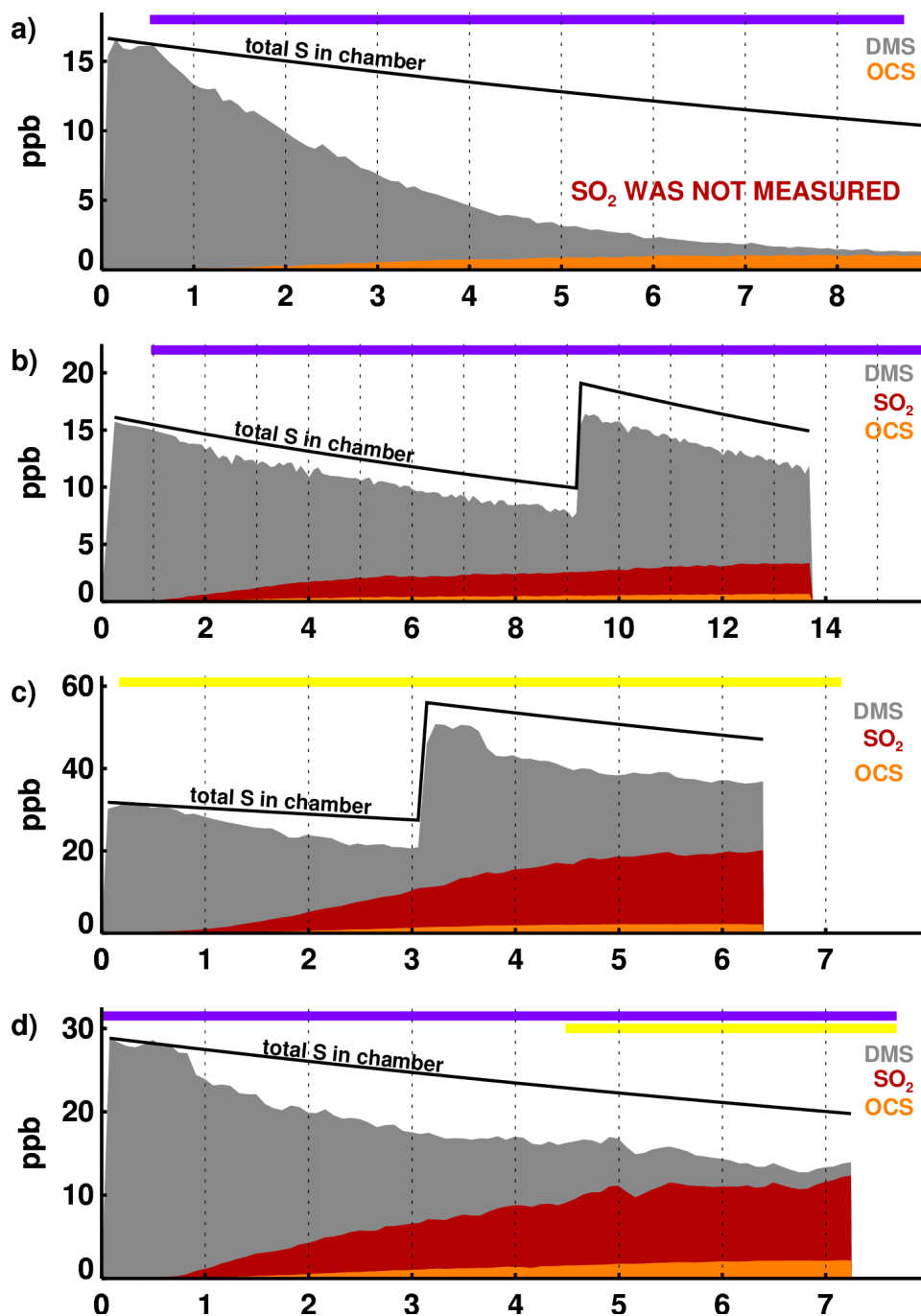
685 Figure S6 Sulfur budget of measured sulfur gases (panels a – d correspond to Experiments I – IV respectively). The black line indicates the total sulfur expected in the SAPHIR chamber accounting for DMS additions and chamber loss by dilution. In Experiments II – IV, DMS and two main product sulfur gases, SO 2 and OCS, are measured, and together make up between 70 and 80 % of the total sulfur in the chamber (based on injected DMS and the chamber dilution rate). We expect the remaining part of the sulfur budget to be made up by other product gases (e.g. dimethyl sulfoxide, DMSO, as the major product gas of the OH addition channel) and intermediates including HPMTF and TPA.
