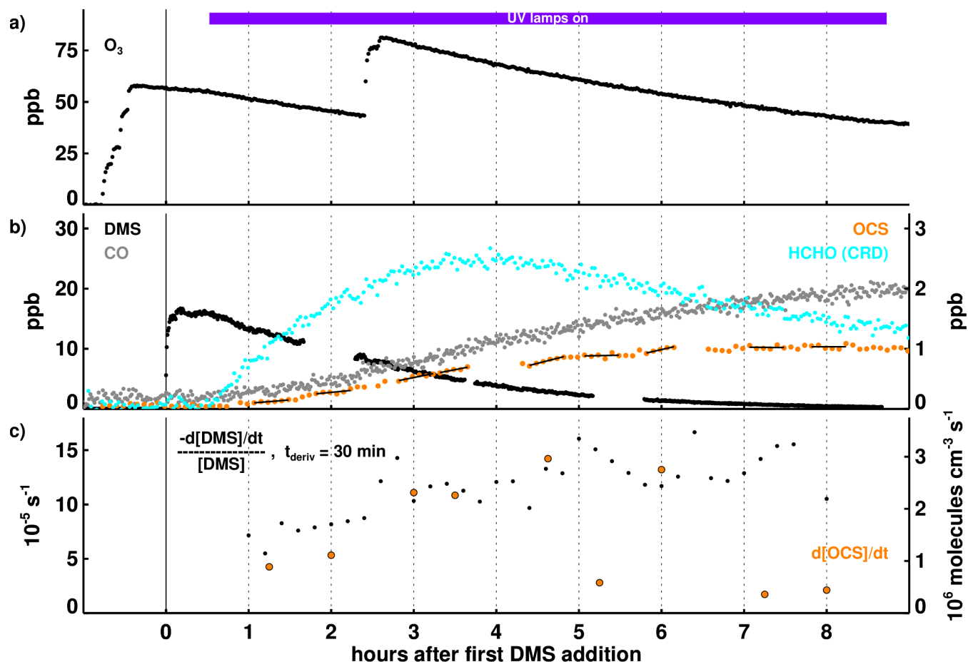
Figure 1 Time series of selected parameters in Experiment I, with time in hours after the first DMS injection and the period with the UV lamps turned on indicated by the coloured bar on the top of panel a). In panels a) and b), mixing ratios for trace gases are shown with the position of the labels indicating which axis refers to which species. In panel c), the first order DMS decay rate is determined for each individual point by a linear least squares fit of the DMS concentration data within \pm 15 minutes of this point. OCS production rates given in panel c) are calculated by linear least squares fitting of the OCS concentration data marked with the black lines in panel b), each encompassing 30 minutes of data (the time periods were chosen to avoid data gaps and periods where the production rate changed significantly within 30 minutes). Both DMS loss and OCS formation rates shown are corrected for the loss induced by the replenishment flow in the SAPHIR.
