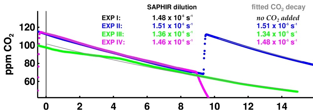
690 Figure S7 Observed decrease in CO 2 mixing ratios and comparison to the dilution rates calculated from the flow into the SAPHIR chamber.
