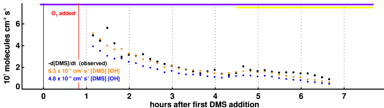
680 Figure S5 Comparison of observed (black) to expected DMS removal rate (orange) in Experiment IV for k_{\text{DMS}+\text{OH}} from Barnes et al. (2006, and references therein) and OH observed by the DOAS instrument. Also shown is the theoretical DMS removal rate for just the H abstraction channel of the DMS + OH reaction (blue, also with rate constants from Barnes et al., 2006) which represents an upper limit for the HPMTF production rate.
