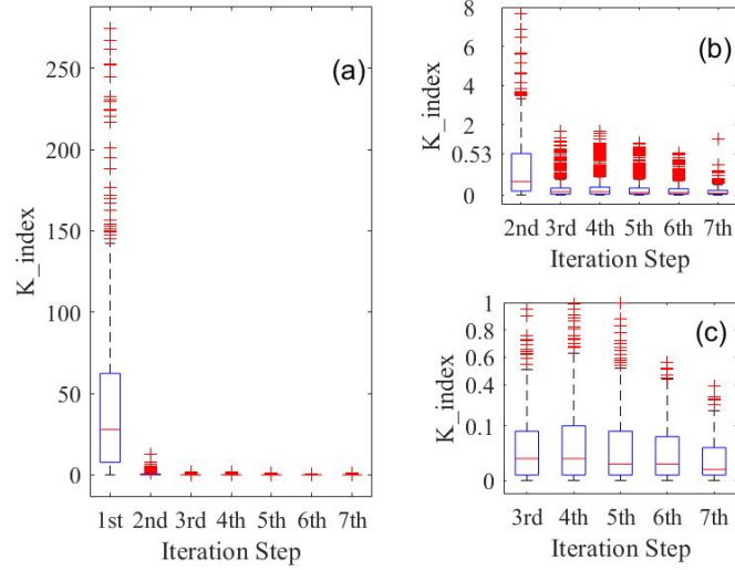
Figure 3. Box-and-whisker plots for K\_Index values at different iterations in the retrieval process of AERIOe. (a) K\_Index values calculated using 826 samples at iterations 1-7, (b) and (c) are the same as (a) but for iterations 2-7 and iterations 3-7, respectively. The boxes show upper-quartile, median (the red line through the middle of the box), and lower-quartile values for K\_Index . The whiskers extend to 1.5 times the interquartile range (IQR). Any outliers above or below the whiskers are plotted as red symbols ‘+’.
