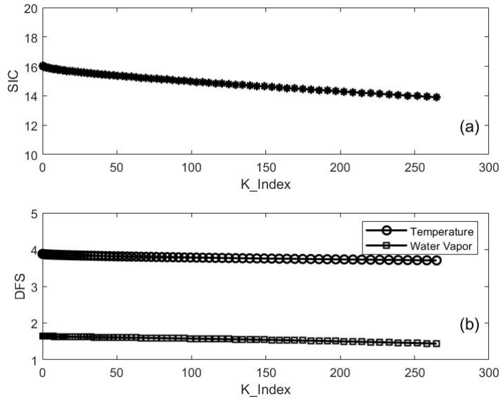
185 Figure 2. (a) The change in SIC as a function of K_Index . (b) The change in DFS as a function of K_Index for temperature (unfilled circles) and water vapor (open squares).
