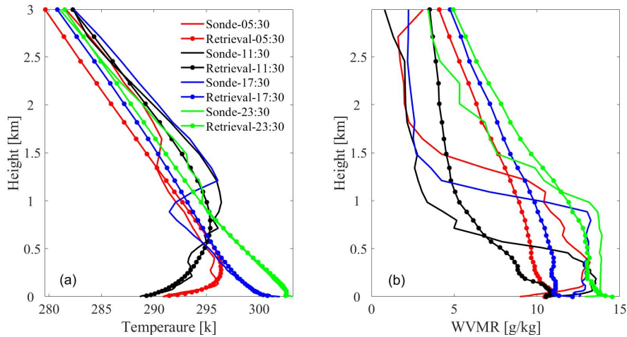
385 Figure 12. Comparisons between retrieved thermodynamic profiles and the coincident radiosonde profiles at 05:30 UTC, 11:30 UTC, 17:30 UTC and 23:30 UTC on Oct. 21, 2012. (a) Temperature profiles, (b) WVMR profiles.
