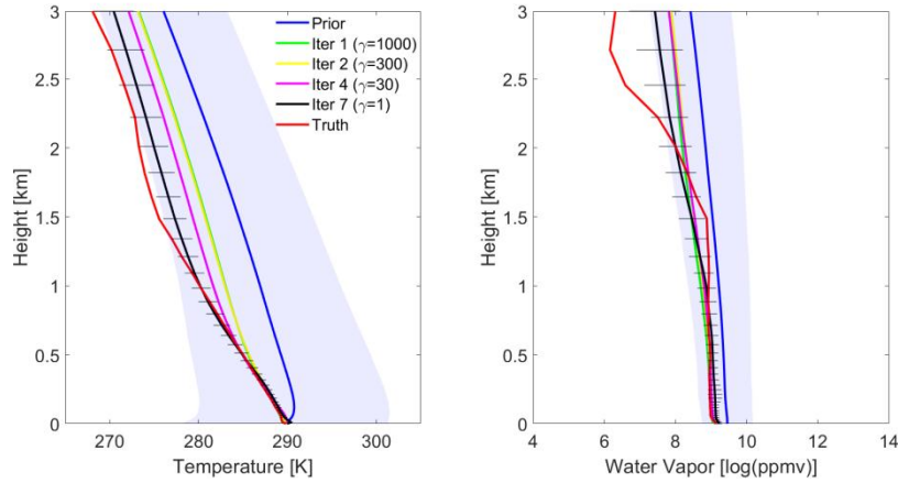
255 Figure 4. Retrieved (left) temperature and (right) water vapor profiles at various iterations from the simulated AERI observations, where the simulated observations were computed from a radiosonde (shown in red curves) launched at the SGP site at 11:30 UTC 20 Apr 2012. The prior mean profile (blue) was used as the first guess, and the blue-shaded area illustrates the 1- \sigma uncertainties in the prior. The profiles at iterations 1, 2, and 7 was shown in solid blue, yellow, purple, and black (with 1- \sigma error bars derived from \hat{S} ) lines, and the \gamma were set to 1000, 300, 30 and 1 for above iterations, respectively.
