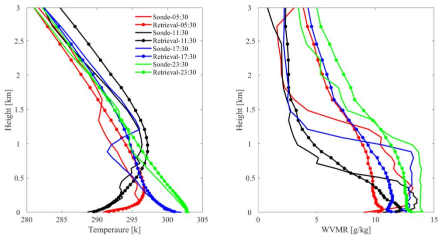
Figure 12. Comparisons between retrieved thermodynamic profiles and the coincident radiosonde profiles at 05:30 UTC, 11:30 UTC, 17:30 UTC and 23:30 UTC on Oct. 21, 2012. (Left) Temperature profiles, (right) WVMR profiles.
