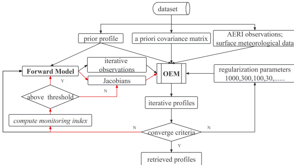
130 Figure 1. Flowchart of the Fast AERIOe retrieval process. Note that the red line indicates the Jacobian updating process. The iterative profiles and observations are defined as temperature and water vapor profiles at iteration n and computed radiance for \mathbf{X}_n , respectively. The monitoring index is used to derive the variations of \mathbf{X}_n .
