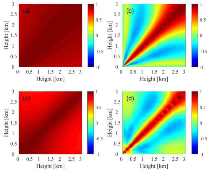
260 Figure 5. The level-to-level correlation of the prior (left) and posterior (right) for temperature (top row) and water vapor (bottom row) at 11:30 UTC 20 Apr 2012.
