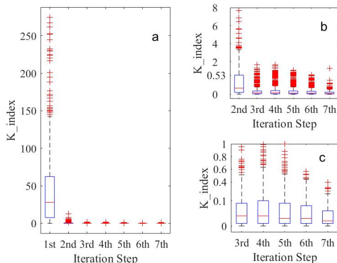
Figure 3. Box-and-whisker plots for K\_Index values at different iterations in the retrieval process of AERIOe. (a) K\_Index values calculated using 826 samples at iterations 1-7, (b) and (c) are same as (a), but for iterations 2-7 and iterations 3-7, respectively. The boxes show upper-quartile, median (the red line through the middle of the box), and lower-quartile values for K\_Index . The whiskers extend to the 1.5 times the inter quartile range (IQR). Any outliers above or below the whiskers are plotted as red symbols ‘+’.
