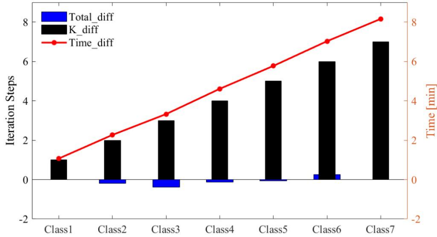
285 Figure 6. The distribution of K\_diff , Total\_diff and Time\_diff with different classes.
