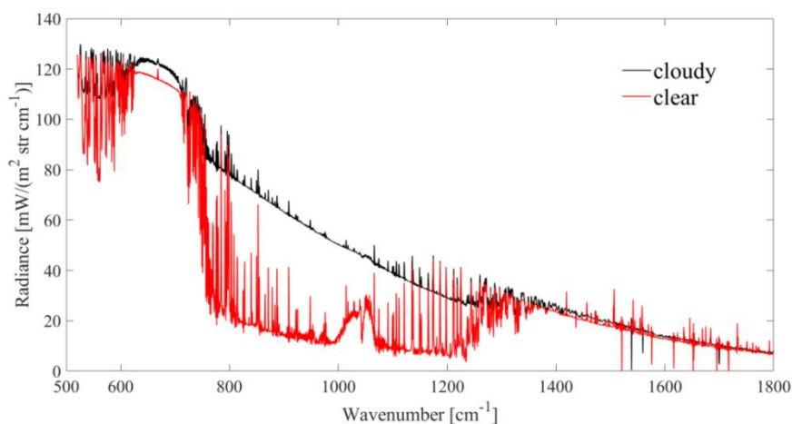
Figure 10. AERI observations in clear and cloudy sky conditions.
