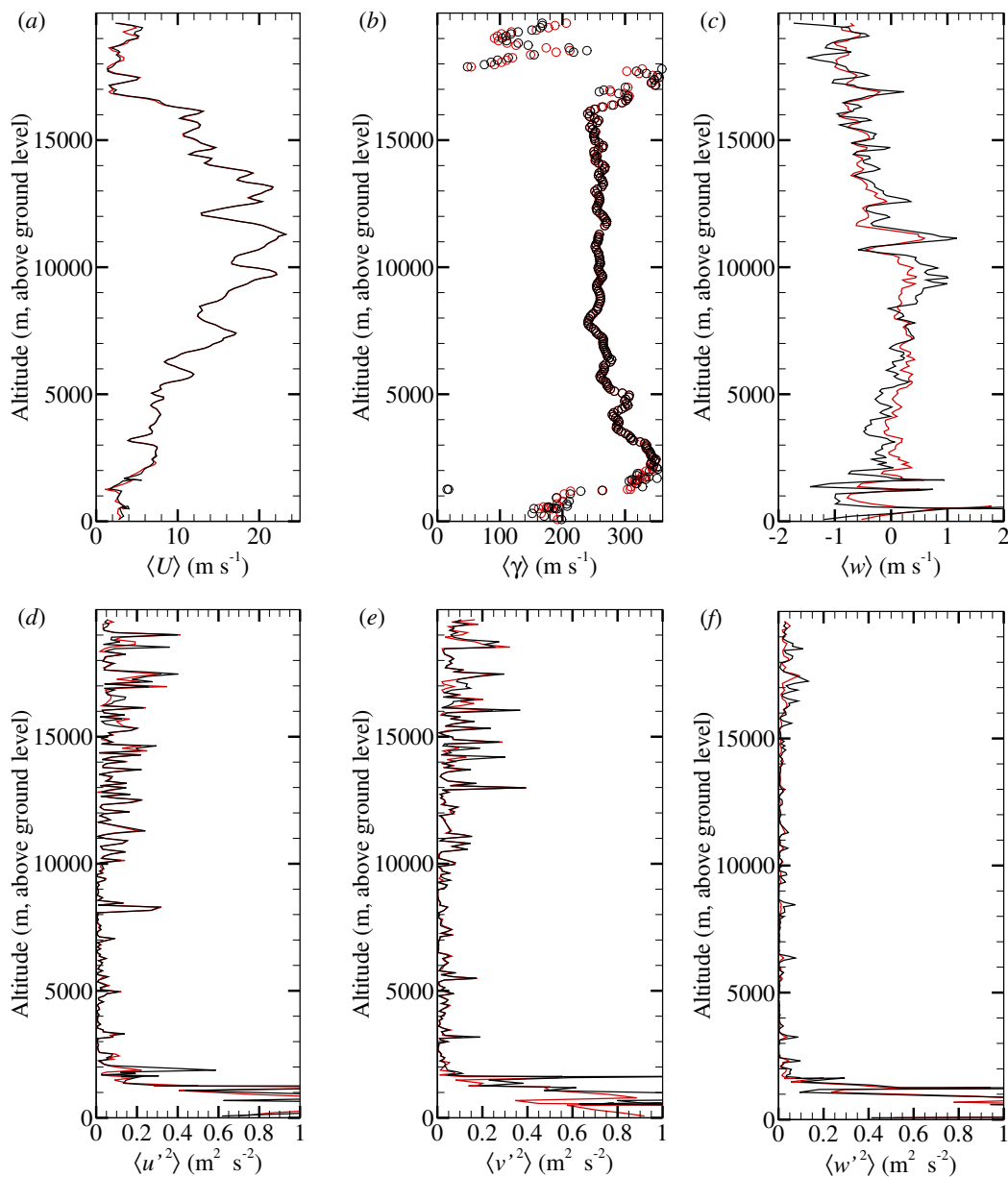
Figure A1. Figures showing comparison of (a) horizontal wind velocity magnitude, (b) horizontal wind direction, and (c) vertical component of wind velocity calculated using all the \Delta P_1 , \Delta P_{32} , and \Delta P_{54} transducers to find Q , \alpha and \beta and (shown in red) with the same properties calculated using only two the \Delta P_1 and \Delta P_{32} transducers to calculate Q and \beta with \alpha determined from the aircraft angle of attack measurement (shown in black). Comparison of resulting (a-d) \langle u'^2 \rangle , (b-e) \langle v'^2 \rangle , and (e-f) \langle w'^2 \rangle Reynolds stress tensor components is also shown.
