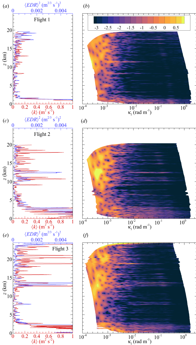
Figure 12. Profiles of \langle k \rangle and \langle EDR \rangle^2 for (a) Flight 1, (c) Flight 2, and (e) Flight 3. Contours of the base-10 logarithm of the magnitude of wavelet coefficient \log_{10}|W|^2 are also shown for (b) Flight 1, (d) Flight 2, and (f) Flight 3 as functions of longitudinal wavenumber \kappa_l and z . Contour levels are the same in (b), (d) and (f).
