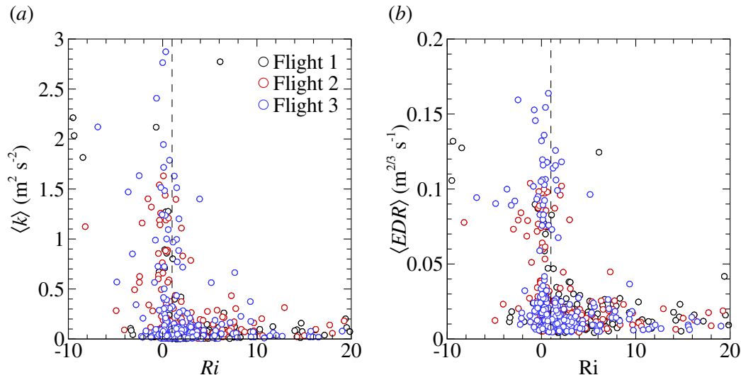
Figure 15. Comparison of (a) turbulent kinetic energy, \langle k \rangle , and (b) eddy dissipation rate, \langle EDR \rangle , to gradient Richardson number, Ri , calculated along flight trajectory. Dashed vertical line indicates Ri = 1 .
