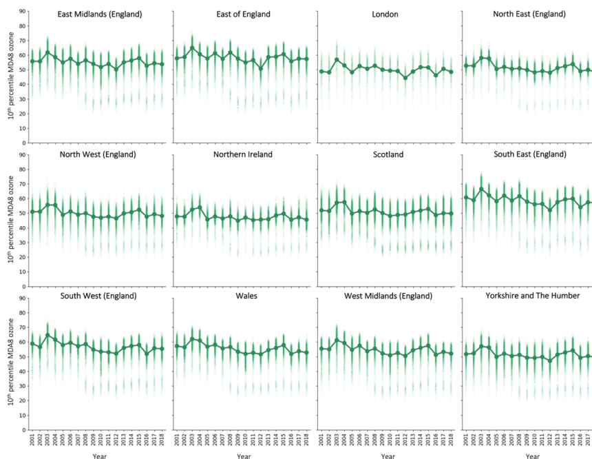
Figure A12: Regional 10 th percentile MDA8 ozone for the downscaled surface, for 2001–2018. Background dots are individual cell estimates, larger foreground dots are the yearly average.
