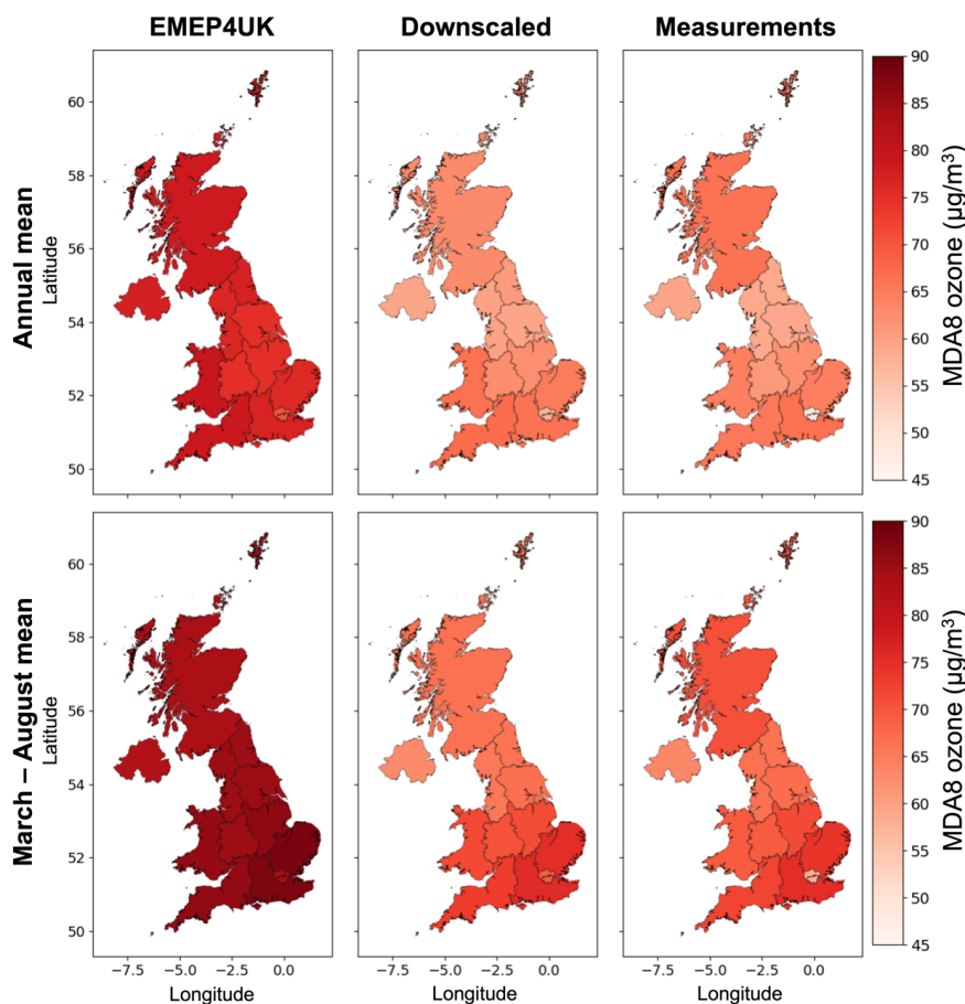
375 Figure 4: Comparing regional averages of EMEP4UK (left column), downscaled (middle column), and measurement (right column) MDA8 ozone ( \mu\text{g}/\text{m}^3 ) for 2014–2018 annual mean (top row) and March–August mean (bottom row).
