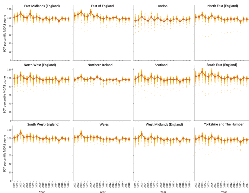
Figure A10: Regional 90 th percentile mean MDA8 ozone for the EMEP4UK surface, for 2001–2018. Background dots are individual cell estimates, larger foreground dots are the yearly average.
