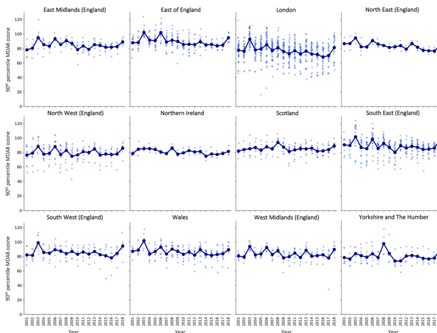
Figure A11: Regional 90 th percentile MDA8 ozone for the measurement data, for 2001–2018. Background dots are individual cell estimates, larger foreground dots are the yearly average.
