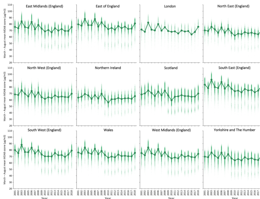
Figure A6: Regional March–August mean MDA8 ozone for the downscaled surface, for 2001–2018. Background dots are individual cell estimates, larger foreground dots are the yearly average.
