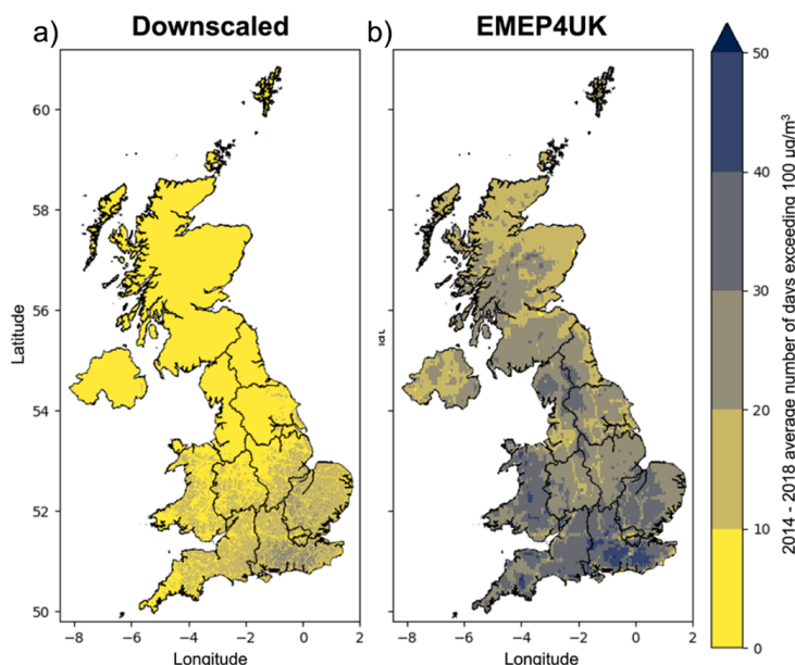
415 Figure 6: 2014–2018 average number of days per year where each cell exceeds a level of 100 \mu\text{g}/\text{m}^3 in a) downscaled ozone surface and b) EMEP4UK ozone surface.
