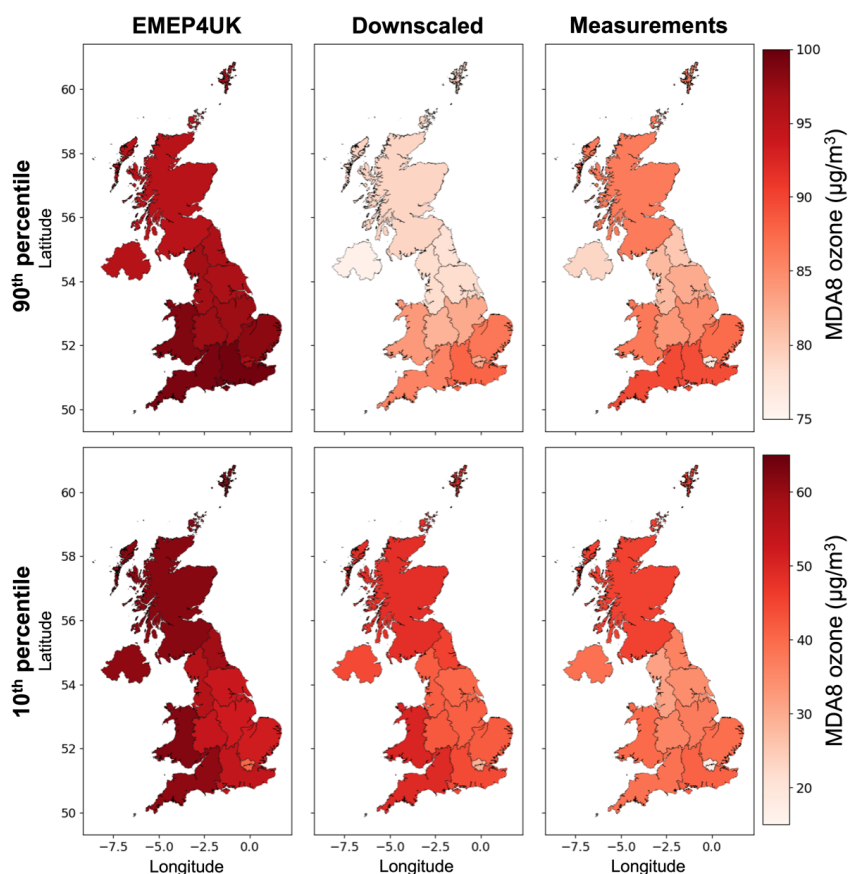
395 Figure 5: Comparing regional averages of EMEP4UK (left column), downscaled (middle column), measurement (right column) MDA8 ozone for 2014–2018 90th percentile (top row) and 10th percentile (bottom row).
