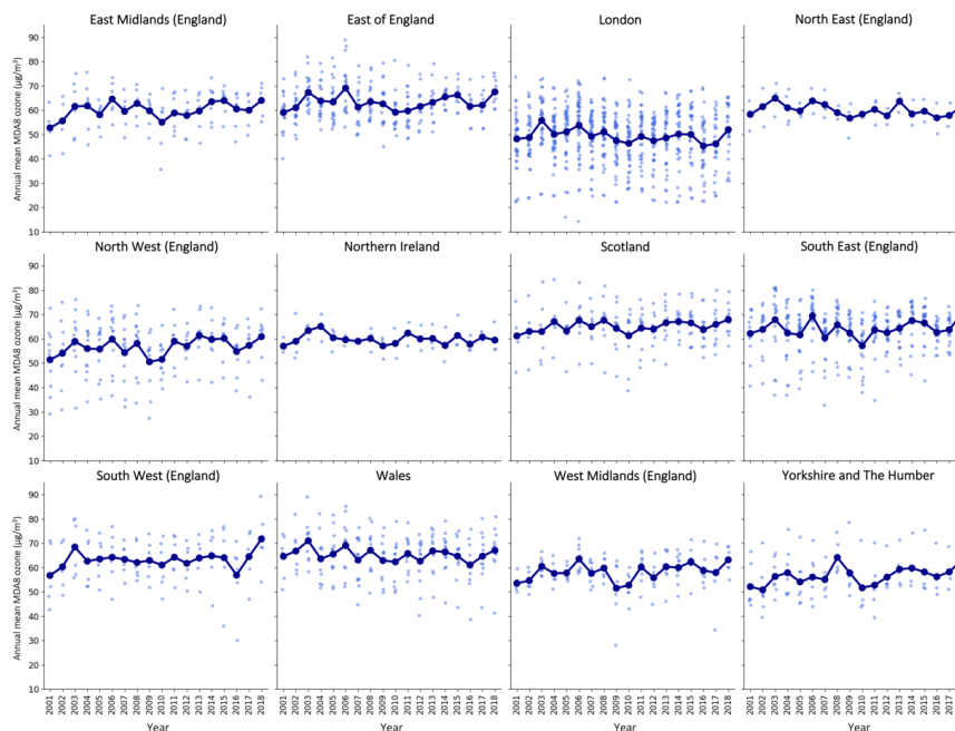
840 Figure A5: Regional annual mean MDA8 ozone for the measurement data, for 2001–2018. Background dots are individual cell estimates, larger foreground dots are the yearly average.
