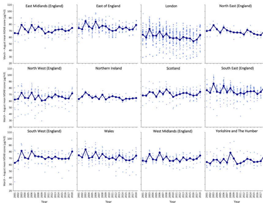
855 Figure A8: Regional March–August mean MDA8 ozone for the measurement data, for 2001–2018. Background dots are individual cell estimates, larger foreground dots are the yearly average.
