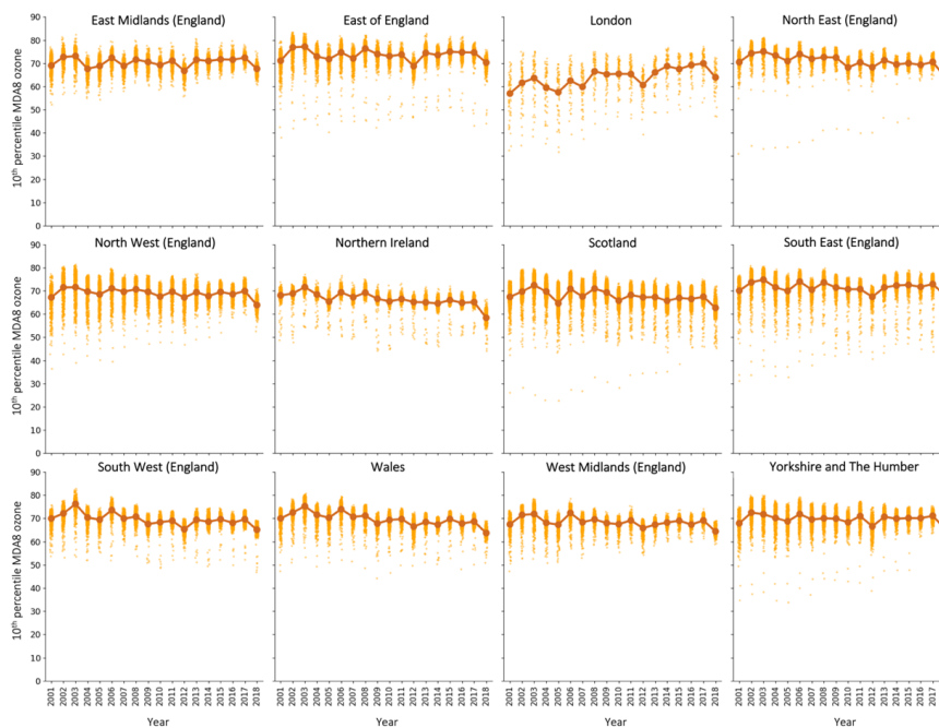
875 Figure A13: Regional 10 th percentile MDA8 ozone for the EMEP4UK surface, for 2001–2018. Background dots are individual cell estimates, larger foreground dots are the yearly average.
