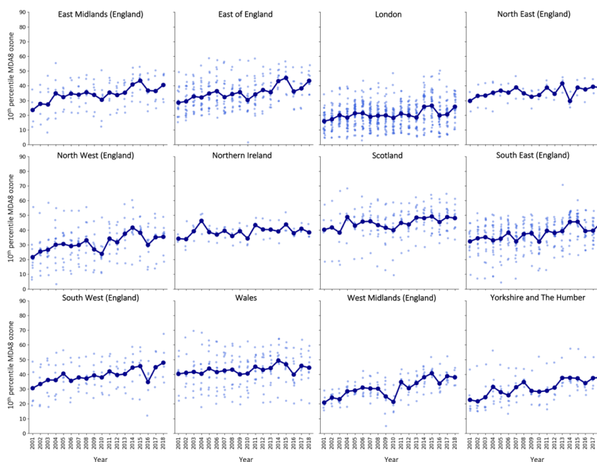
Figure A14: Regional 10 th percentile MDA8 ozone for the measurement data, for 2001–2018. Background dots are individual cell estimates, larger foreground dots are the yearly average.
