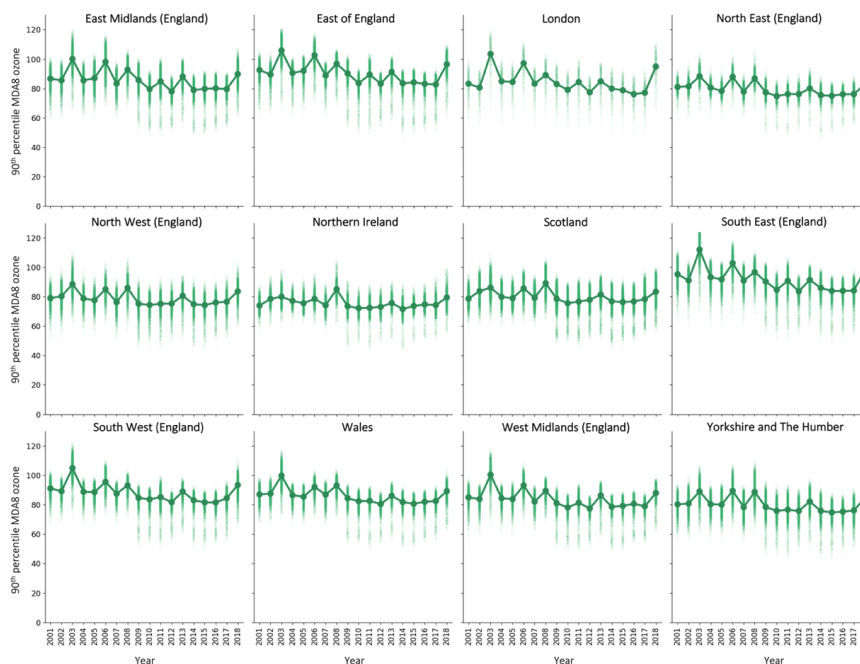
860 Figure A9: Regional 90 th percentile MDA8 ozone for the downscaled surface, for 2001–2018. Background dots are individual cell estimates, larger foreground dots are the yearly average.
