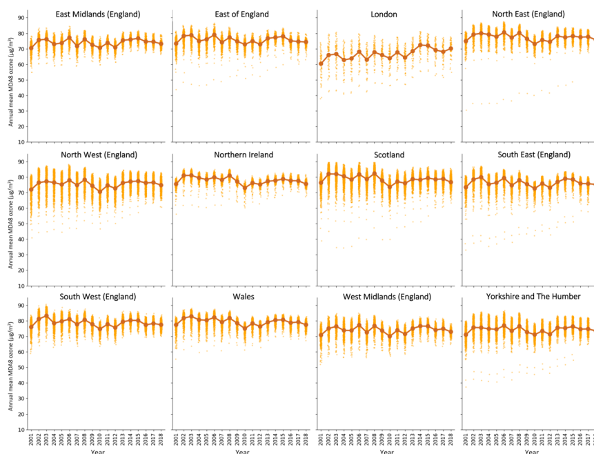
835 Figure A4: Regional annual mean MDA8 ozone for the EMEP4UK surface, for 2001–2018. Background dots are individual cell estimates, larger foreground dots are the yearly average.
