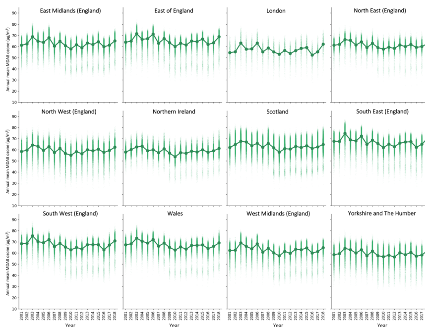
Figure A3: Regional annual mean MDA8 ozone for the downscaled surface, for 2001–2018. Background dots are individual cell estimates, larger foreground dots are the yearly average.
