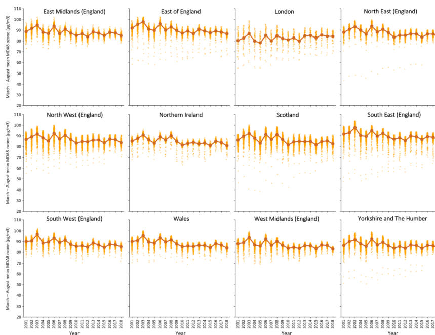
850 Figure A7: Regional March–August mean MDA8 ozone for the EMEP4UK surface, for 2001–2018. Background dots are individual cell estimates, larger foreground dots are the yearly average.
