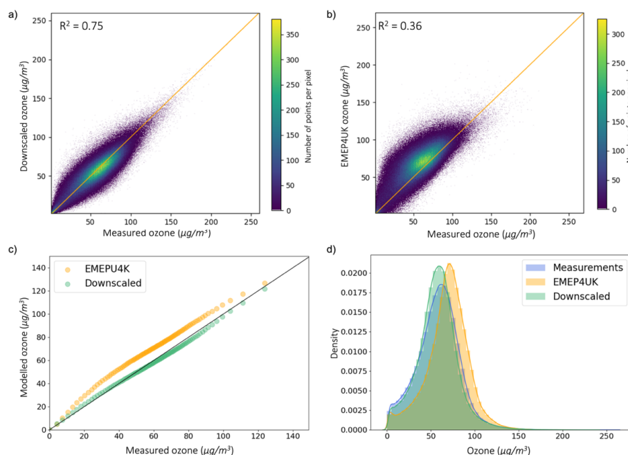
300 Figure 2: a) scatter density plot of downscaled surface vs measurement ozone; b) scatter density plot of EMEP4UK surface vs measurement ozone; c) percentile-percentile plot comparing ordered percentiles of downscaled vs measurement ozone (green) and EMEP4UK vs measurement ozone (orange); and d) density plots of measurement ozone (blue), corresponding downscaled surface ozone (green) and corresponding EMEP4UK surface ozone (orange).
