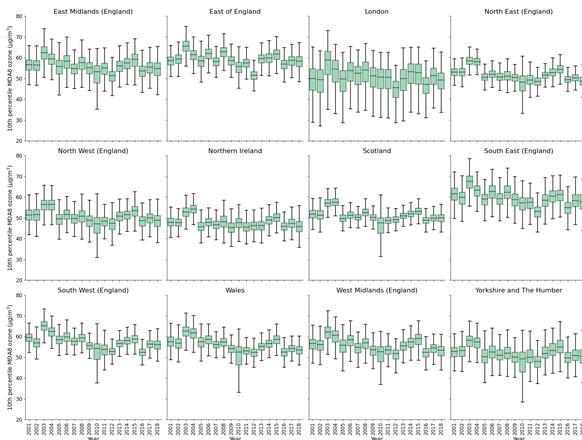
900 Figure A12: Regional yearly boxplots of 10 th percentile MDA8 ozone for the downscaled surface, for 2001–2018.
