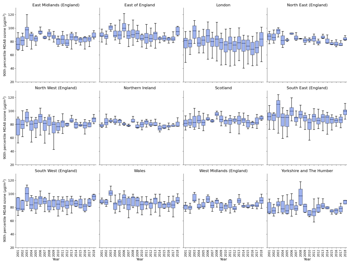
895 Figure A11: Regional yearly boxplots of 90 th percentile MDA8 ozone for the measurement data, for 2001–2018.
