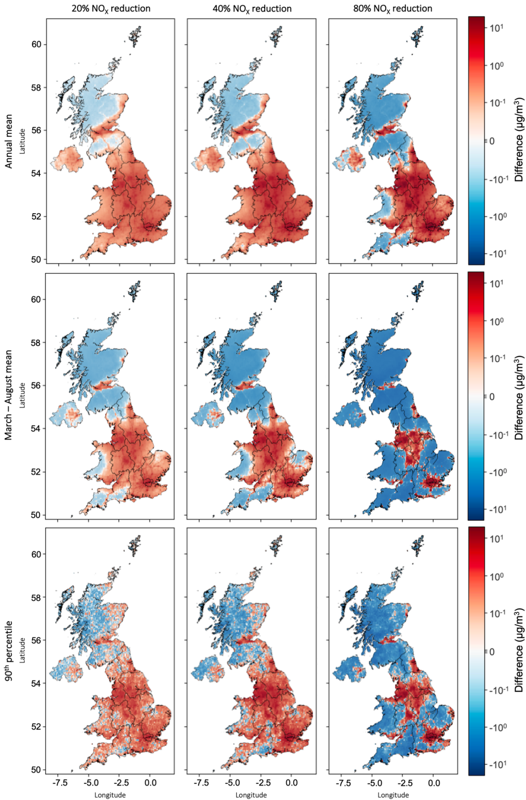
910 Figure A15: Original EMEP4UK difference in annual mean (top), March–August mean (middle), and 90 th percentile (bottom) MDA8 ozone compared to 2018 for three UK NO x scenarios: 20% reduction in NO x (left), 40% reduction in NO x (middle), 80% reduction in NO x (right).
