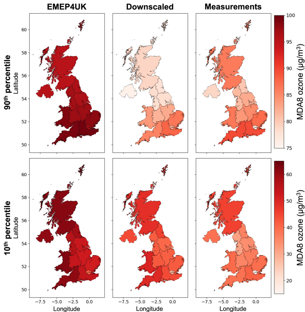
415 Figure 5: Comparing regional averages of EMEP4UK (left column), downscaled (middle column), measurement (right column) MDA8 ozone for 2014–2018 90th percentile (top row) and 10th percentile (bottom row).
