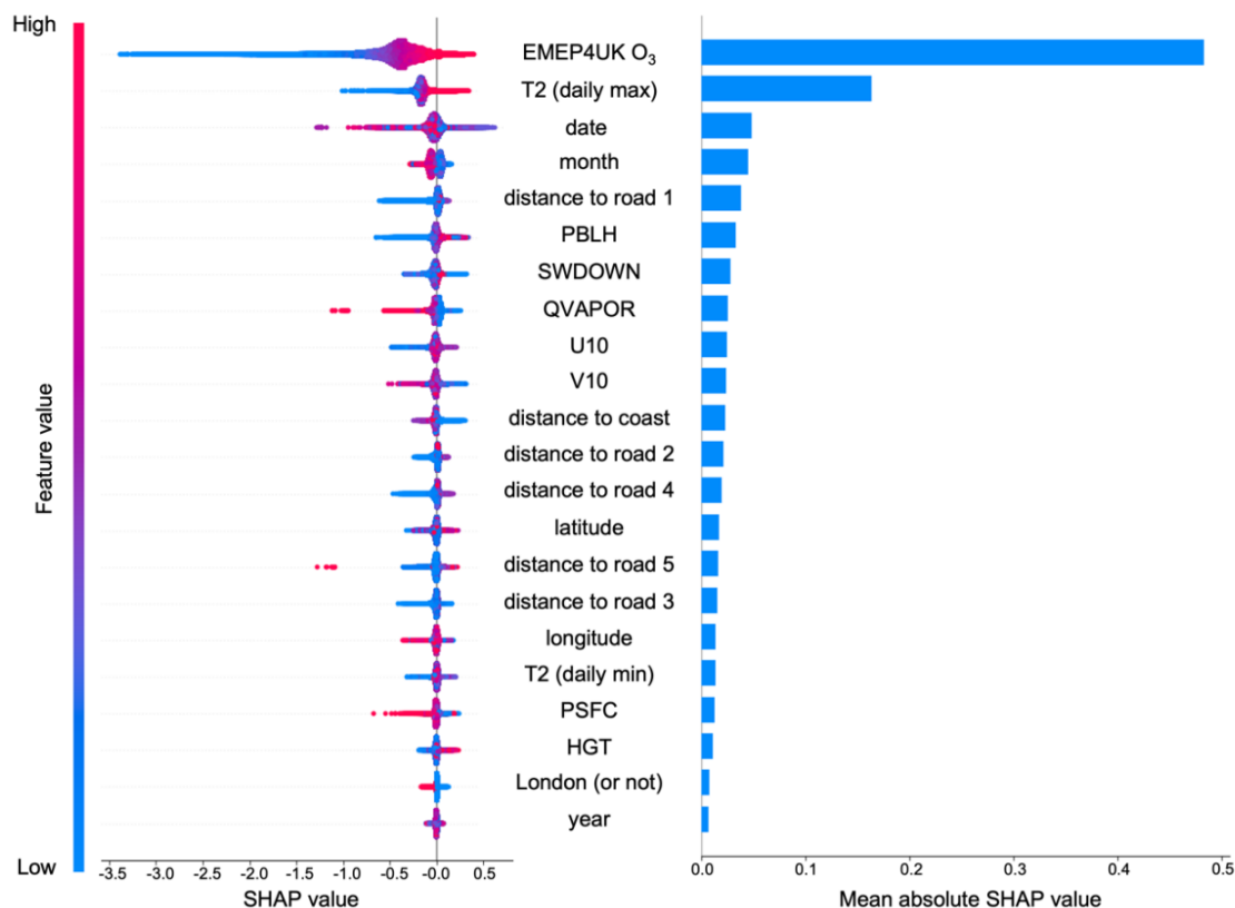
350 Figure 3: Feature importance in the GBT model ordered from most important (top), to least important (bottom). Local SHAP values (left) show the model impact of each feature based on feature value, negative SHAP value results in a lower ozone prediction, and positive SHAP value results in a higher ozone prediction. Mean absolute SHAP values (right) show the overall impact of each feature on model output.
