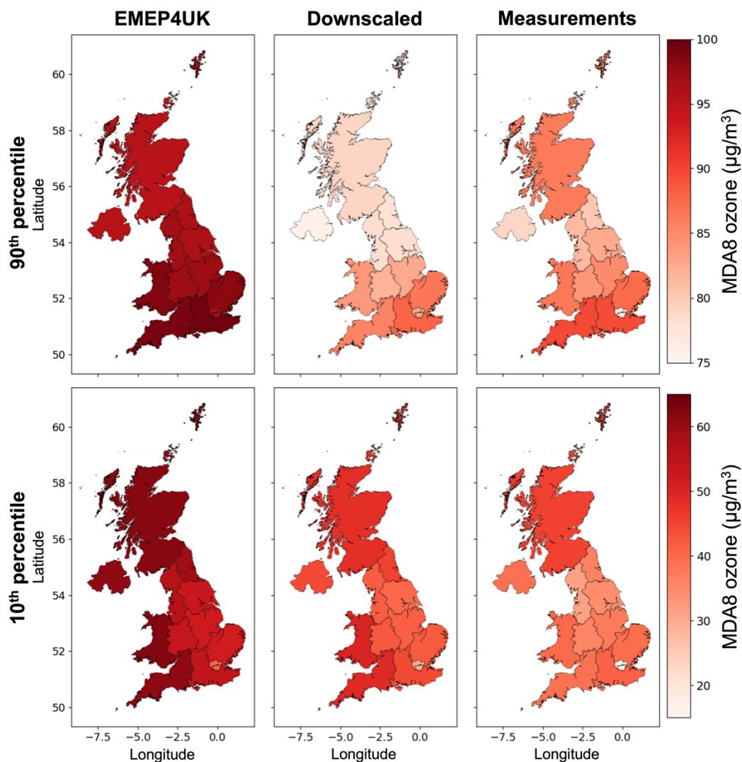
415 Figure 5: Comparing regional averages of EMEP4UK (left column), downscaled (middle column), measurement (right column) MDA8 ozone for 2014–2018 90th percentile (top row) and 10th percentile (bottom row).
