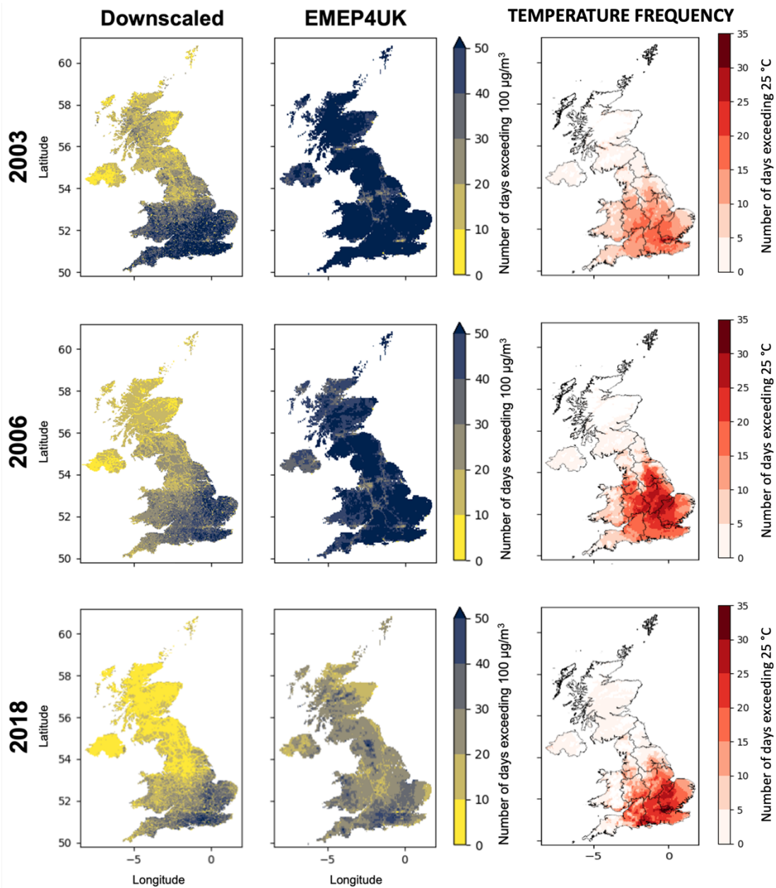
Figure 9: Number of days where each cell exceeds a level of 100 \mu\text{g}/\text{m}^3 in downscaled surface ozone (left) and EMEP4UK surface ozone (middle), for heatwaves years 2003, 2006 and 2018. Also given are the number of days exceeding 25 \text{ }^\circ\text{C} for each heatwave year.
