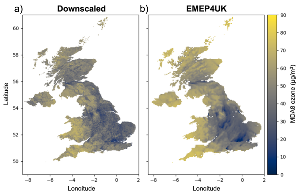
230 Figure 1: (a) An example of the downscaled MDA8 ( \mu\text{g}/\text{m}^3 ) surface (1×1 km resolution) and (b) original EMEP4UK surface (right, 5×5 km) for 01-01-2008.
