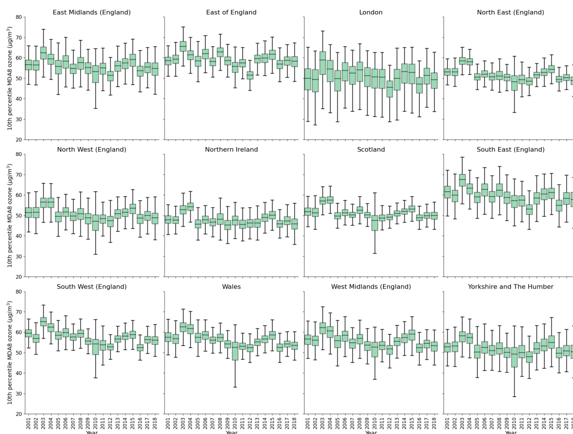
900 Figure A12: Regional yearly boxplots of 10 th percentile MDA8 ozone for the downscaled surface, for 2001–2018. Background dots are
