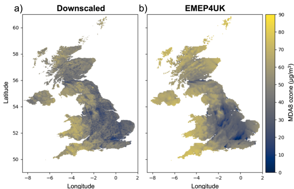
225 Figure 1: (a) An example of the downscaled MDA8 ( \mu\text{g}/\text{m}^3 ) surface (1×1 km resolution) and (b) original EMEP4UK surface (right, 5×5 km) for 01-01-2008.
