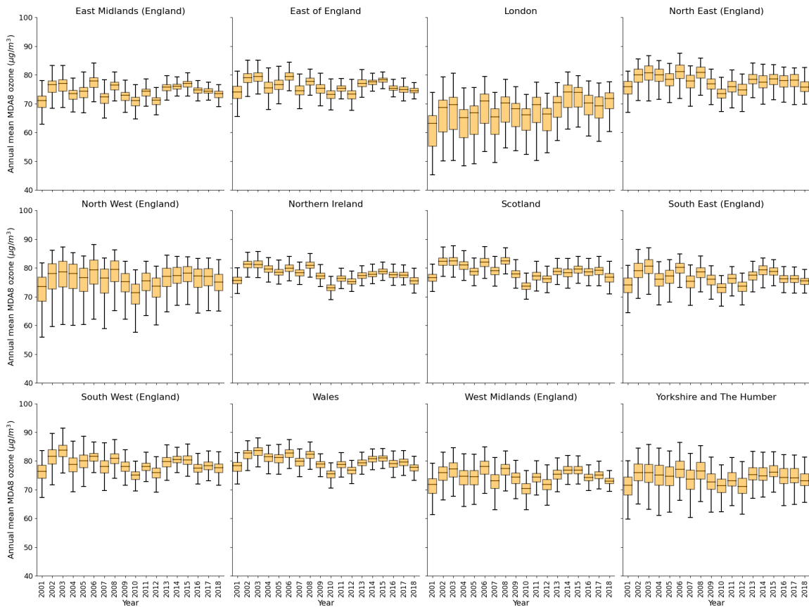
855 Figure A4: Regional yearly boxplots of annual mean MDA8 ozone for the EMEP4UK surface, for 2001–2018.
