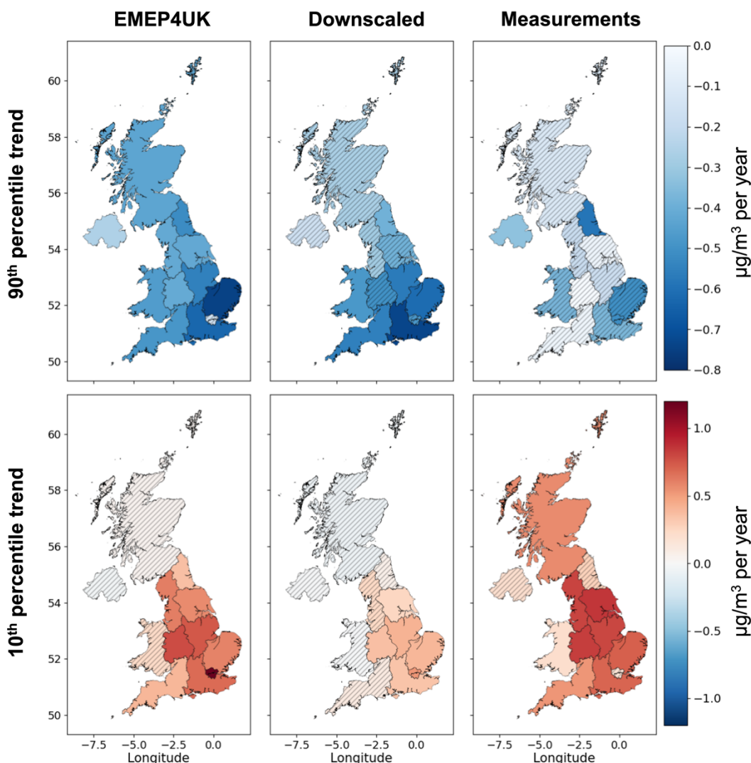
485 Figure 8: 90 th and 10 th percentile trends for each region, for each dataset. Regions with insignificant trends are hatched.
