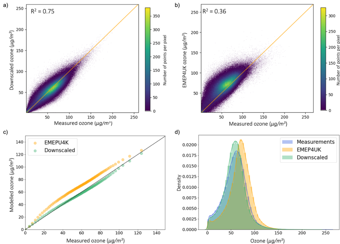
310 Figure 2: a) scatter density plot of downscaled surface vs measurement ozone; b) scatter density plot of EMEP4UK surface vs measurement ozone; c) percentile-percentile plot comparing ordered percentiles of downscaled vs measurement ozone (green) and EMEP4UK vs measurement ozone (orange); and d) density plots of measurement ozone (blue), corresponding downscaled surface ozone (green) and corresponding EMEP4UK surface ozone (orange).
