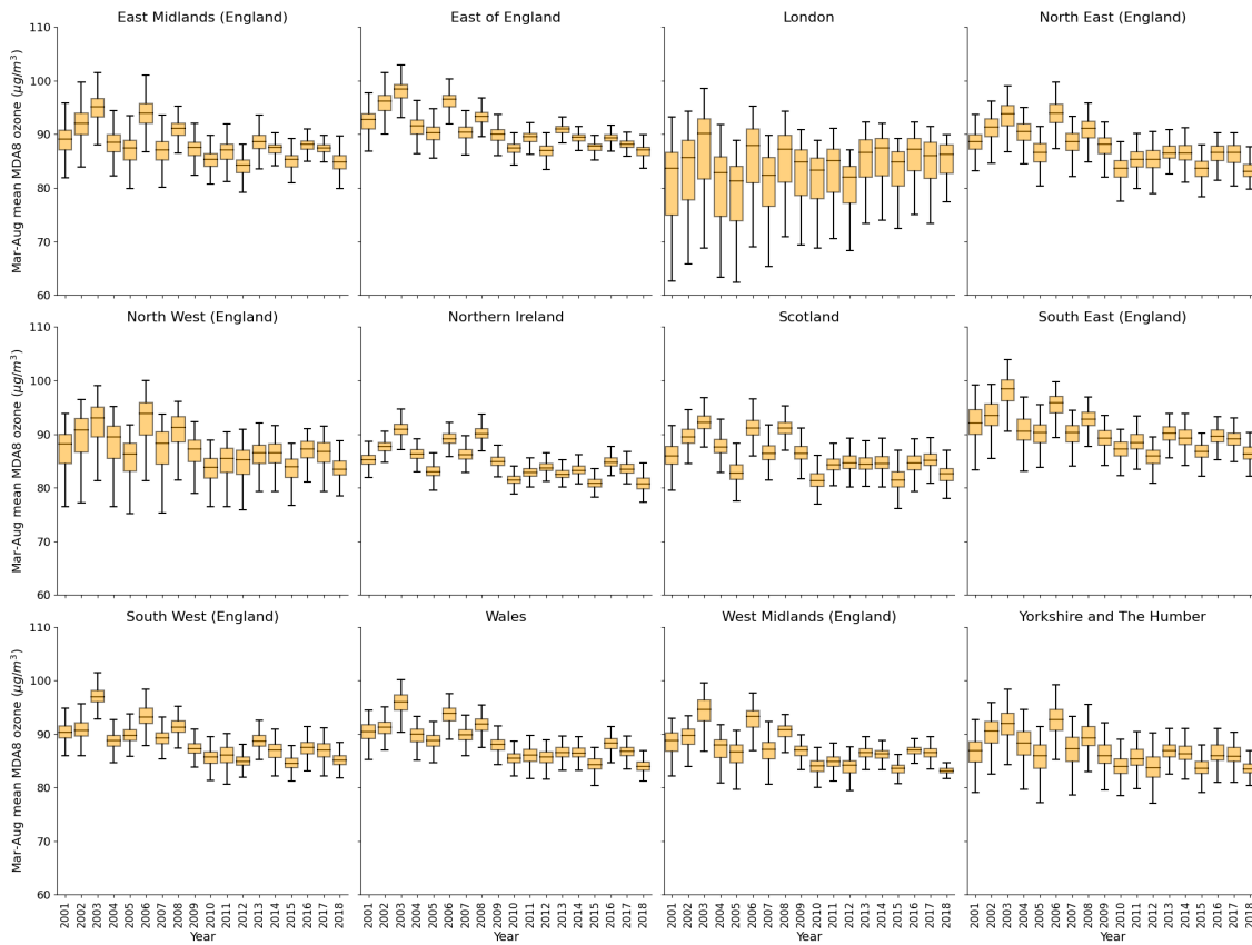
865 Figure A7: Regional yearly boxplots of March–August mean MDA8 ozone for the EMEP4UK surface, for 2001–2018.
