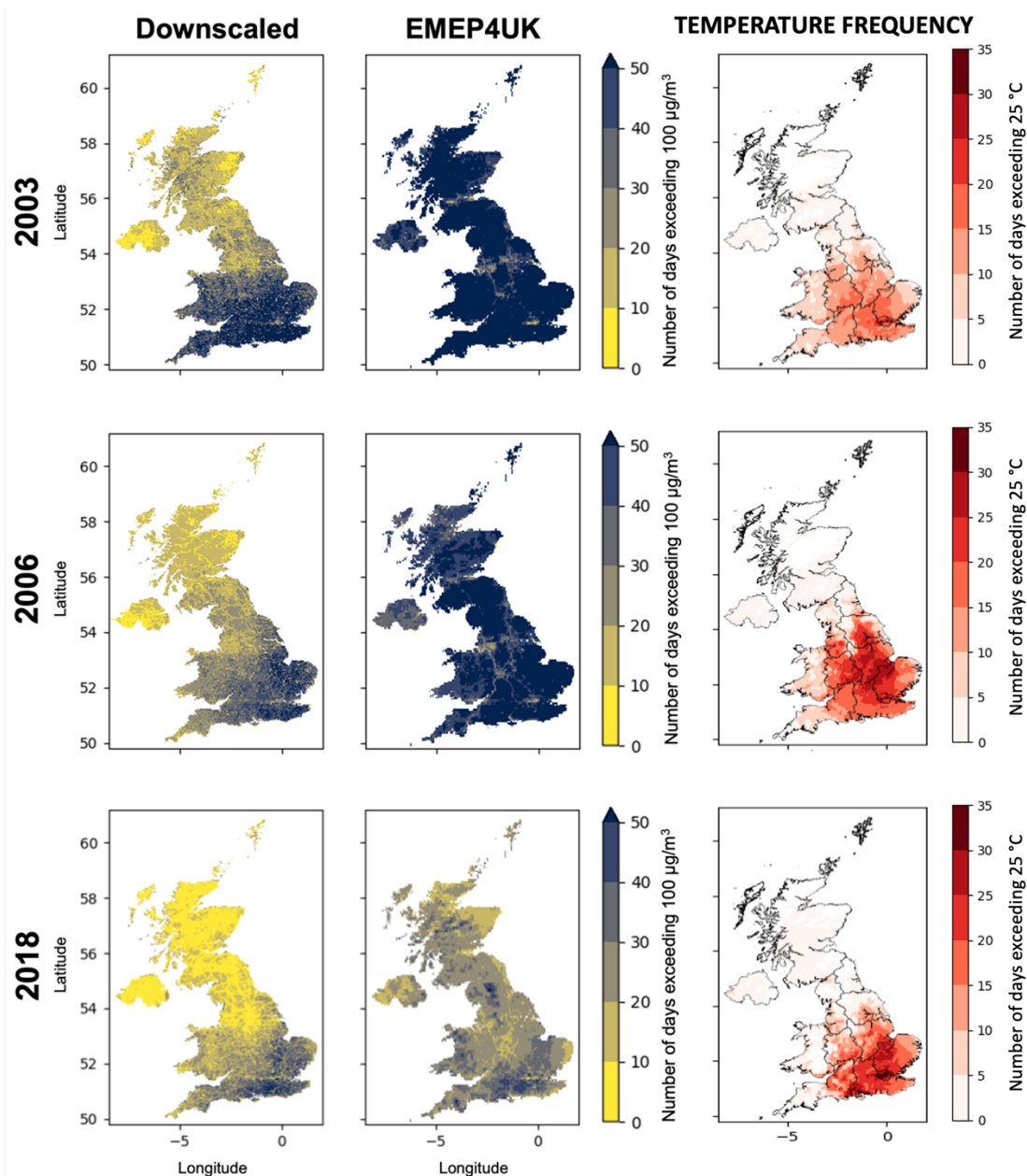
515 Figure 9: Number of days where each cell exceeds a level of 100 \mu\text{g}/\text{m}^3 in downscaled surface ozone (left) and EMEP4UK surface ozone (middle), for heatwaves years 2003, 2006 and 2018. Also given are the number of days exceeding 25^\circ\text{C} for each heatwave year.
