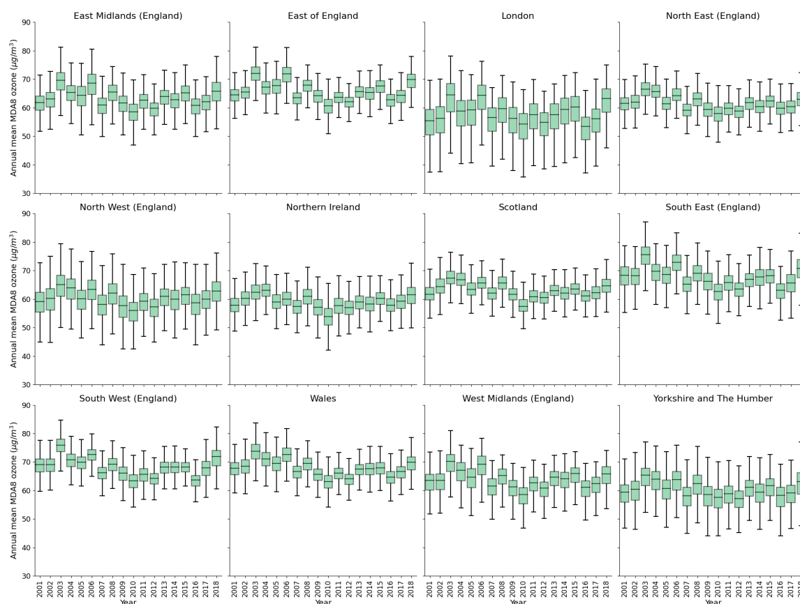
Figure A3: Regional yearly boxplots of annual mean MDA8 ozone for the downscaled surface, for 2001–2018.
