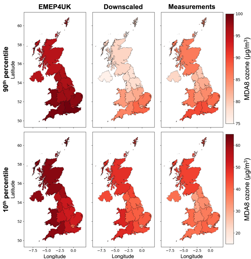
405 Figure 5: Comparing regional averages of EMEP4UK (left column), downscaled (middle column), measurement (right column) MDA8 ozone for 2014–2018 90th percentile (top row) and 10th percentile (bottom row).
