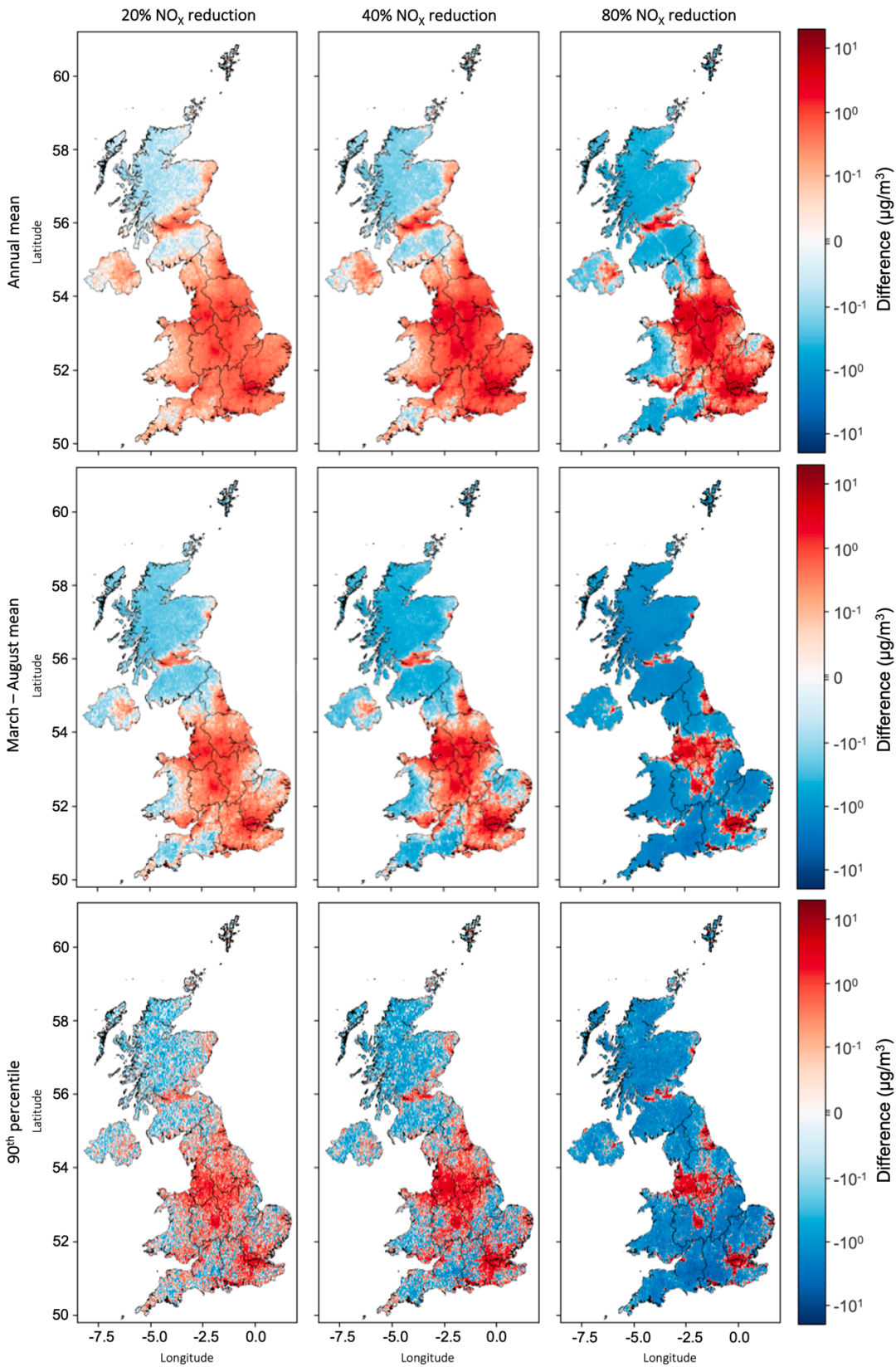
565 Figure 10: Difference in annual mean (top), March–August mean (middle), and 90 th percentile (bottom) MDA8 ozone compared to 2018 for three UK NO x scenarios: 20% reduction in NO x (left), 40% reduction in NO x (middle), 80% reduction in NO x (right).
