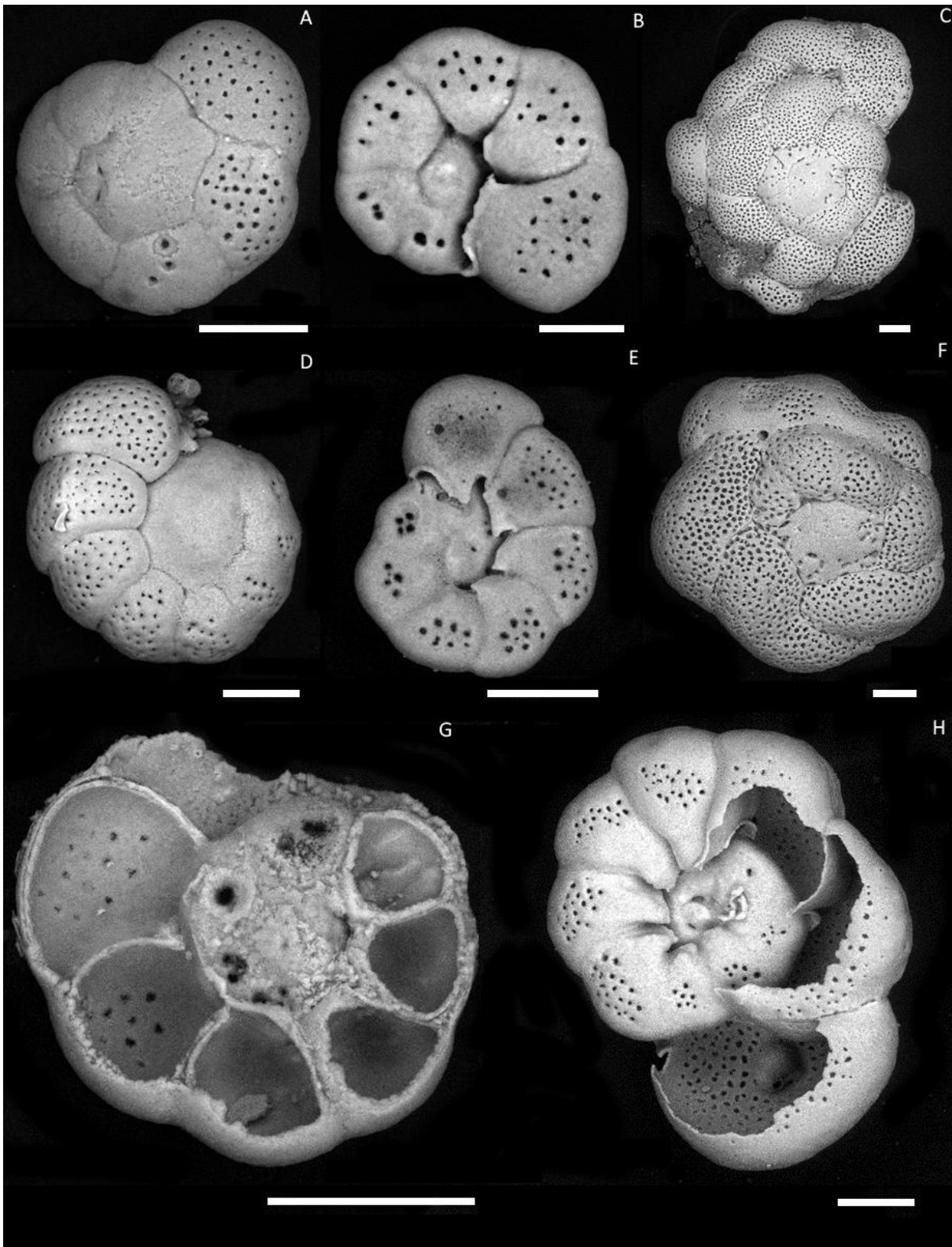
680 Figure 2. Foraminiferal strains cultured in this study. For1C1: (A) Rosalina like morphotype (11-12 chambers) reproducing asexually, dorsal view, (B) same as A, ventral view, (C) Morphotype with more than 12 chambers, starting as Rosalina morphotype and then developing annular disposition of the last chambers, dorsal view. C1Tg: (D) Rosalina like morphotype, (E) same as D, ventral view, (F) morphotype with annular arrangement of the last chambers, dorsal view. (G and H) ventral view of C1Tg with a broken test permitting to see the layered structure of the test's wall (G) and the foramen position inside of the test (H). Scale bar 50 \mu\text{m} , SEM picture in BSE 685 mode operated at 10 to 22 mPa and 20 000kV.
