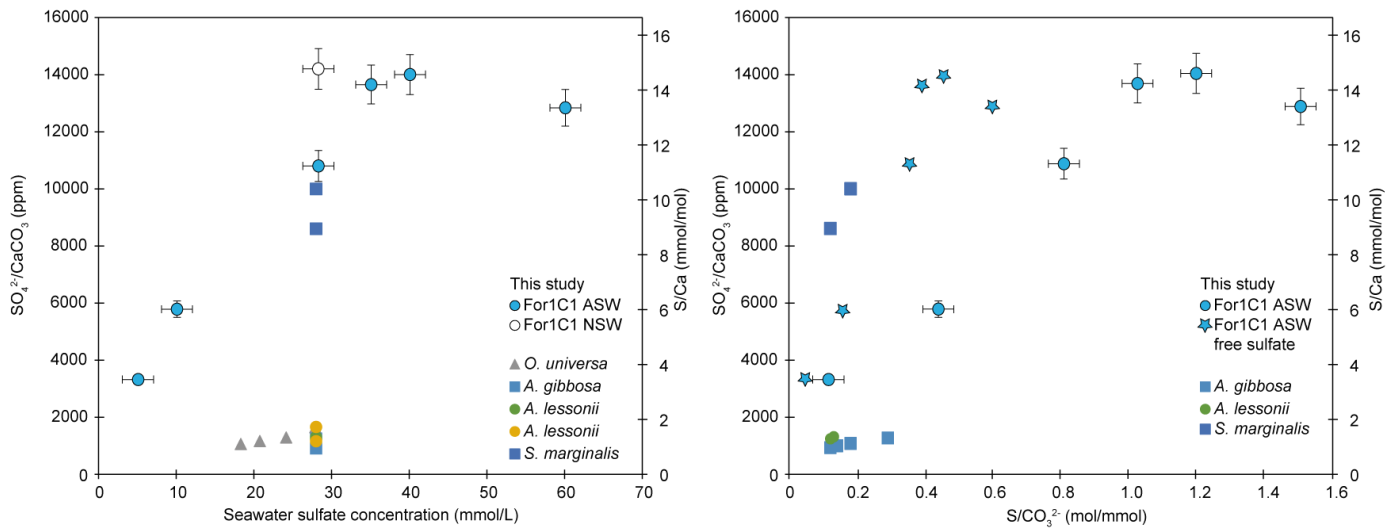
730 Figure 7. Left panel: SO_4^{2-}/CaCO_3 and S/Ca ratios on tests of the For1C1 strain at the end of SET1 and SET2 experiments, as a function of seawater [SO_4^{2-}] (5, 10, 28.2, 35, 40 and 60 mM). Right panel: SO_4^{2-}/CaCO_3 and S/Ca ratios on tests of the For1C1 strain at the end of SET1 and SET2 experiments, as a function of seawater S/CO_3^{2-} . For our experimental results, we report the values using both S as the sum of free and complexed sulfate based on our model results (circles), and as only free sulfate (stars). Each measurement has been performed on a pool of a hundred to several hundreds of specimens. Values are compared to other culture experiments of foraminifera targeting specifically the CAS content of the tests (Paris et al., 2014; van Dijk et al., 2017; 2019), and, when available, S/CO_3^{2-} as well. See Appendix B, Table B2 for details.
