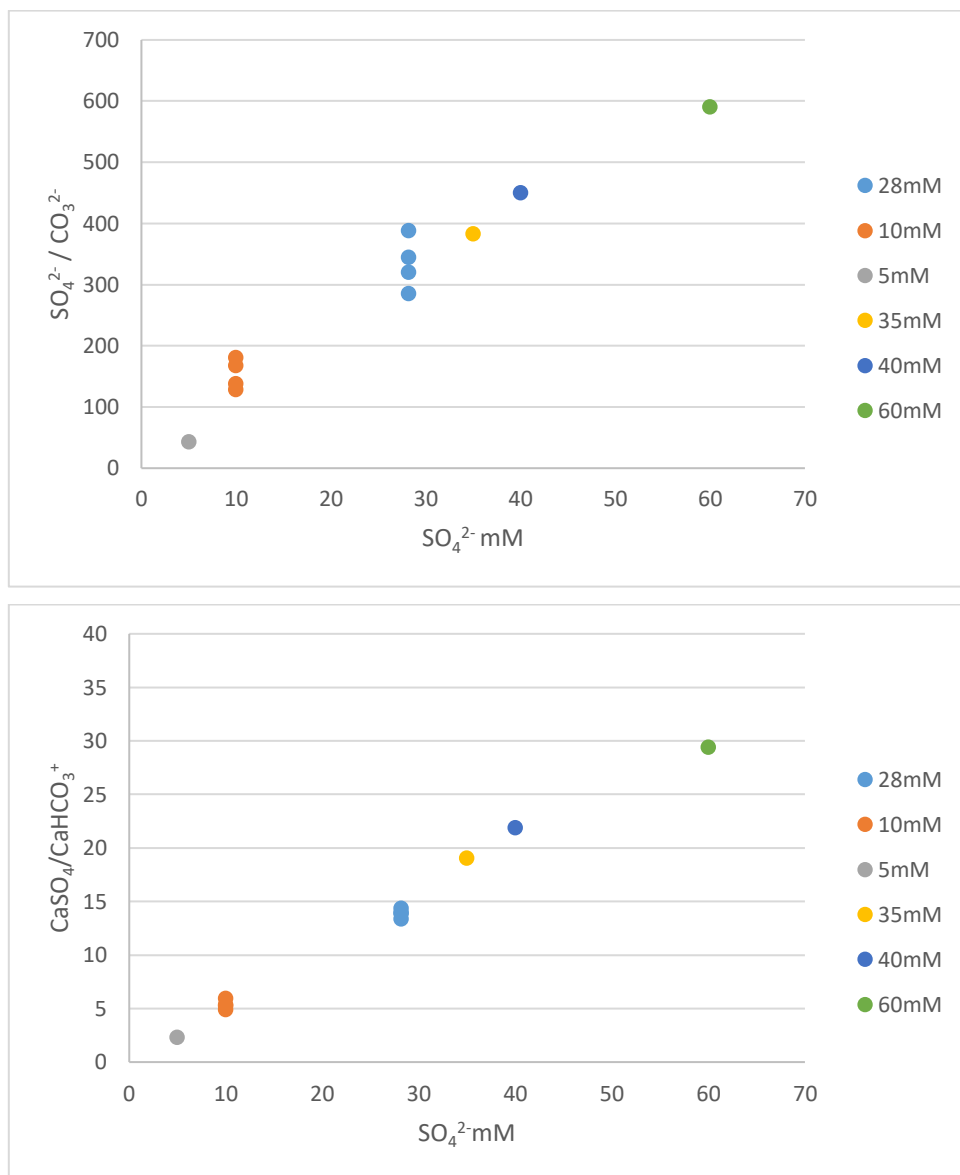
845 Figure D1. Geochemical modeling results showing \text{SO}_4^{2-}/\text{CO}_3^{2-} ratio and \text{CaSO}_4/\text{CaHCO}_3 ratio in solution as a function of total sulfate concentration in solution (dots color indicate each sulfate concentration). Each point corresponds to a different computational run, for samples where DIC and pH were measured, and were used as constraints to the model. Both ratios increase linearly to a slight inflection point at 60mM, but no plateau is seen between 28mM and 60mM.
