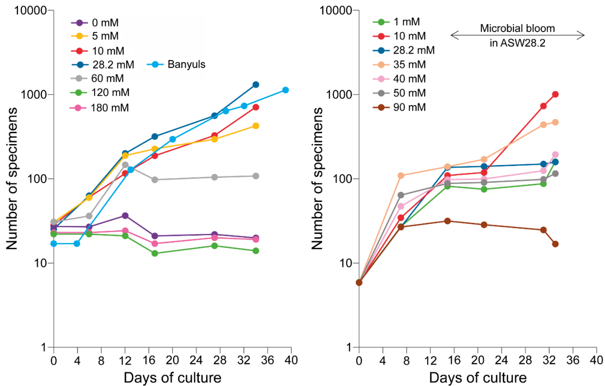
715 Figure 5. Evolution of the number of the attached specimens of the For1C1 strain in each culture medium at different [SO_4^{2-}] for (a) Set 1 and (b) Set 2. The number of foraminifera counted (with a precision of \pm 3 individual) corresponds to the living ones adhering to the bottom of the Petri dish before the change of medium. The increase in the number of individuals is due to asexual multiplication (see Appendix A). In Set 1, the largest population in terms of size occurs for 28.2 mM (ASW[28] and NSW Banyuls). In Set 2, a microbial bloom occurred after 12 days in medium ASW[28], likely affecting the reproduction rate (Appendix C, Appendix Fig. C1). The y-axes are on log scales.
