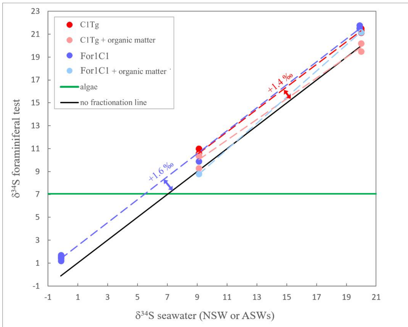
740 Figure 8. \delta^{34}\text{S} in foraminiferal test (with or without organic matter) for the two strains For1C1 and C1Tg. The two strains were cultured in several media (For1C1 in ASW[5], ASW[10] ASW[28], ASW[35], ASW[ 40], ASW[60] and NSW (Banyuls), C1Tg in NSW (Concarneau) and ASW[28]) whose \delta^{34}\text{S} has been also measured. The \delta^{34}\text{S} value of the media depend on the salts used to make the solution. The green line corresponds to the \delta^{34}\text{S} composition of the algae that were fed to the foraminifera, and whose isotopic composition remain stable. 2\sigma error bars ( \pm 0.2\text{‰} to \pm 0.3\text{‰} ) are smaller than symbols.
