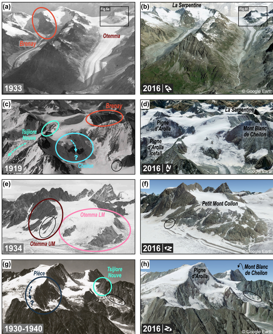
835 Figure 6: Ice cover changes across deglaciating source rockwalls in the Pigne d'Arolla massif between the beginning of the (a, c, e, g) 20th and (b, d, f, h) 21st century. For each historical photograph on the left, the approximately same view from Google Earth ( https://earth.google.com ) is shown on the right. The years shown are indicated (historical photographs by ETH Library, 2022; Swisstopo, 2022). For clarity, debris source areas are only indicated on the left (coloured circles), and mountain peaks or ridges mentioned in the text are only labelled on the right. Areas where subglacial erosion may bias our medial moraine records are indicated (dashed arrows). Note the examples of small-scale rockfalls representative for rockwall erosion (black circles).
