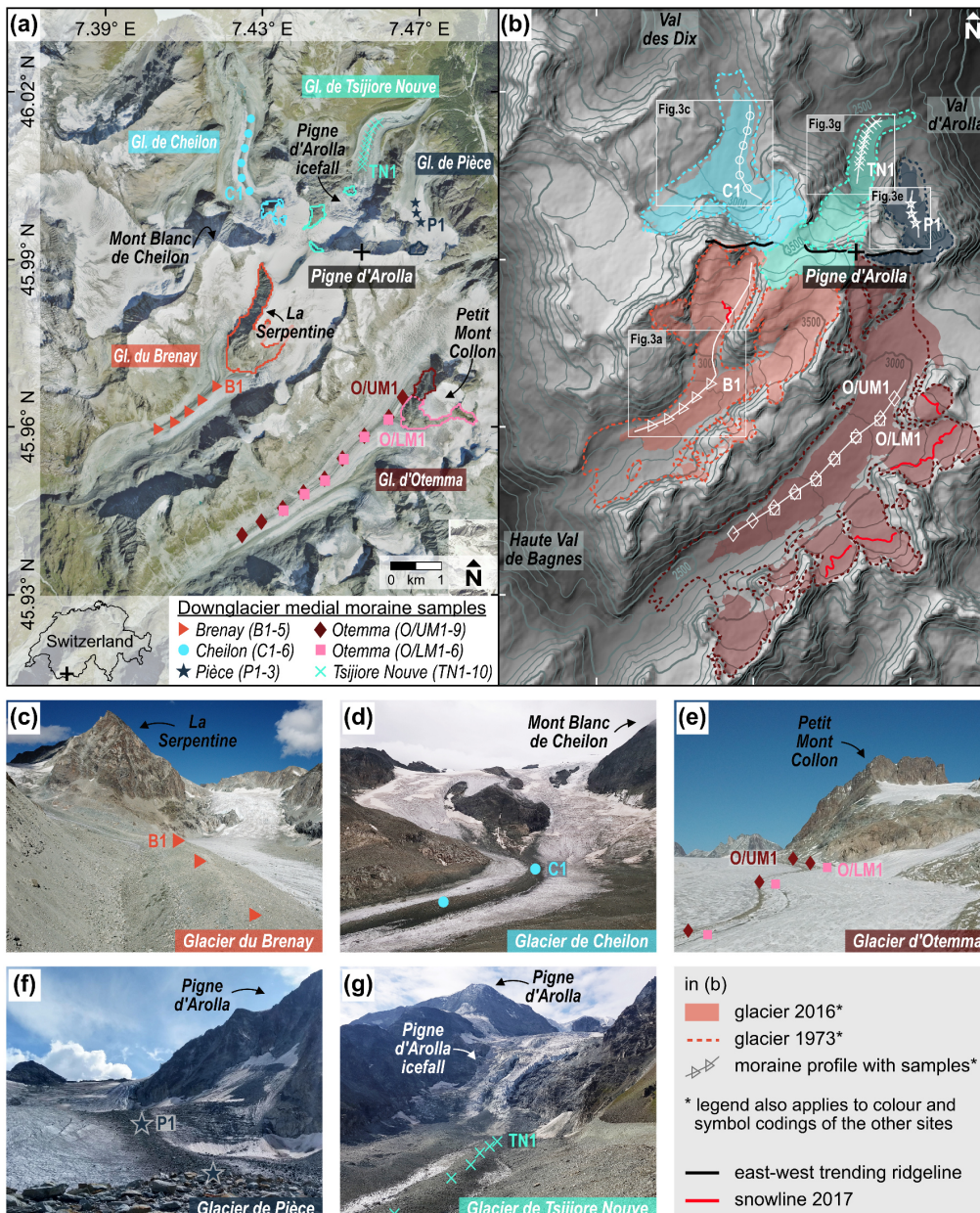
790 Figure 1: Pigne d'Arolla massif, Switzerland. (a) Orthoimage showing the five glacier catchments and their downglacier medial moraine 795 sample locations. The respective associated source rockwalls are outlined (orthoimage from 2017 by Swisstopo, 2022). (b) Hillshade image of the same area as in (a) with glacier extents in 2016 and 1973 after Linsbauer et al. (2021) and Müller et al. (1976), respectively. The snowline of the 2017 orthoimage is indicated as approximation of the recent equilibrium line altitude. Hillshade and 100 m contour lines are based on the DEM SRTM GL1 (NASA Shuttle Radar Topography Mission SRTM, 2013). White rectangles indicate map extents shown in Fig. 3. Note the east-west trending ridgeline between Pigne d'Arolla and Mont Blanc de Cheilon following closely the ~3500 m contour line. (c-g) Field photographs showing medial moraines, approximated sample locations and associated source rockwalls of (c) Glacier du Brenay, (d) Glacier de Cheilon, (e) Glacier d'Otemma (samples from Wetterauer et al., 2022a), (f) Glacier de Pièce, and (g) Glacier de Tsijjore Nouve.
