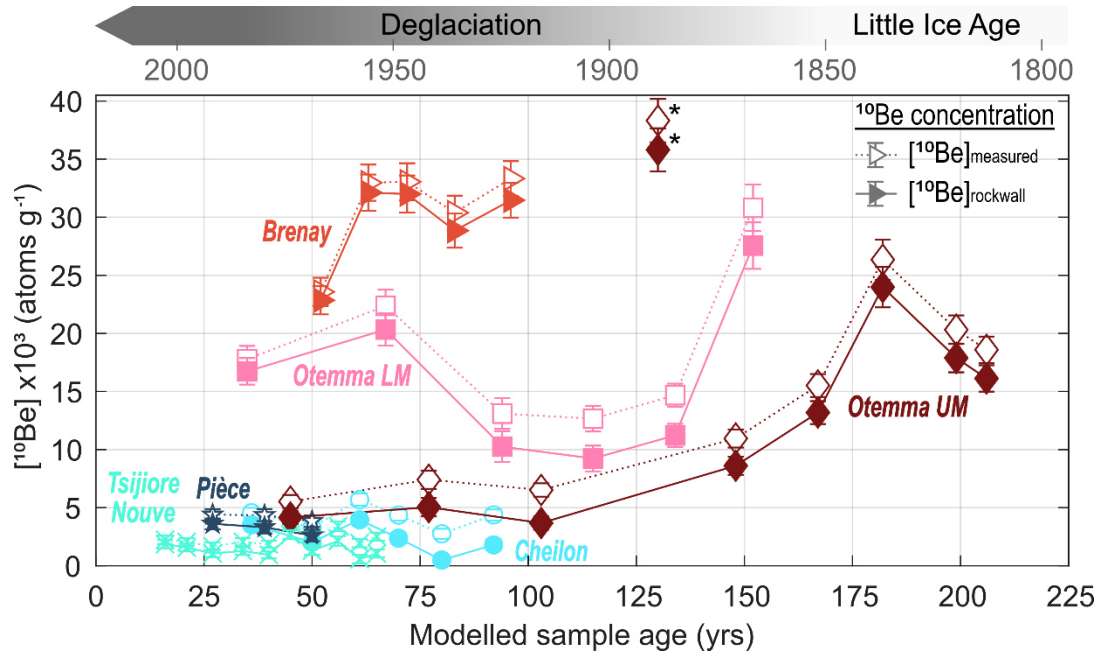
830 Figure 5: Comparison of uncorrected ( [^{10}\text{Be}]_{\text{measured}} ) and transport-corrected ( [^{10}\text{Be}]_{\text{rockwall}} ) medial moraine [^{10}\text{Be}] records of the Pigne d'Arolla massif through time (data from Glacier d'Otemma by Wetterauer et al., 2022a). Concentrations ( \pm 1\sigma analytical error) are plotted against modelled sample ages, reflecting the timing of rockwall erosion either during the Little Ice Age or the following deglaciation period, as indicated by the timeline above. Note that a re-measurement of a high concentration outlier at the Otemma UM moraine (*) at a slightly coarser grain size fraction fits the temporal trend well (see Fig. 6a in Wetterauer et al., 2022a).
