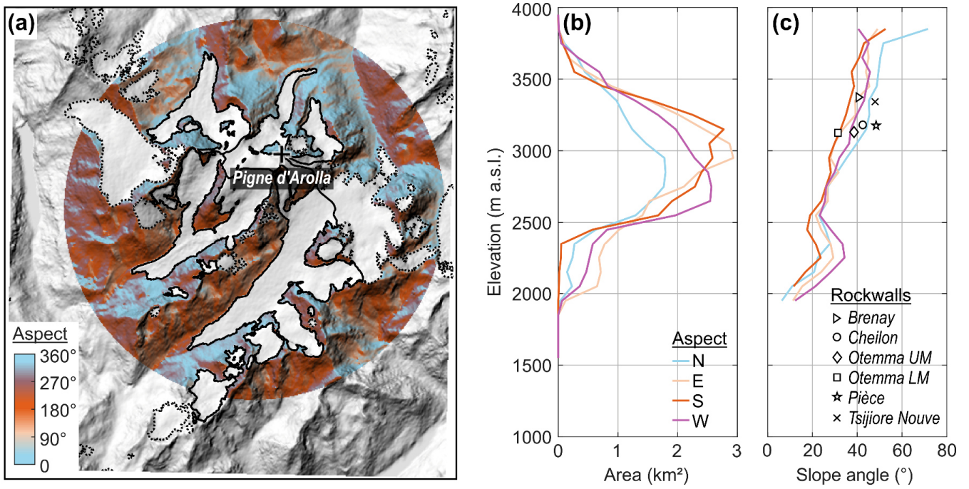
800 Figure 2: Morphology of ice-free rock faces and slopes in an area with 6 km radius, centred on the studied glaciers of the Pigne d'Arolla 805 massif. (a) Topographic map indicating the aspect of ice-free areas. Areas covered by glacial ice (dashed black outlines) are excluded from the analysis and the five studied glacier sites (bold black outline) explicitly highlighted (2016 glacier outlines by Linsbauer et al., 2021). (b) Hypsometry and (c) slope angles of ice-free areas in 100 m elevation bins, differentiated by aspect. Symbols denote the mean elevation and mean slope angle of the studied source rockwalls.
