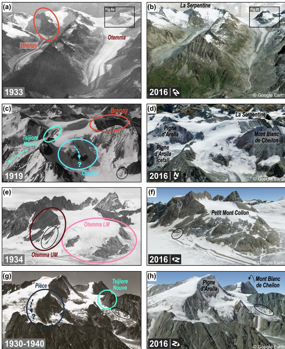
395 Figure 6: Ice cover changes across deglaciating source rockwalls in the Pigne d'Arolla massif between the beginning of the (a, c, e, g) 20th and (b, d, f, h) 21st century. For each historical photograph on the left, the approximately same view from Google Earth ( https://earth.google.com ) is shown on the right. The years shown are indicated (historical photographs by ETH Library, 2022, swisstopo, 2022). For clarity, debris source areas are only indicated on the left (coloured circles), and mountain peaks or ridges mentioned in the text are only labelled on the right. Areas where subglacial erosion may bias our medial moraine records are indicated (dashed arrows). Note the examples of small-scale rock falls representative for rockwall erosion (black circles).
