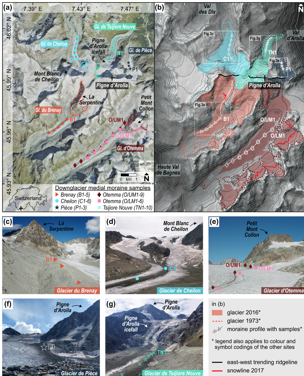
95 Figure 1: Pigne d’Arolla massif, Switzerland. (a) Orthoimage showing the five adjacent glacier catchments and their downglacier medial moraine sample locations. The respective associated source rockwalls are outlined (orthoimage from 2017 by swisstopo, 2022). (b) Hillshade image of the same area as in (a) with glacier extents in 2016 and 1973 after Linsbauer et al. (2021) and Müller et al. (1976), respectively. The snowline of the 2017 orthoimage is indicated as approximation of the recent equilibrium line altitude. Hillshade and 100 m spaced contour lines are based on the DEM SRTM GL1 (NASA SRTM, 2013). White rectangles indicate map extents shown in Fig. 3. Note the east-west trending ridgeline between Pigne d’Arolla and Mont Blanc de Cheilon following closely
