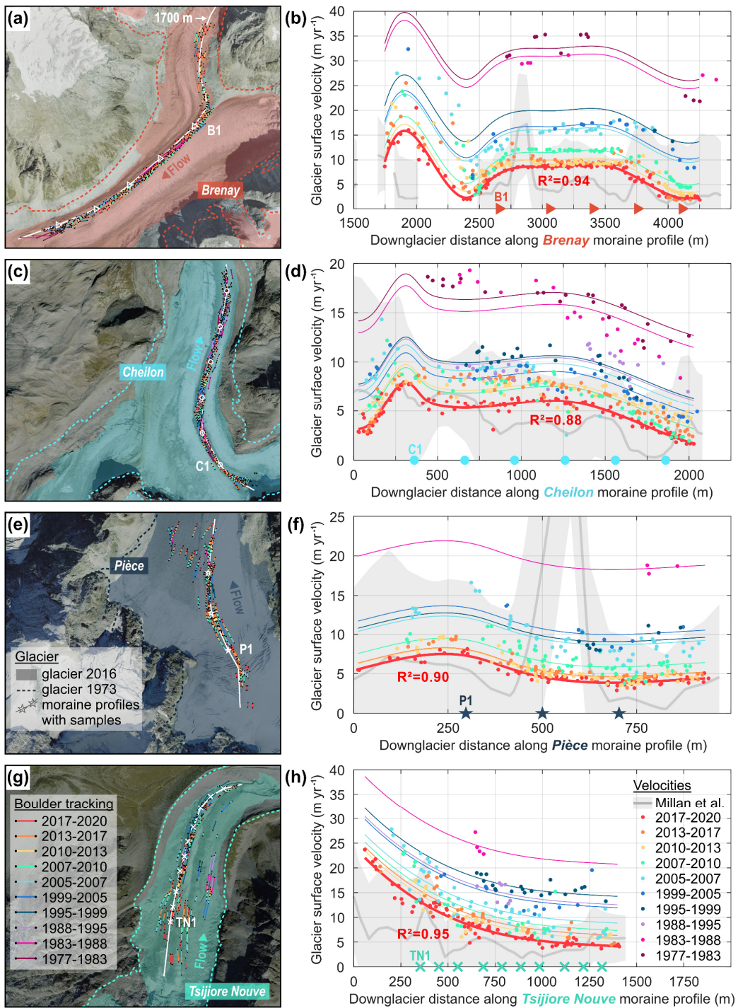
280 Figure 3: Glacier surface velocities along the four newly sampled medial moraines, reconstructed from 10 boulder tracking periods between the years 1977 to 2020. (a, c, e, g) Tracked boulder displacements along downglacier profiles, which trace the sampled medial moraines. Where a boulder could be followed across several tracking periods color-coded lines are connected. Note that boulder displacements at Brenay could only be tracked after a profile distance of ~1700 m, due to englacial transport along the first
