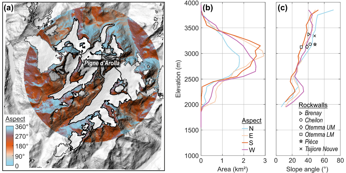
110 115 Figure 2: Morphology of ice-free rock faces and slopes in an area with 6 km radius, centred on the studied glaciers of the Pigne d'Arolla massif. (a) Topographic map indicating the aspect of ice-free areas. Areas covered by glacial ice (dashed black outlines) are excluded from the analysis and the five studied glacier sites (bold black outline) explicitly highlighted (2016 glacier outlines by Linsbauer et al., 2021). (b) Hypsometry and (c) slope angles of ice-free areas in 100 m elevation bins, differentiated by aspect. Symbols denote the mean elevation and mean slope angle of the studied source rockwalls.
