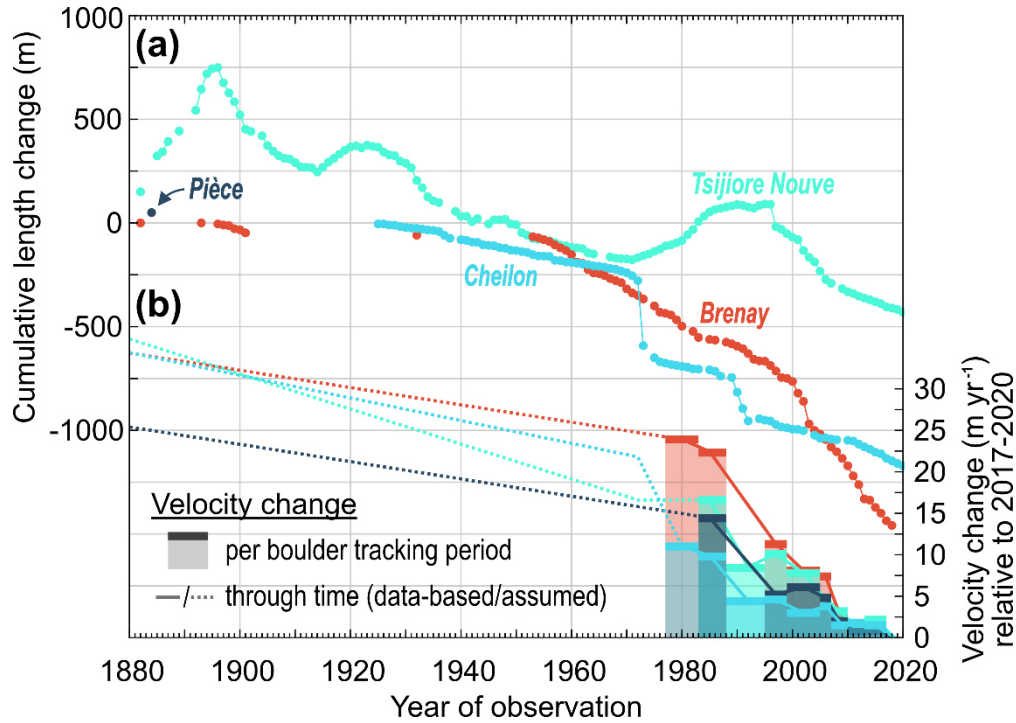
295 Figure 4: Glacier change at the four new study sites since 1880. (a) Long-term monitoring records of glacier length change (GLAMOS, 2021a). Note that markers from consecutive years are connected and that no length change record exists for Glacier de Pièce. (b) Reconstructed temporal changes in glacier surface velocity, relative to the most recent boulder tracking period 2017-2020. Per boulder tracking period, the velocity change corresponds to the y-axis shift of its fit line to the solid red fit line in Fig. 3b,d,f,h. On a year-to-year basis, velocity changes are based on linear interpolation between the velocity changes of the different tracking periods. Pre-1977 changes in velocities were approximated with reference to the linear gradient of the glacier's length change in (a). Due to lacking length data at Glacier de Pièce, pre-1977 assumptions there align with Glacier du Brenay. For reconstructions of Glacier d'Otemma see Wetterauer et al. (2022b). 300
