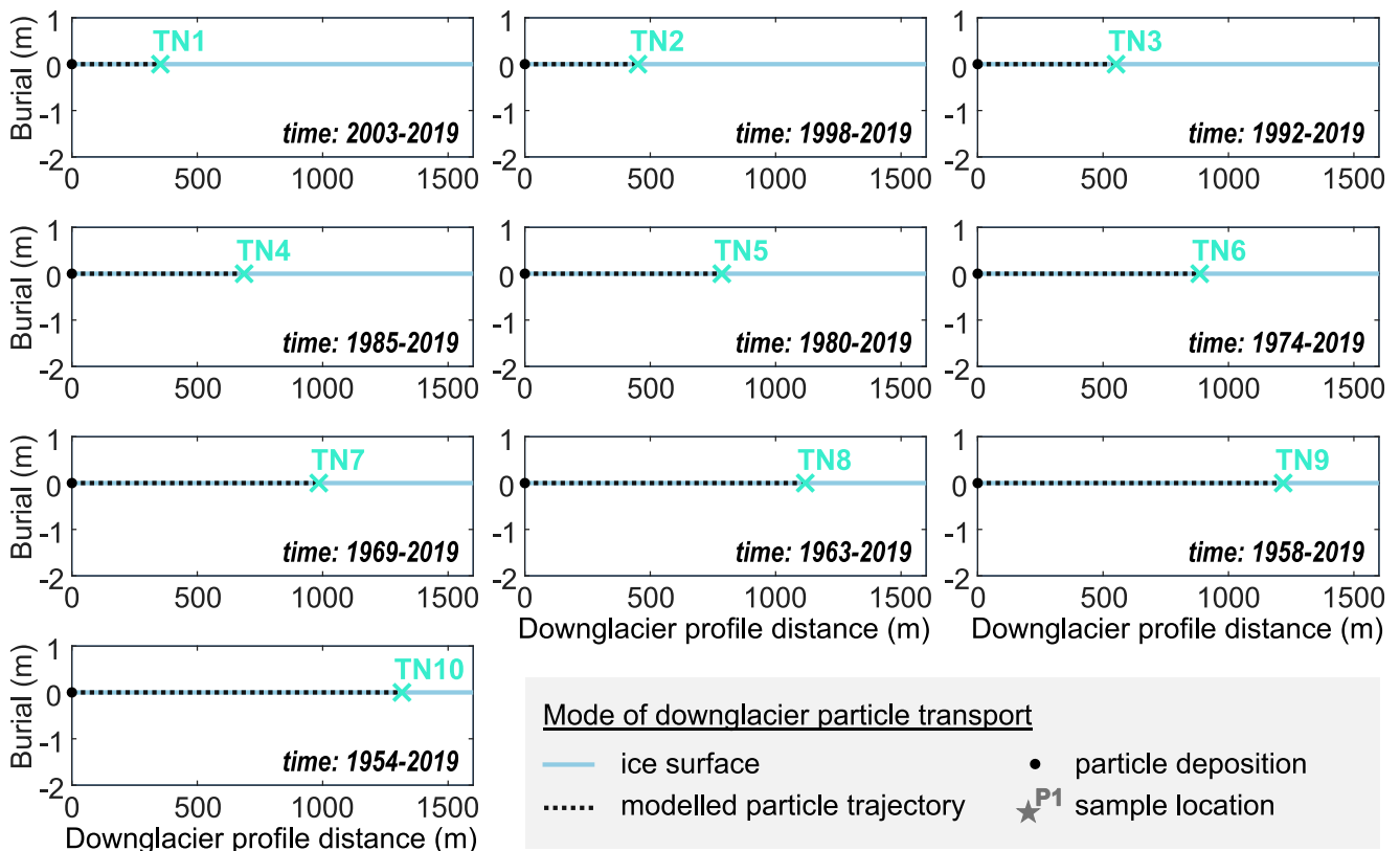
Figure S4: Modelled debris particle trajectories indicating the mode of downglacier particle transport from source rockwalls to sample locations at (a) Glacier de Cheilon, (b) Glacier de Pièce, and (c) Glacier de Tsijiore Nouvelle. Note that each graph stands for an individual sample. Shown is the burial depth of particles, which indicates whether a particle was transported within the ice (englacially; burial depth < 0 m) and shielded from cosmic radiation, or on the ice surface (supraglacially; burial depth = 0 m) and exposed to cosmic radiation. A particle's transport begins at the ice surface and profile head at the time as indicated and ends at the ice surface and downglacier distance of a sample's location in 2019.
