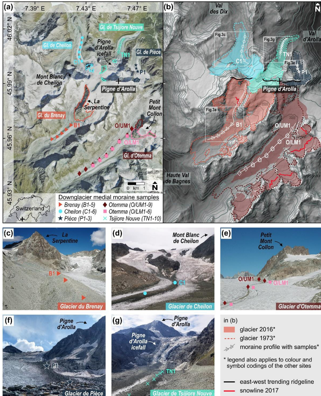
95 Figure 1: Pigne d’Arolla massif, Switzerland. (a) Orthoimage of the year 2017 showing the five adjacent glacier catchments, and their respective downglacier medial moraine sample locations, and their The respective associated source rockwalls are outlined (orthoimage from 2017 by swisstopo, 2022). (b) Hillshade image of the same area as in (a) with elevation as greyscale (bright = high). Coloured polygons/outlines show the glacier extents in 2016 and 1973 after Linsbauer et al. (2021) and Müller et al. (1976), respectively. The snowline of the 2017 orthoimage is indicated as approximation of the recent equilibrium line altitude. Hillshade
