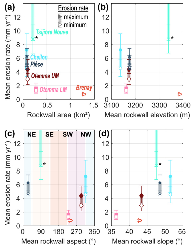
515 Figure 7: Comparison of apparent mean rockwall erosion rates with respect to (a) area, (b) mean elevation, (c) mean aspect, and (d) mean slope of the 1973-exposed source rockwalls. Apparent mean erosion rates ( \pm 1\sigma ) are depicted as shaded ranges from minimum (uncorrected) to maximum (transport-corrected) estimates. For comparison, mean erosion rates here include only samples associated with the recent deglaciation period (Fig. 5), but exclude samples from the Little Ice Age (O/UM6-9). The high concentration outlier at Glacier d'Otemma (O/UM4, Fig. 5) is also excluded, but would not change the overall pattern if included. 520 Note that mean erosion rates at Glacier de Tsijiore Nouve (*) should be treated with caution and are likely overestimated due to an unquantified subglacial bias (see Sect. 5.1), and that Glacier de Cheilon sample C5 was excluded from the maximum estimate due to its unreasonable high erosion rate (see Sect. 5.1).
