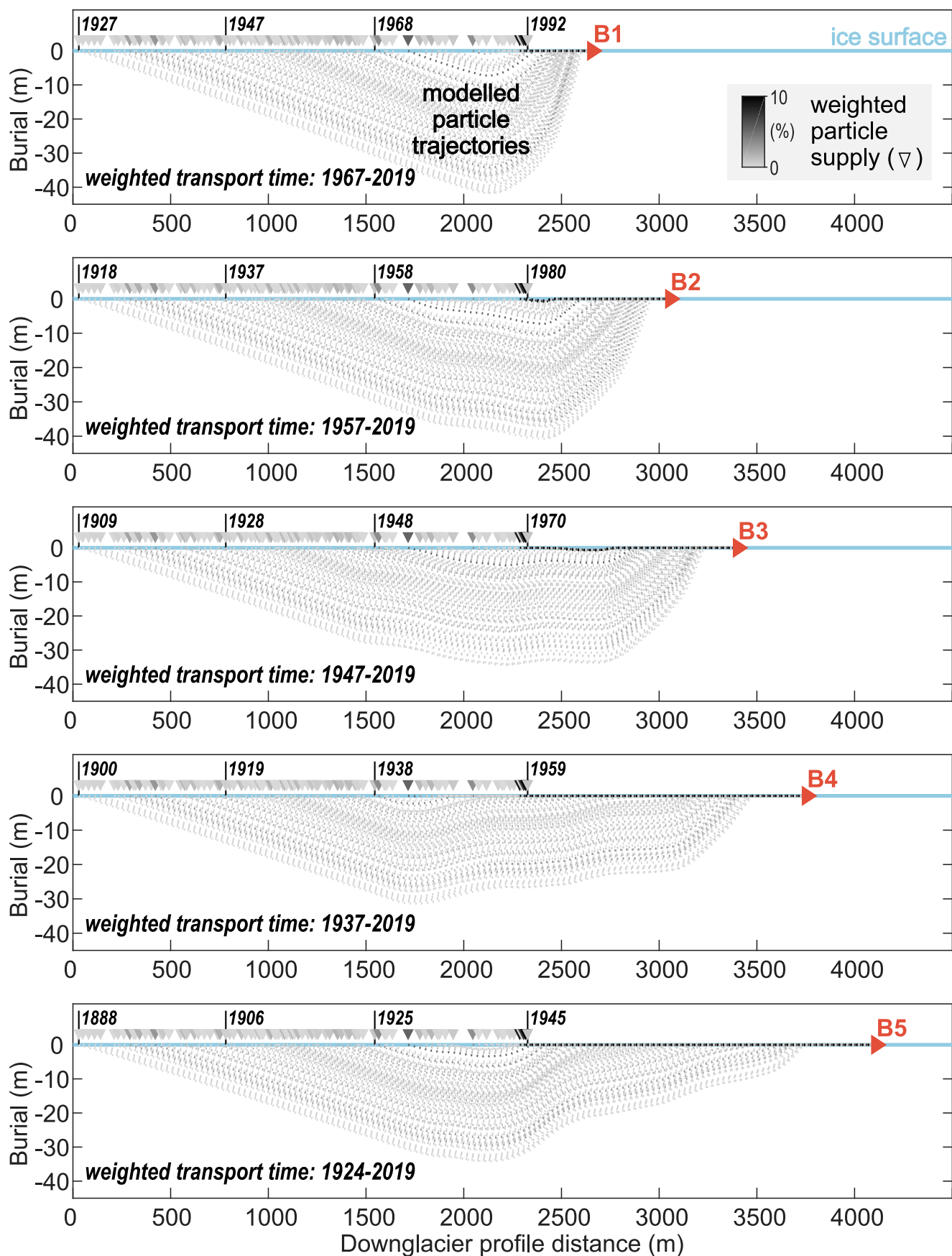
Figure S3: Modelled debris particle trajectories indicating the mode of downglacier particle transport from source rockwalls to sample locations B1-B5 at Glacier du Brenay. Shown are all trajectories of particles deposited along the first ~2.3 km of the downglacier profile that arrive at the ice surface and downglacier distance of a sample's location in 2019. For reference, start years of four trajectories are given. The burial depth indicates whether a particle was transported within the ice (englacially; burial depth < 0 m) and shielded from cosmic radiation, or on the ice surface (supraglacially; burial depth = 0 m) and exposed to cosmic radiation. Graded colours indicate the percentage debris particle supply along the first ~2.3 km profile distance (see also Fig. S2b) and the weight of its corresponding trajectory, used to estimate a weighted time of downglacier particle transport.
